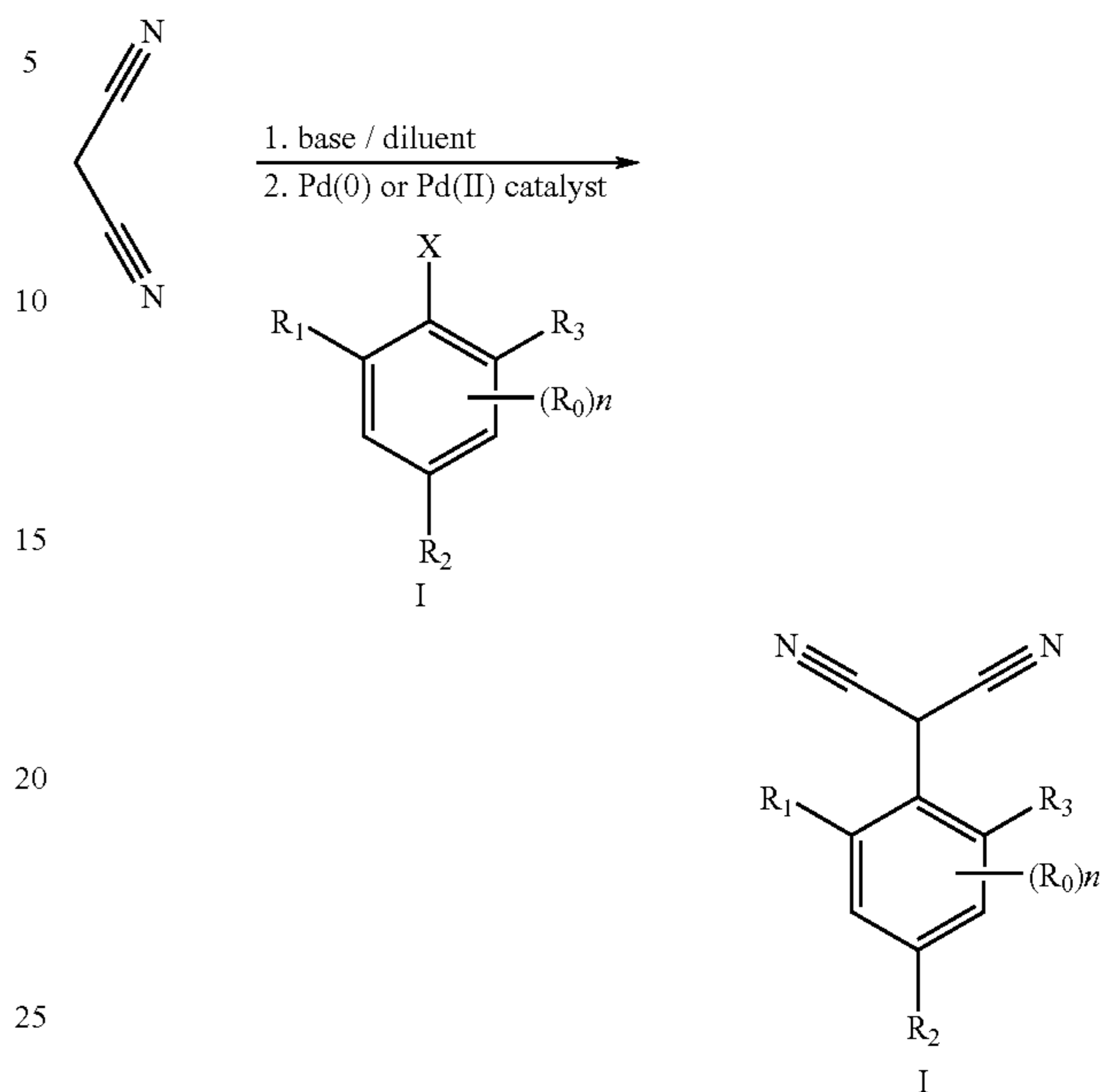
Reaction scheme 1
