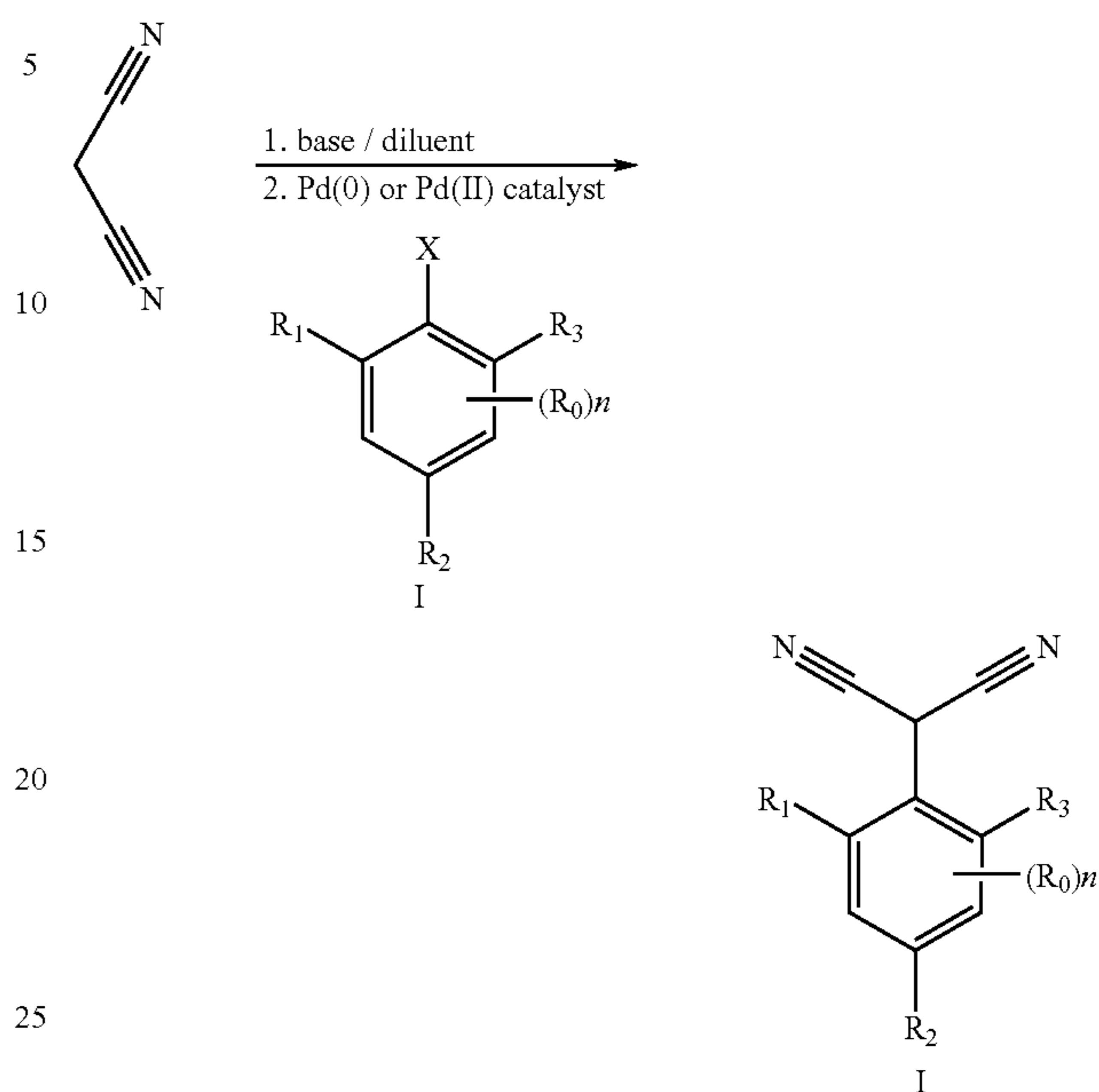
Reaction scheme 1
