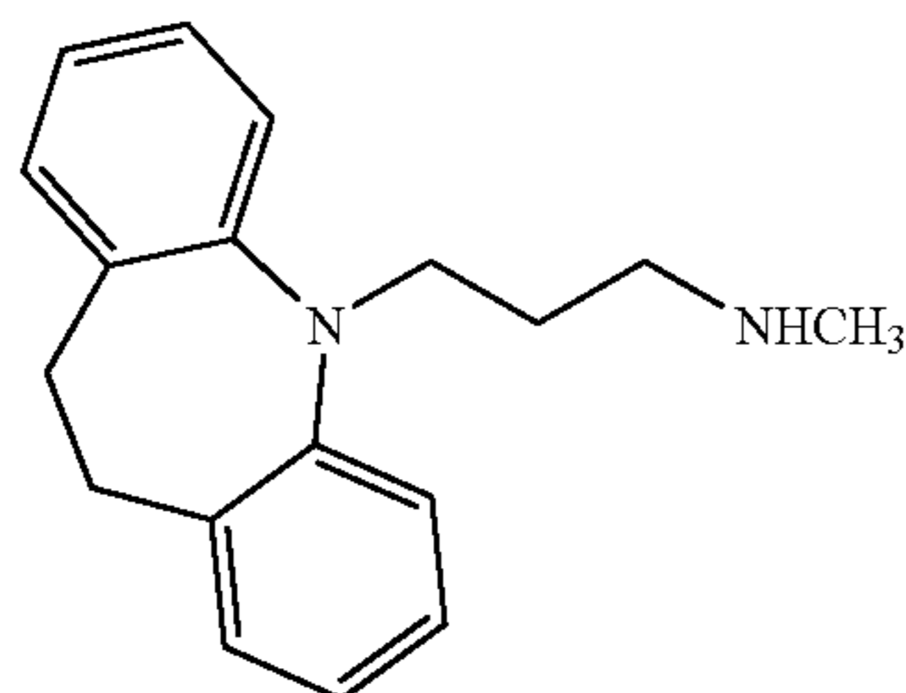
Desipramine
