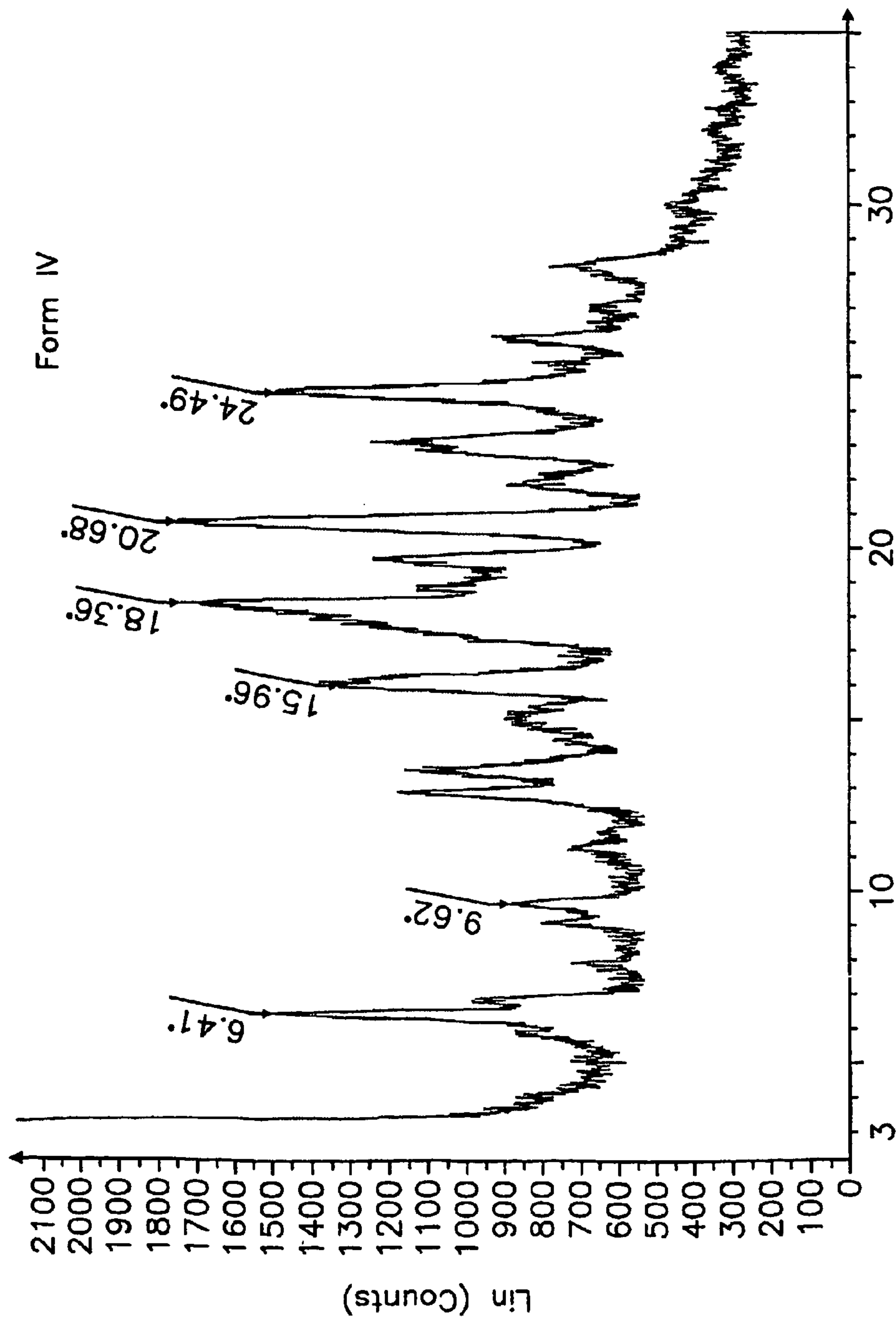
2-Theta-Scale
