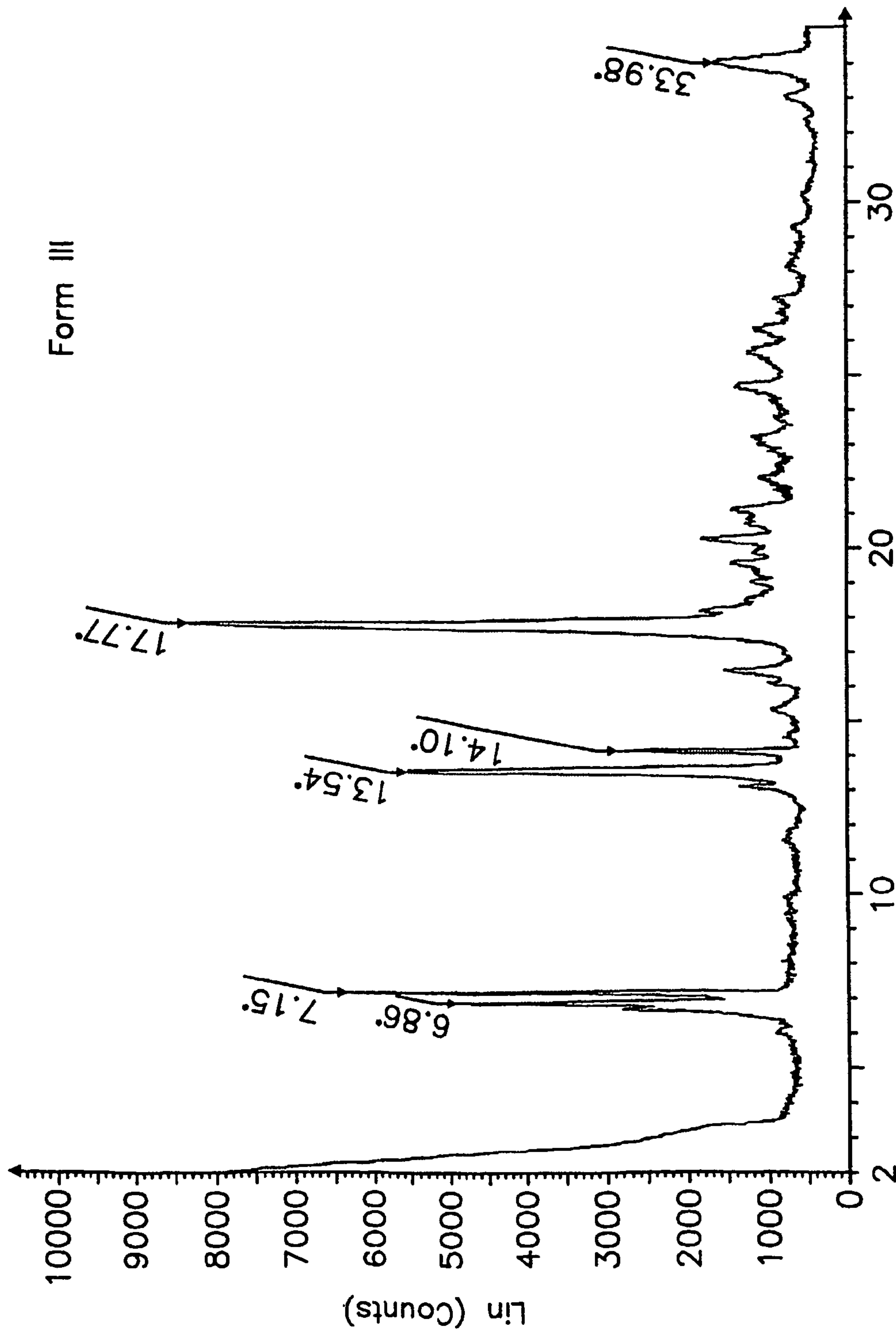
2-Theta-Scale
