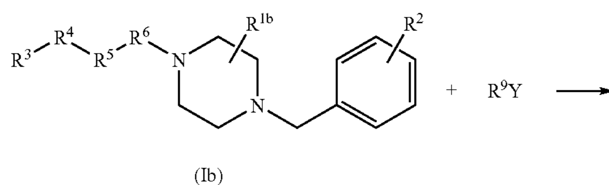
Reaction Scheme 8
