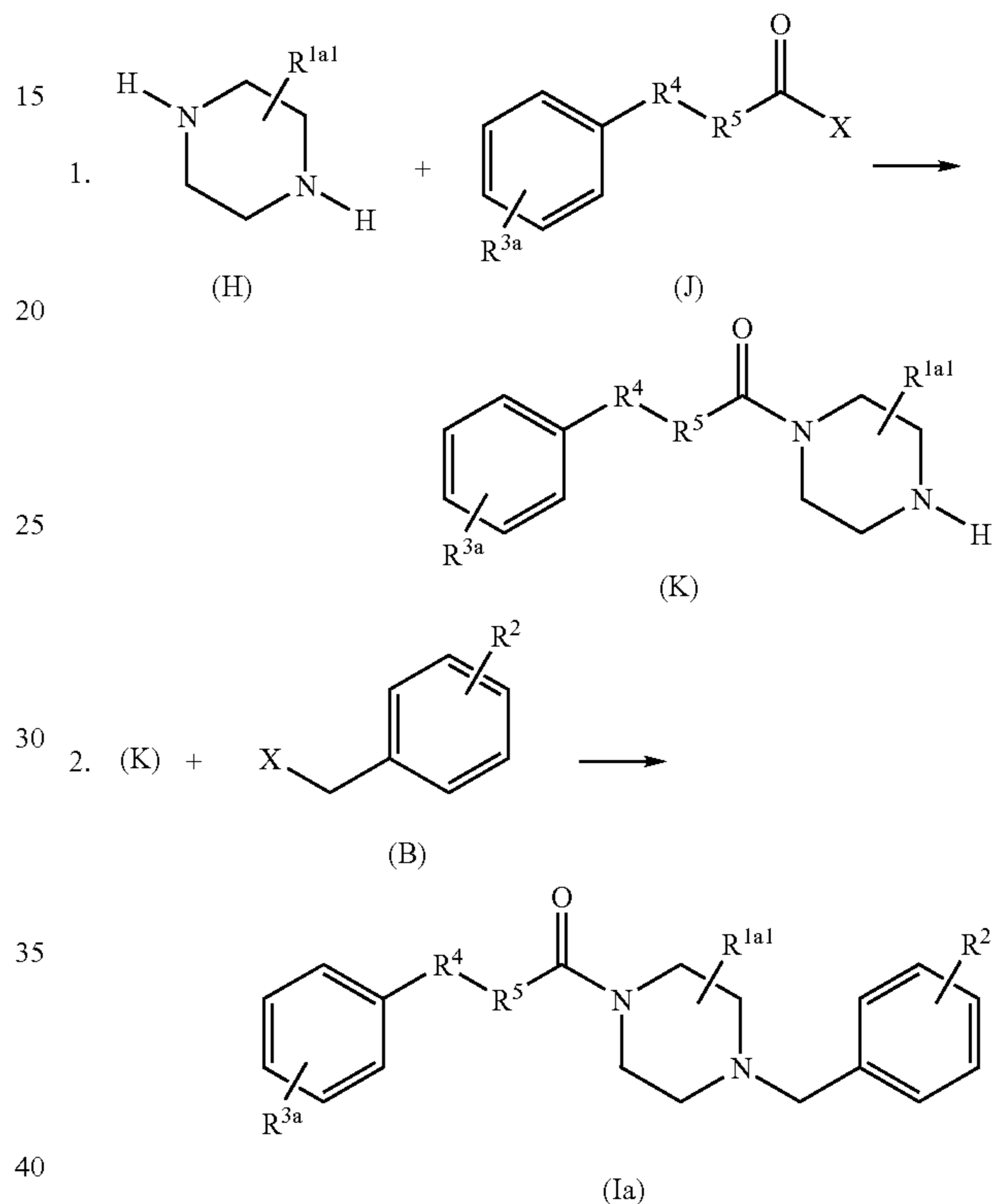
Reaction Scheme 3
