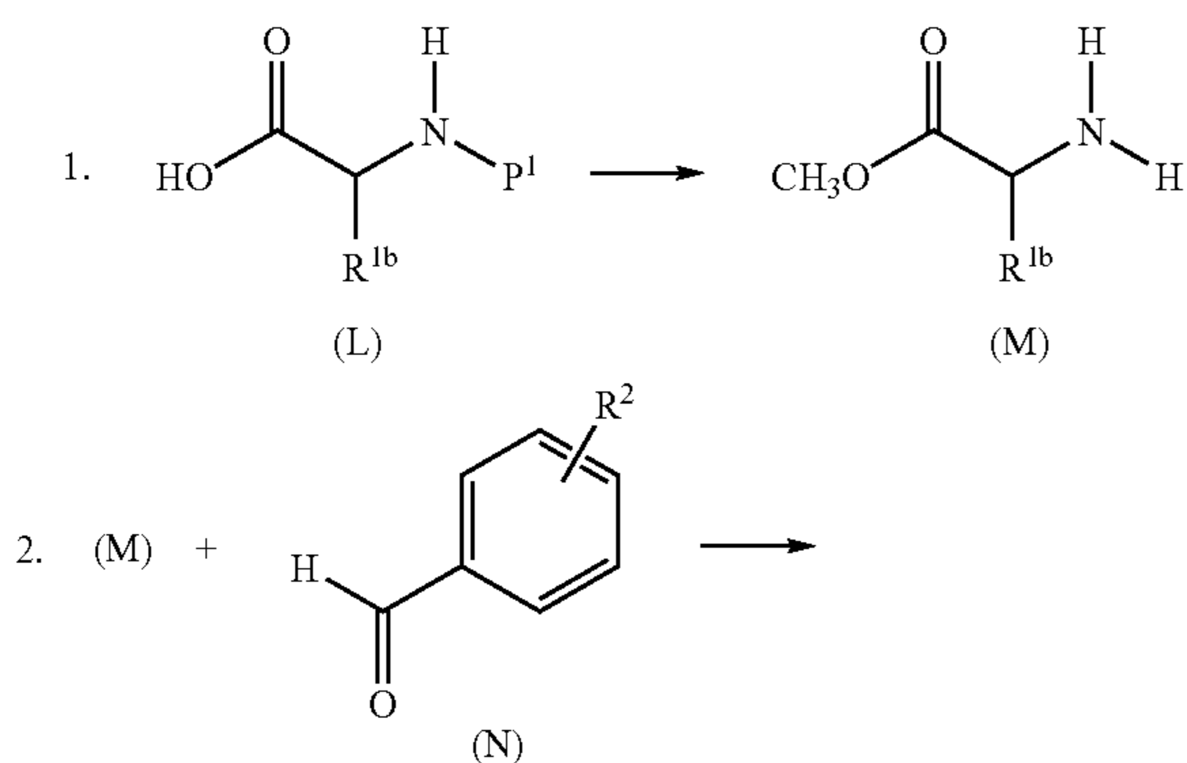
Reaction Scheme 4
