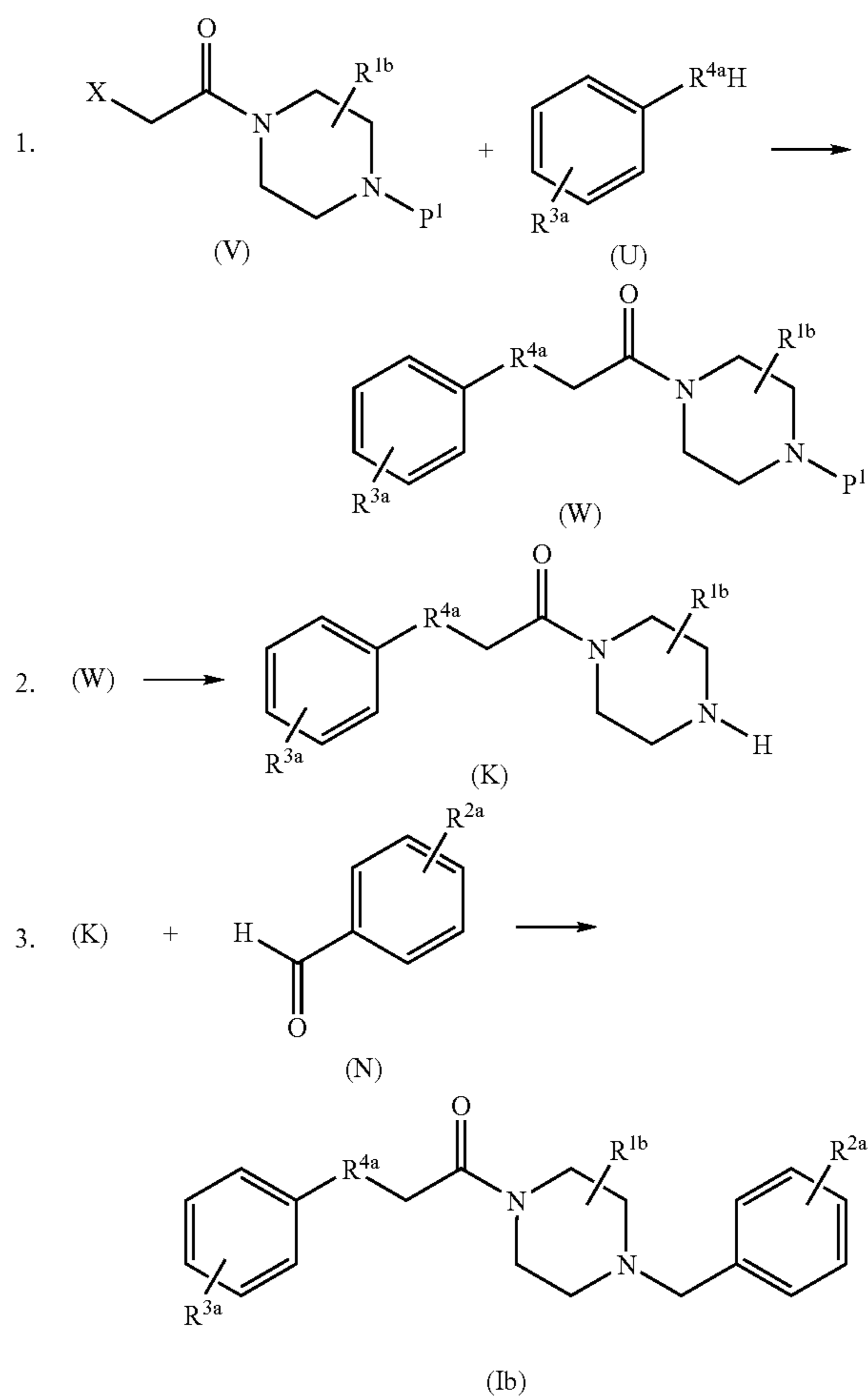
Reaction Scheme 6
