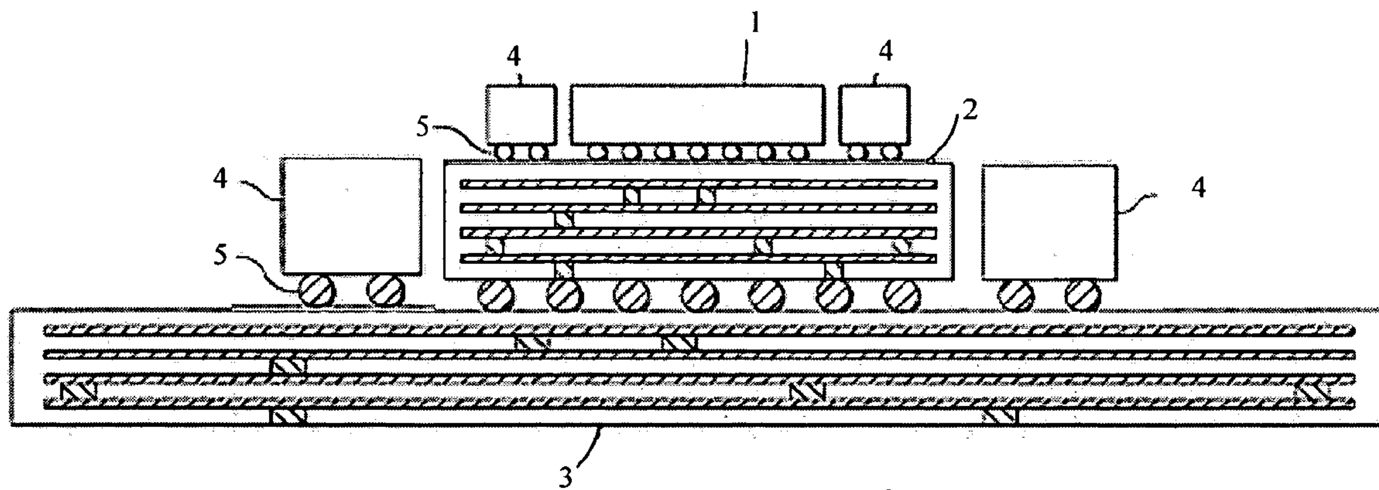
Fig. 1 Prior Art
