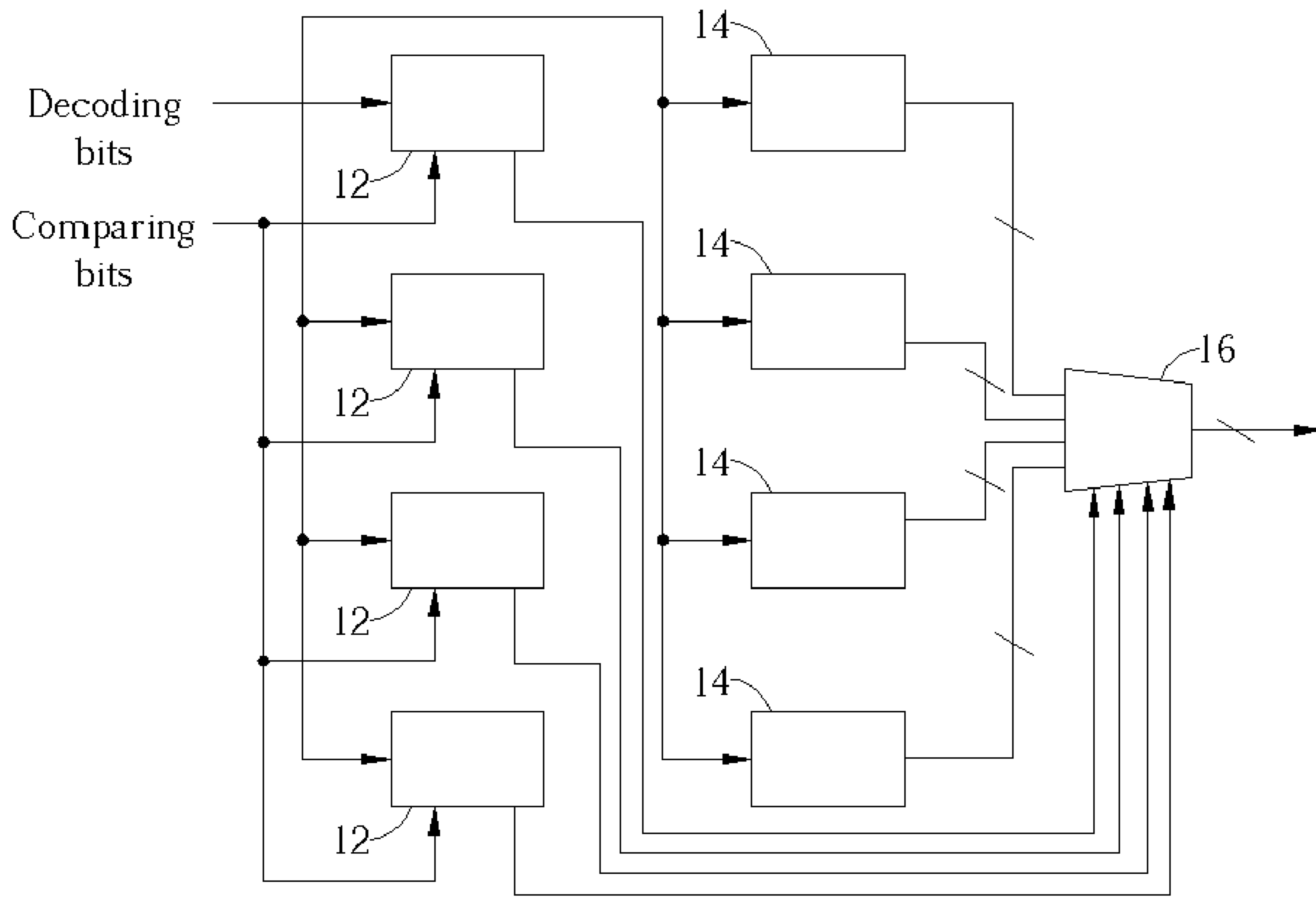
Fig. 2 Prior art
