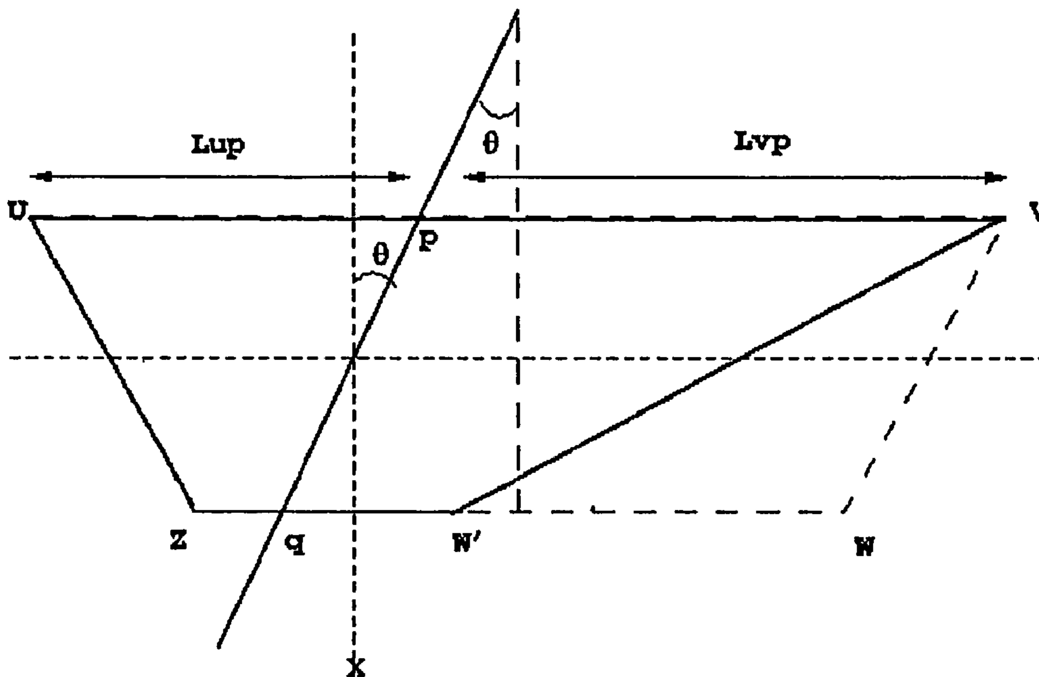
GENERATION OF THE GRID (U, V, W', Z) ASSOCIATED TO (x \theta )
