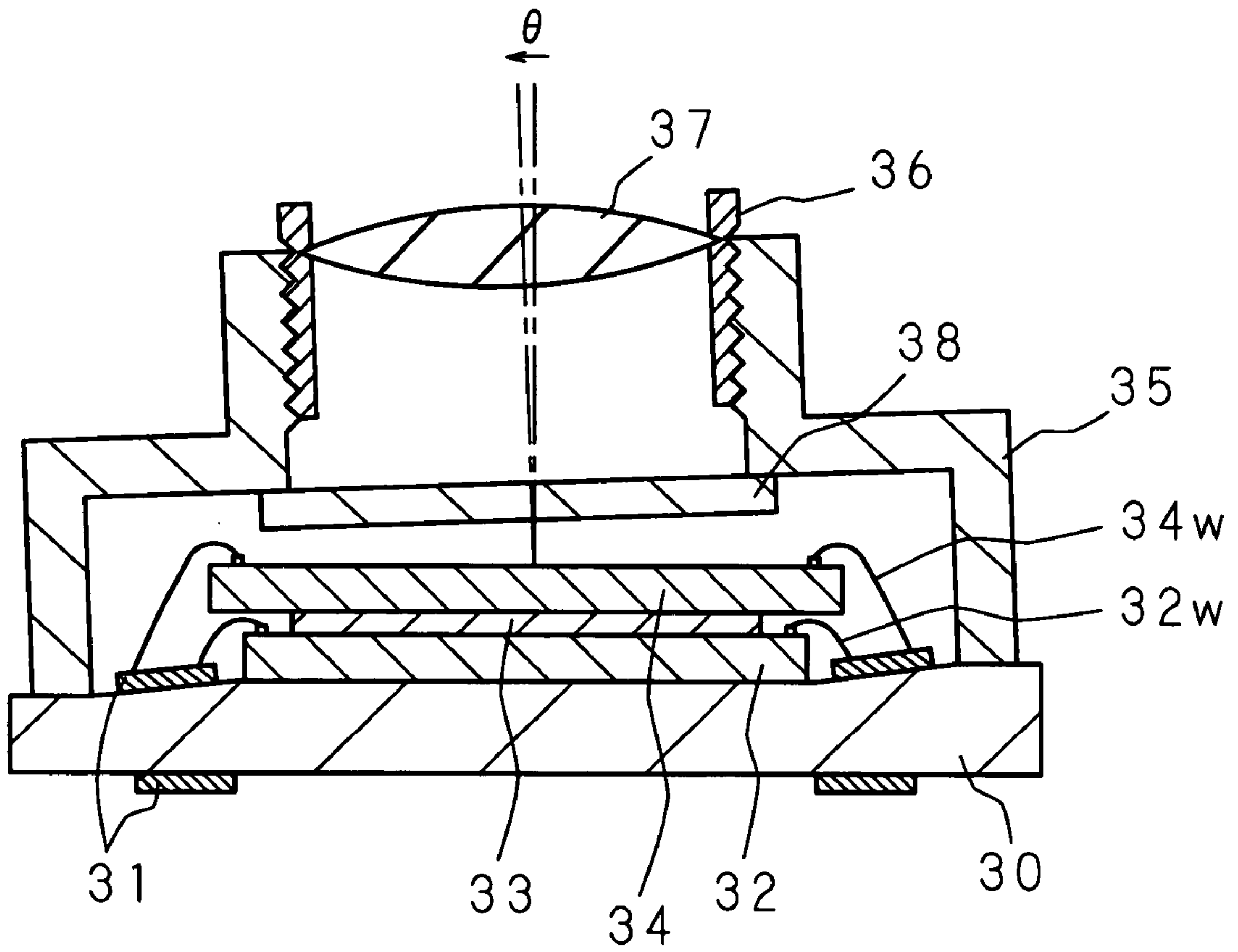
FIG. 4 PRIOR ART
