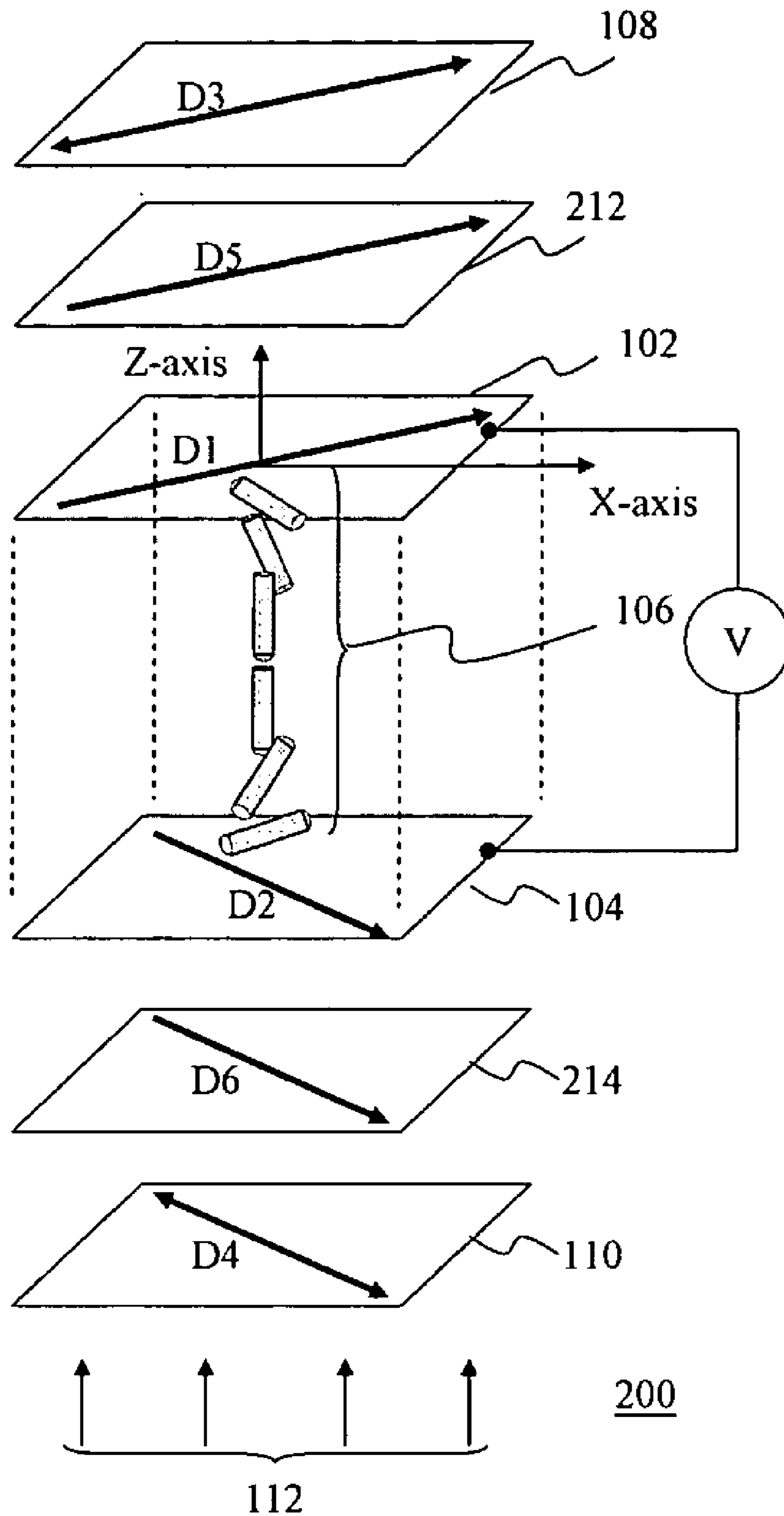
FIG. 2 (PRIOR ART)
