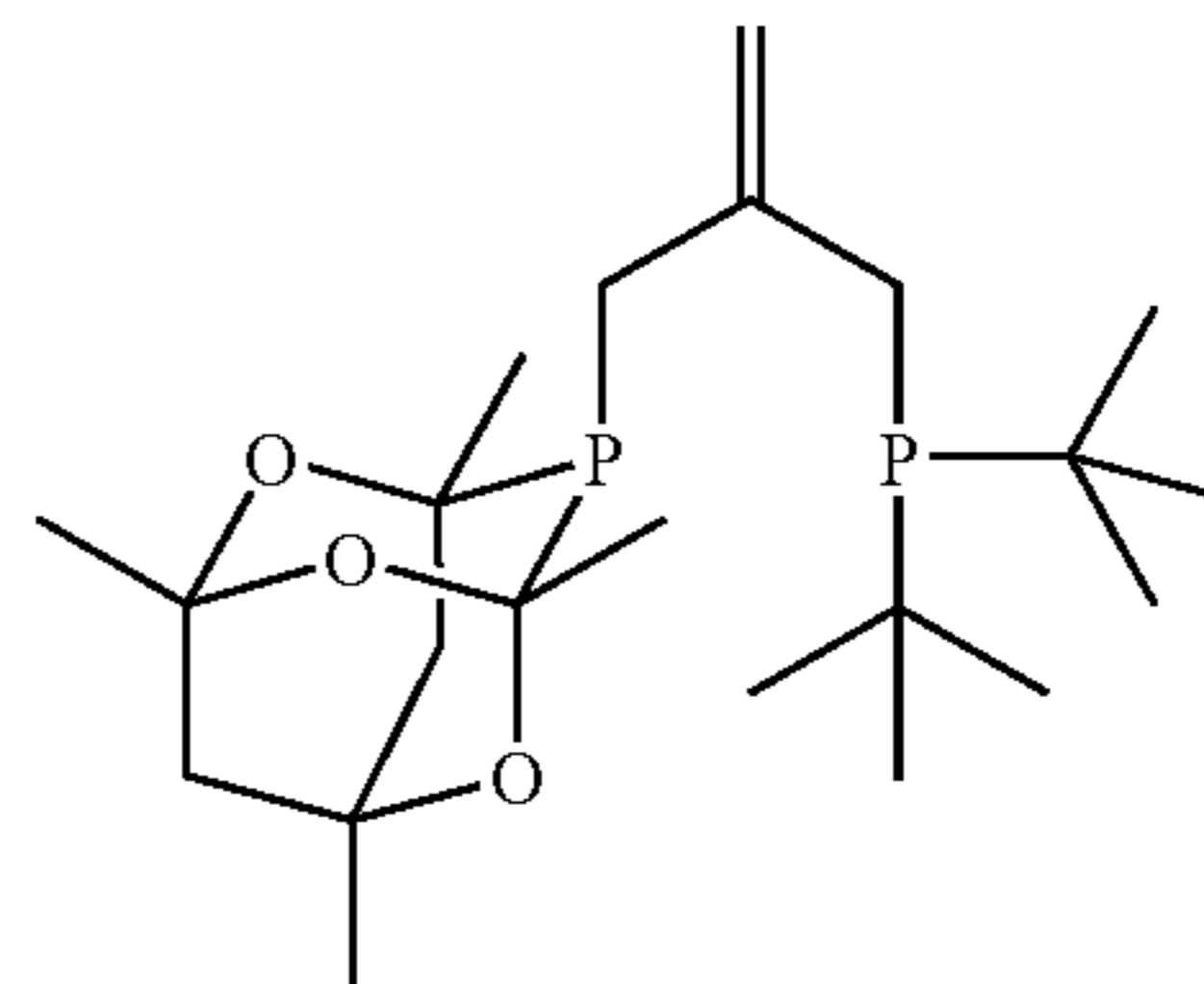
FIG. 2: 8-(2-[[di(tert-butyl)phosphino]methyl]-2-propenyl)-1,3,5,7-tetramethyl-2,4,6-trioxa-8-phosphatricyclo[3.3.1.1.{3,7}]decane
