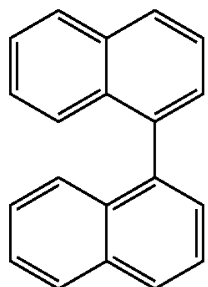
1,1'-binaphthyl
