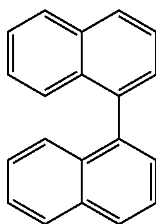
1,1'-binaphthyl
