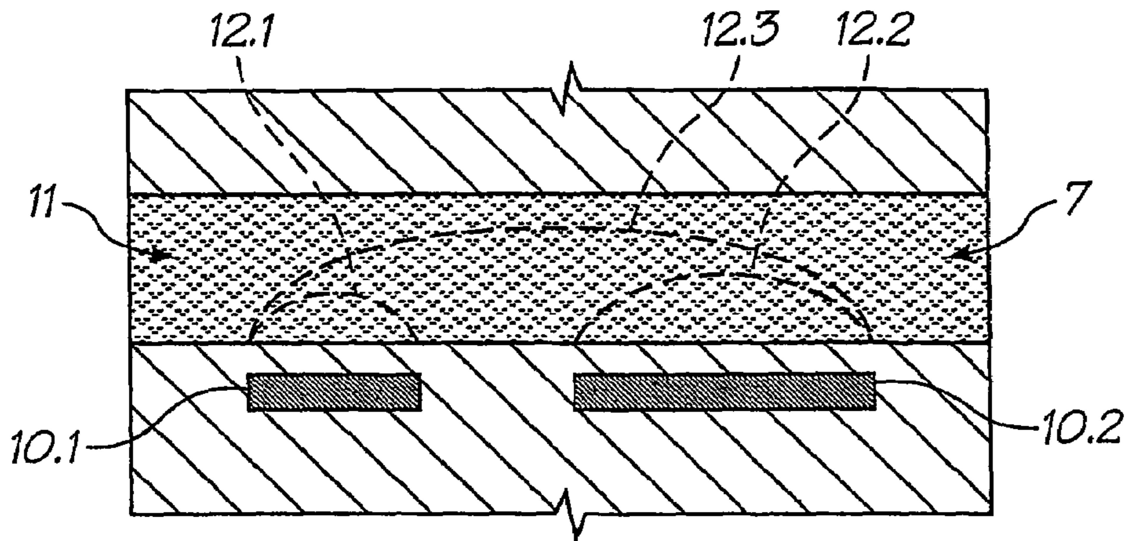
FIG. 52 (PRIOR ART)
