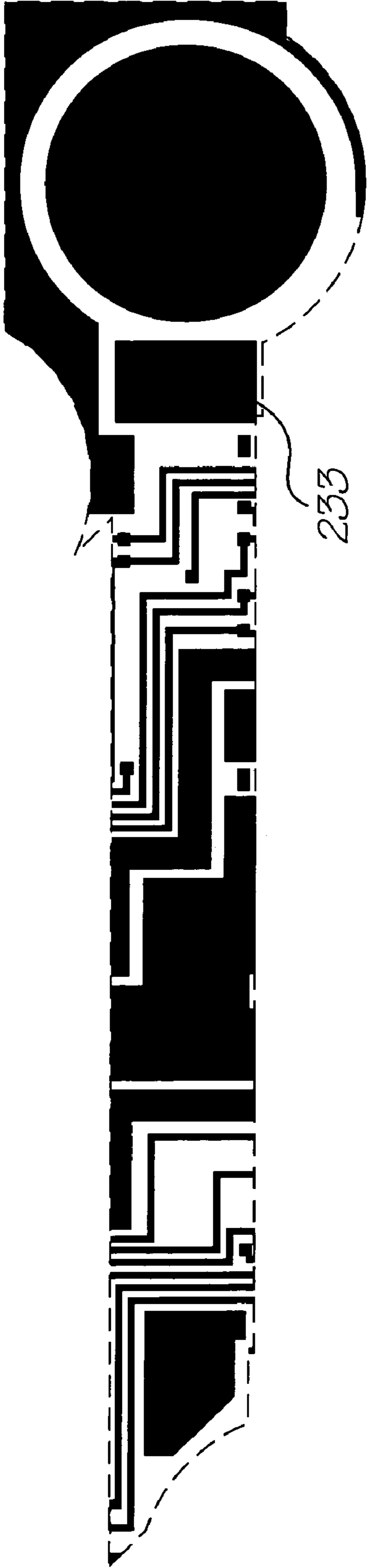
Metal 2 mask
