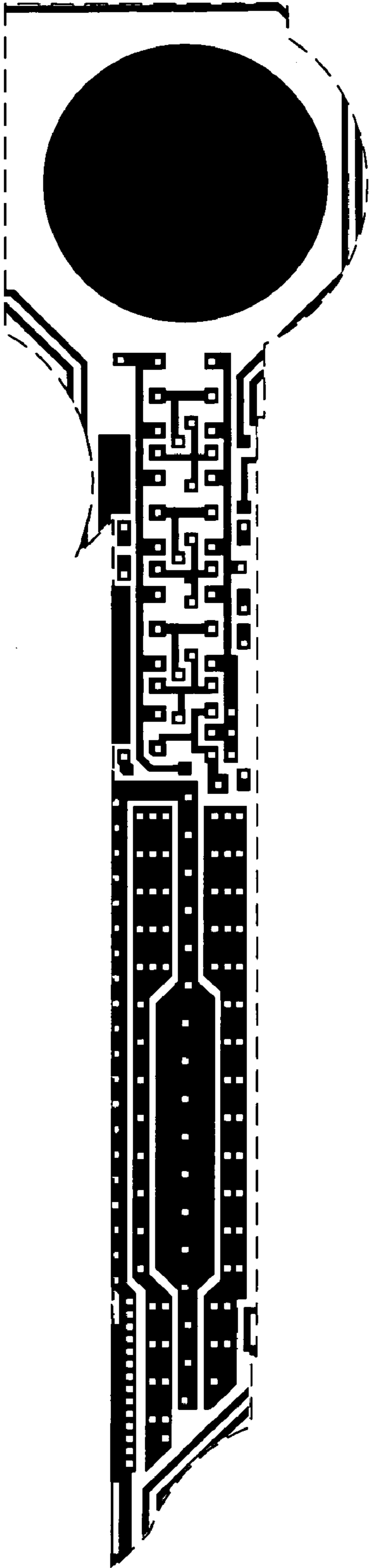
Metal 1 mask
