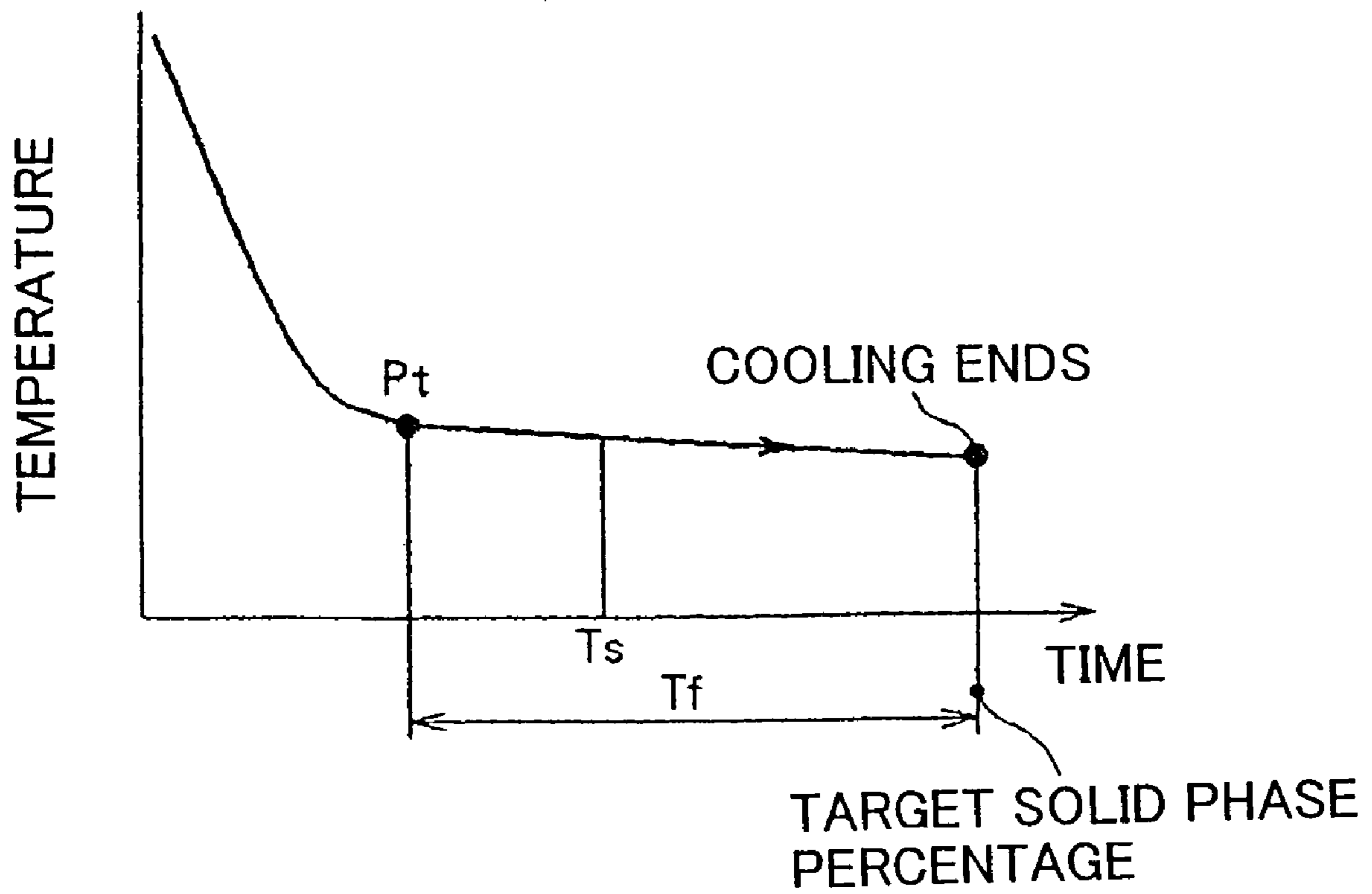
FIG. 36 (Prior Art)
