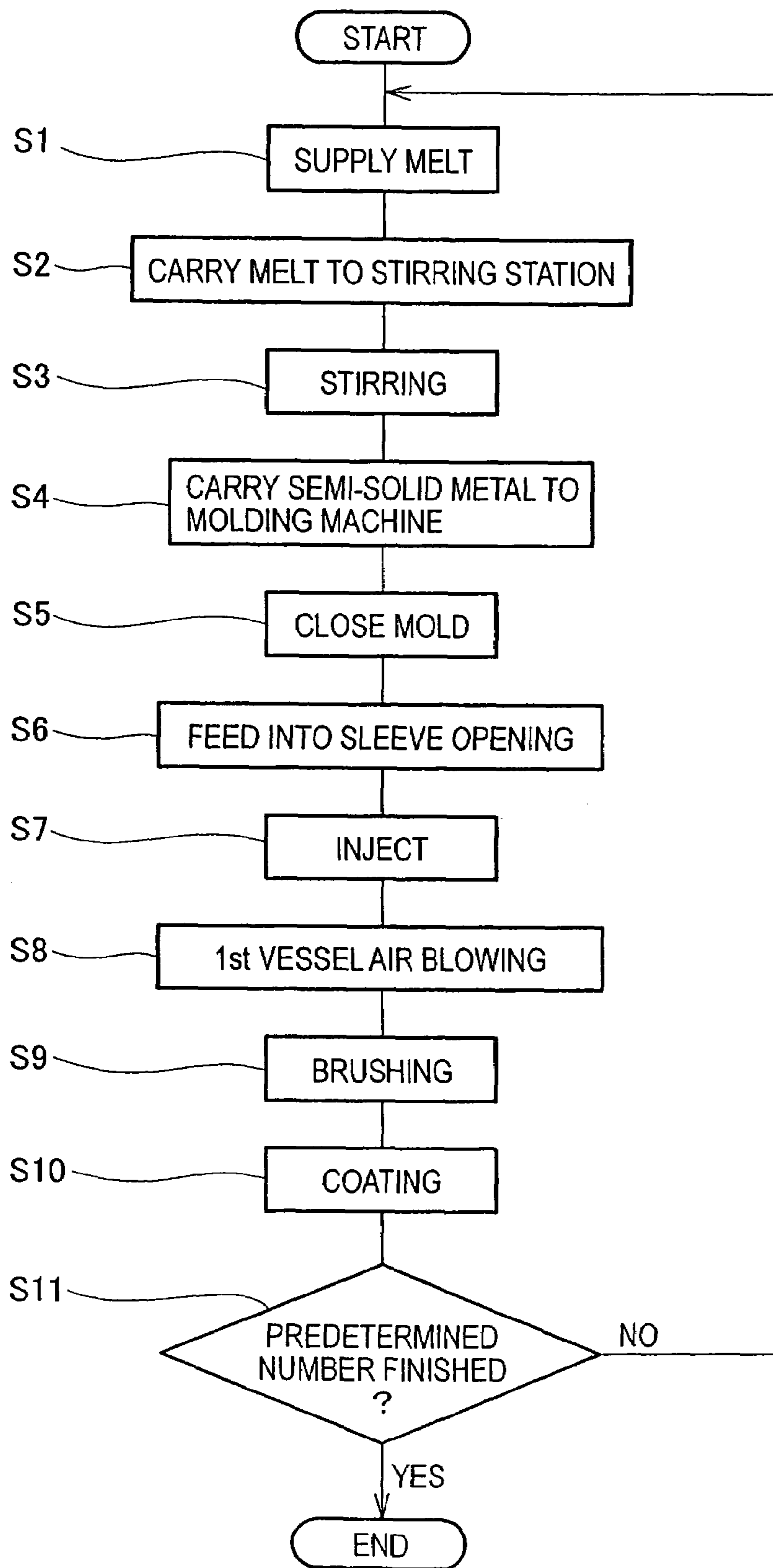
FIG. 37 (Prior Art)
