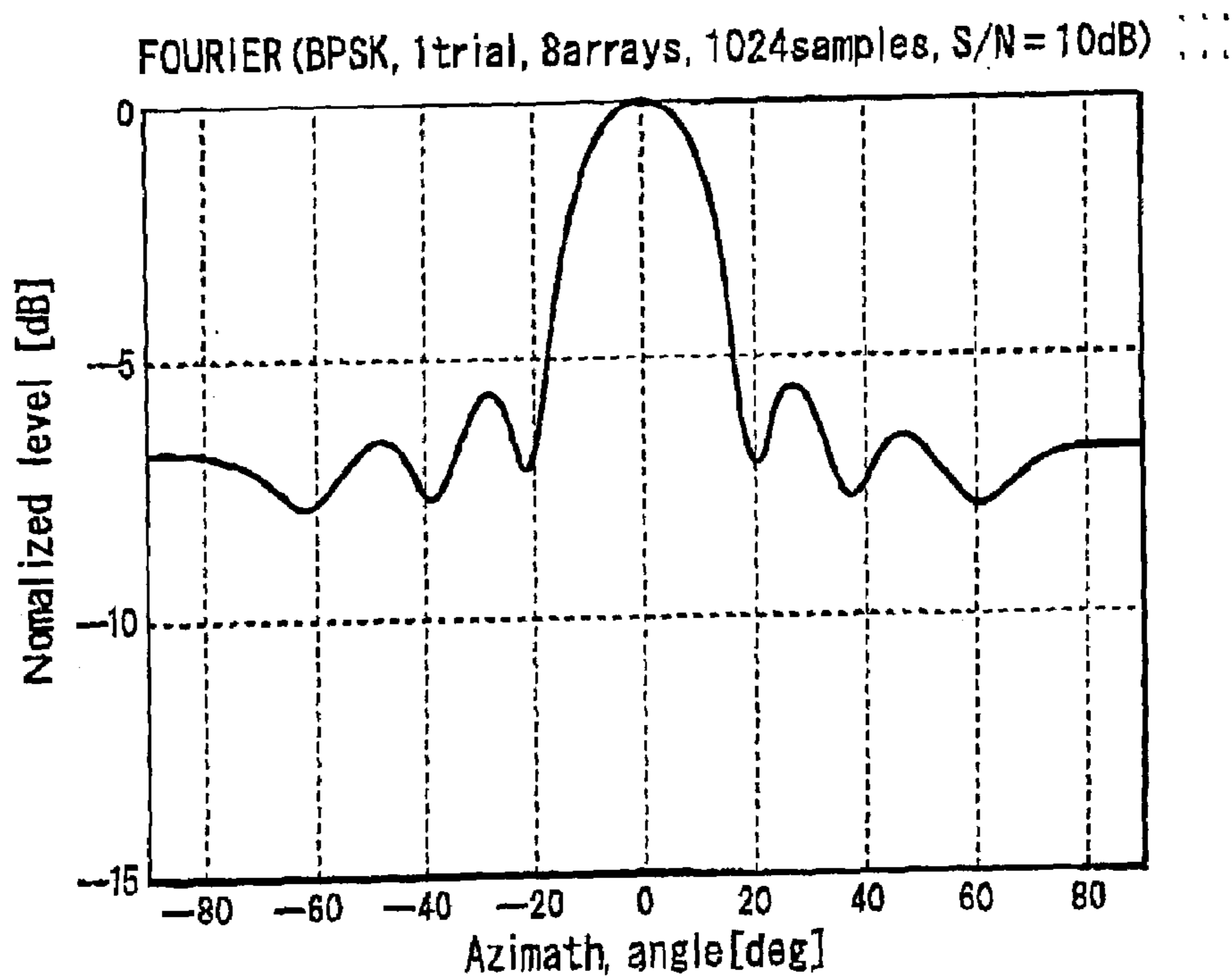
(b) DIRECTION ESTIMATION RESULT FOR PATH, 1=5° , PATH, 2=-5°
