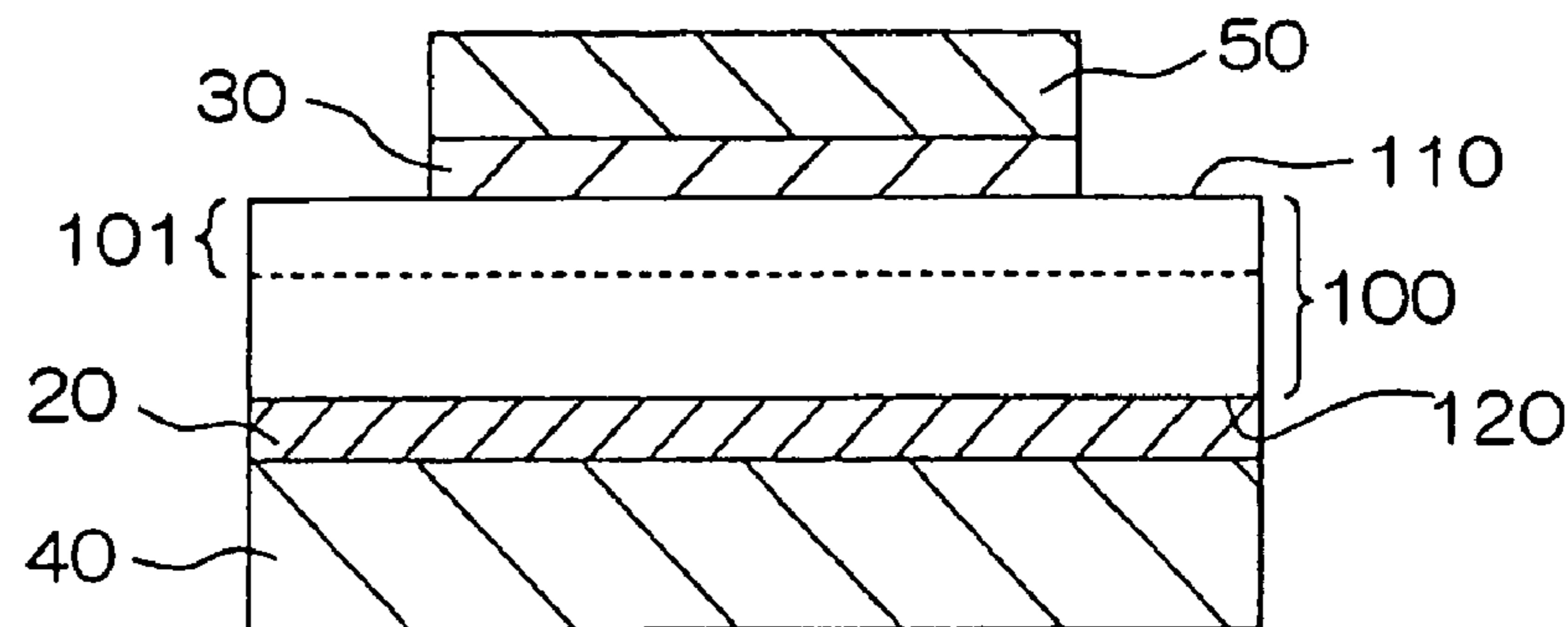
FIG. 9(e) PRIOR ART
