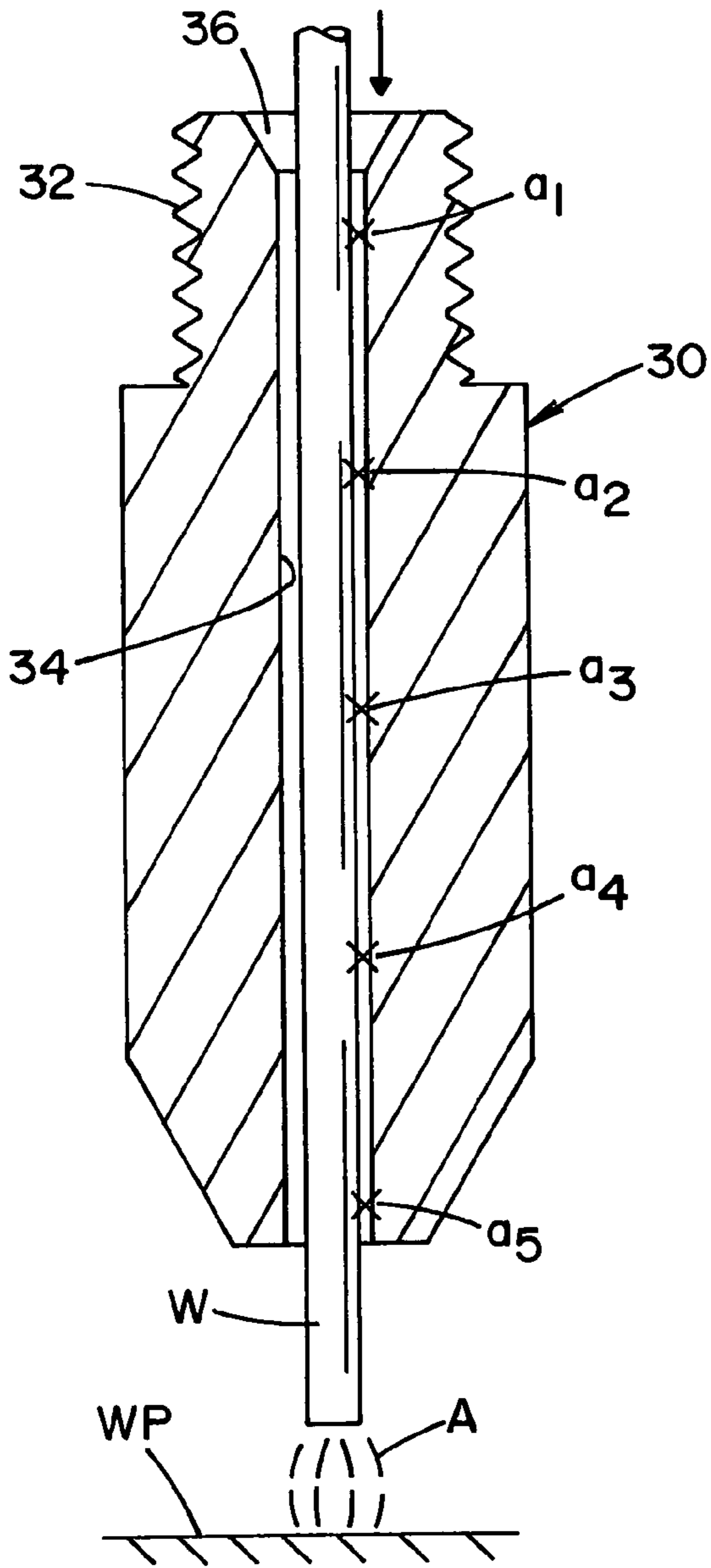
FIG. 5 (PRIOR ART)
