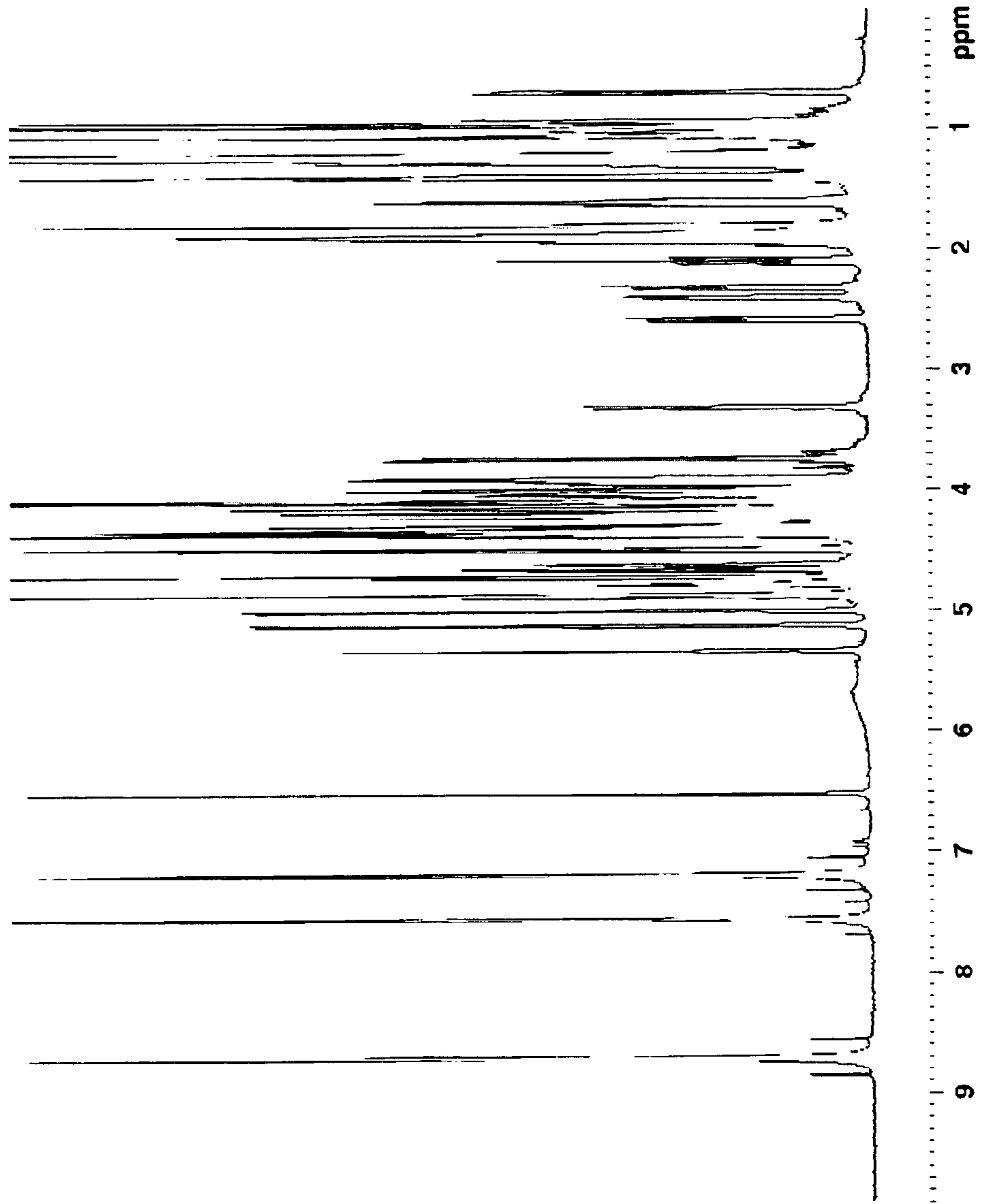
Figure 54 O54-H-NMR
