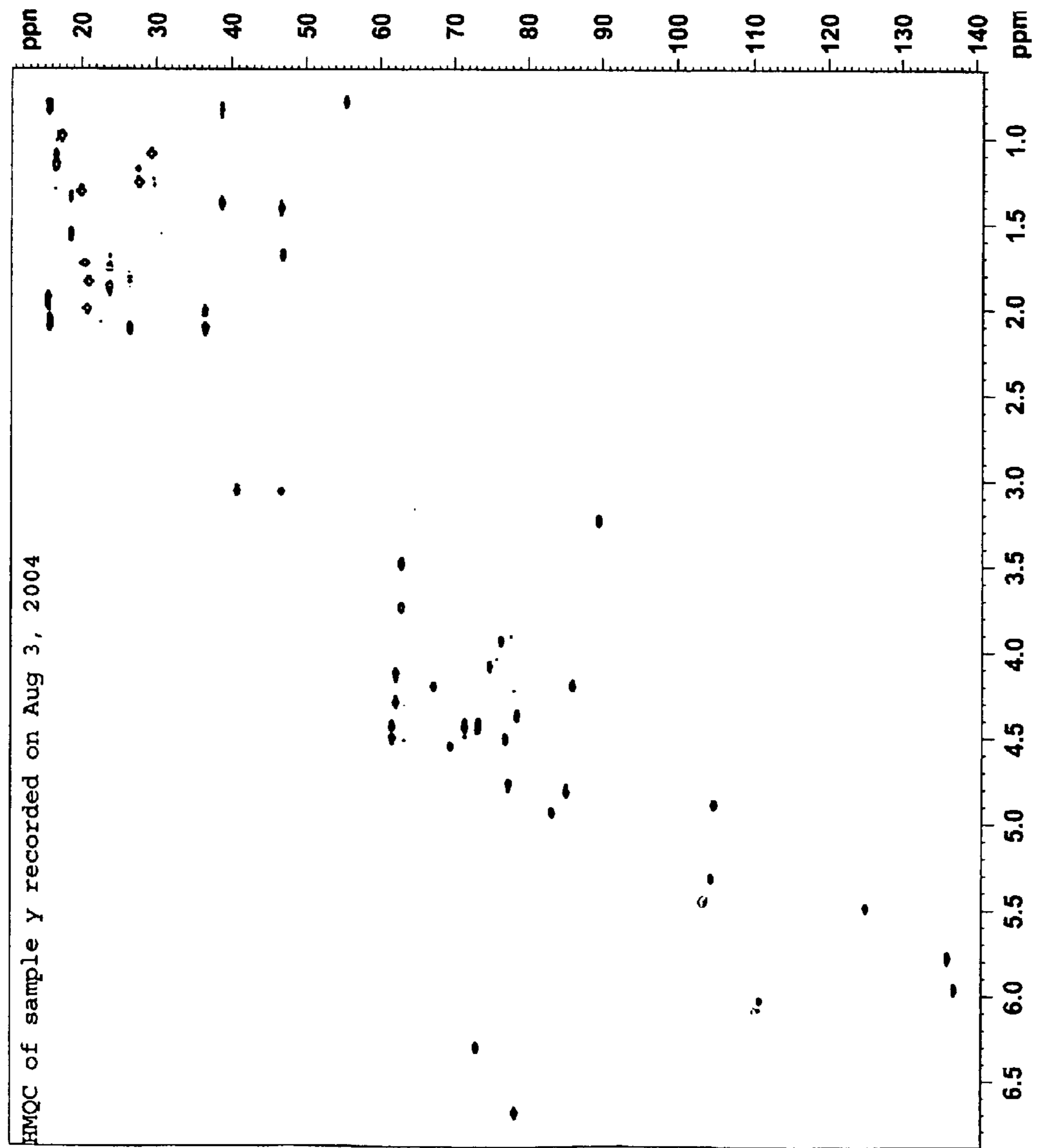
Figure 19 2D NMR (HMQC) of Y
