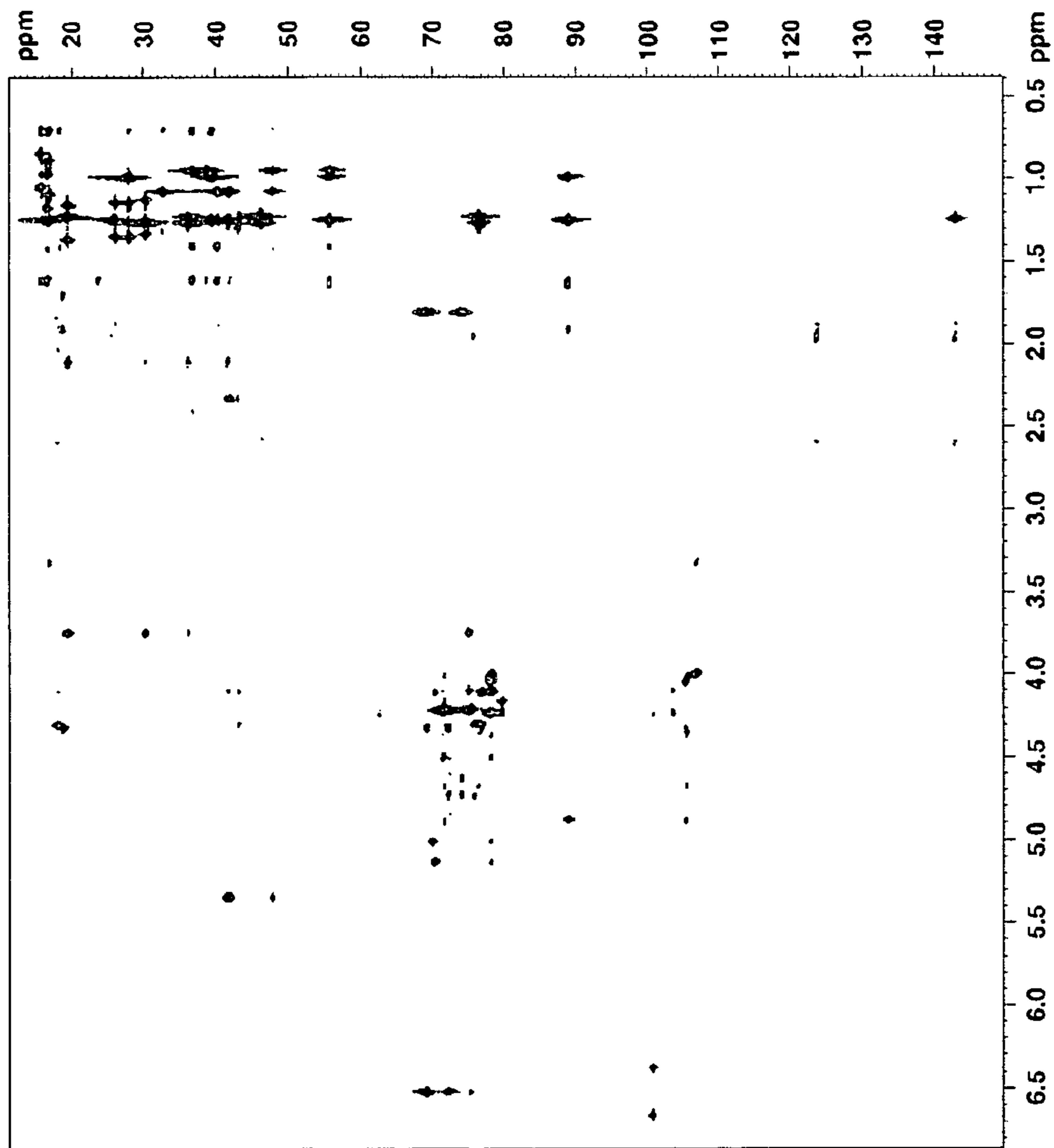
Figure 56 O54-HMBC
