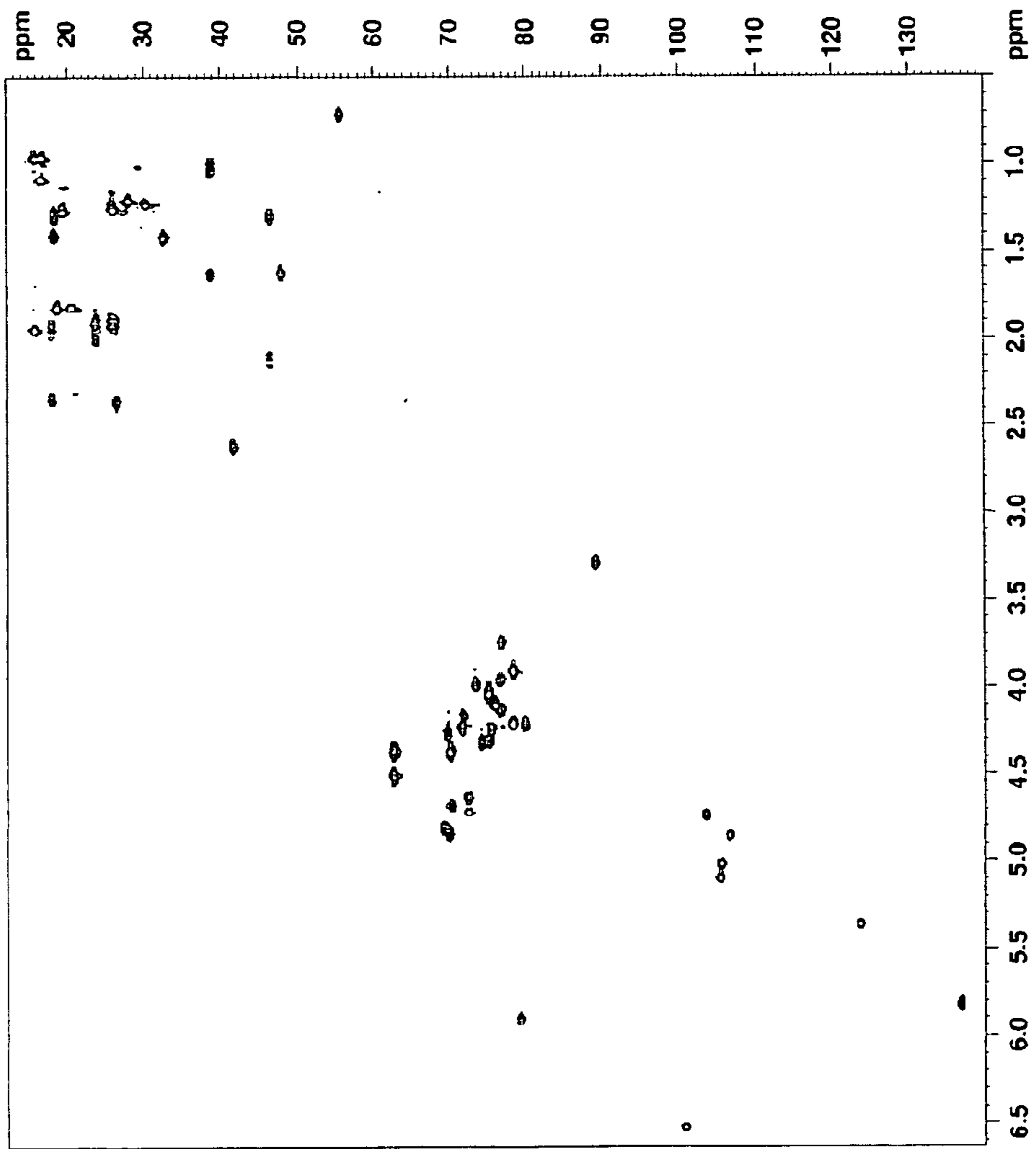
Figure 49 R1-HMQC
