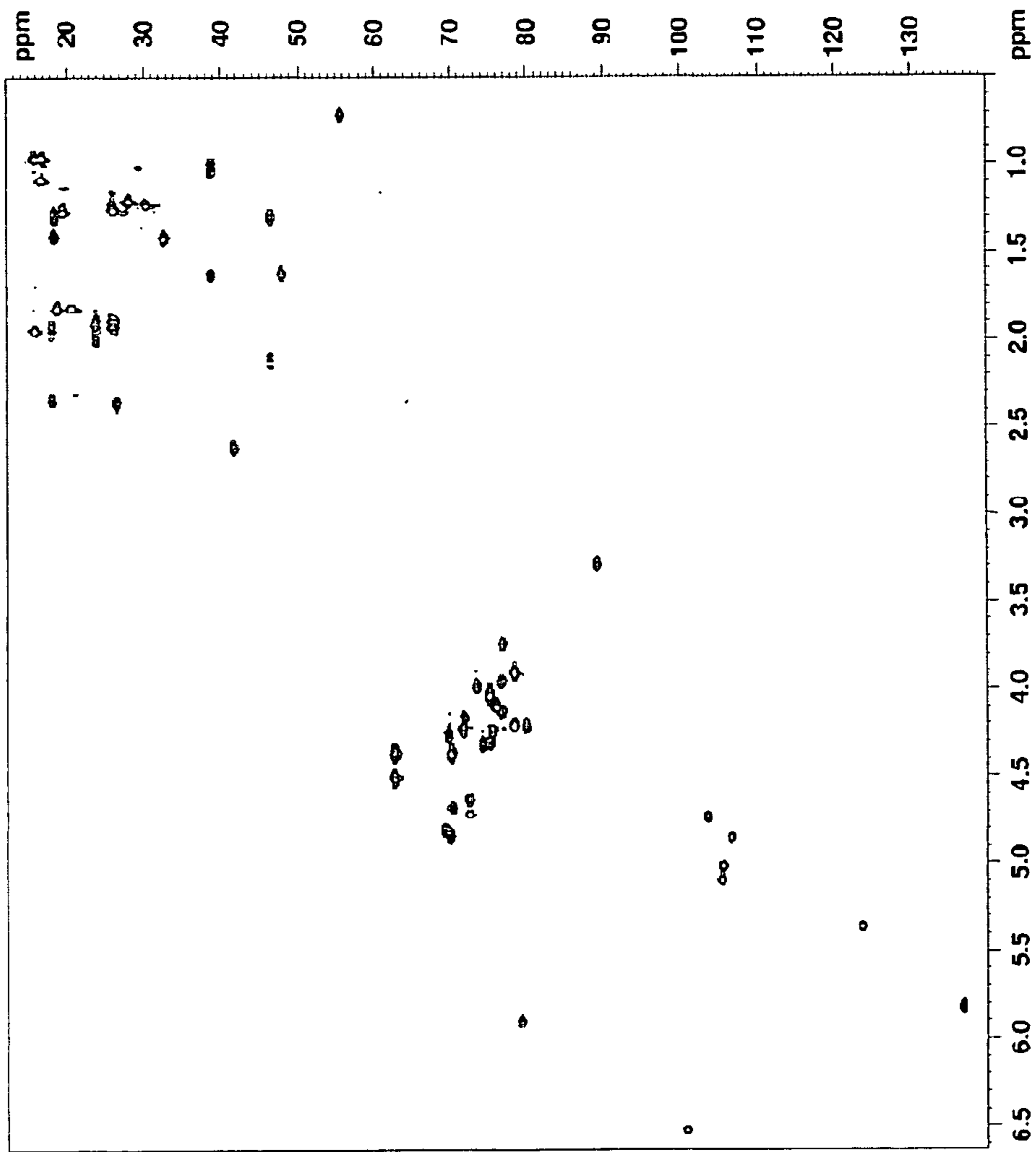
Figure 49 R1-HMQC
