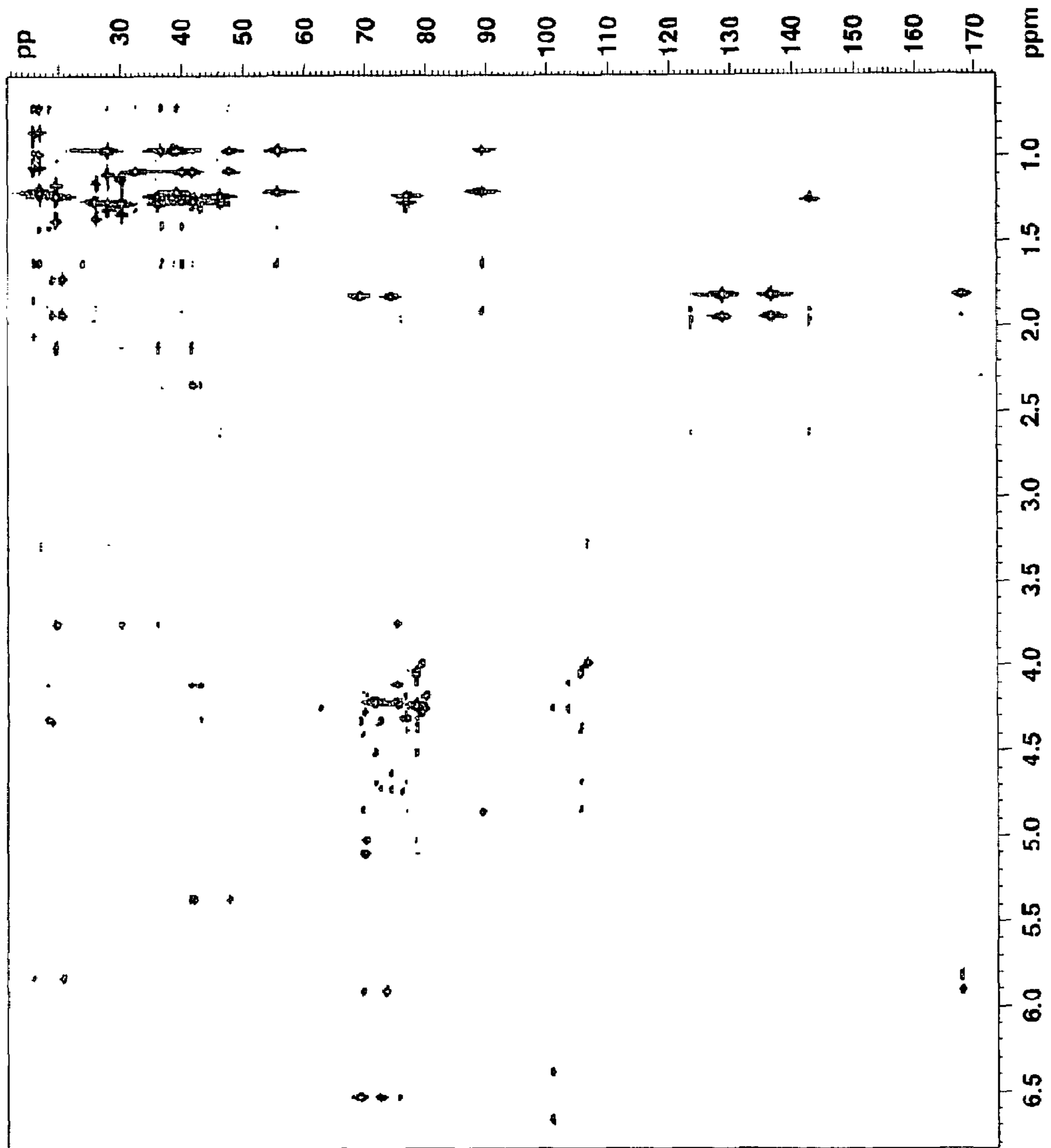
Figure 50 R1-HMBC-level 1
