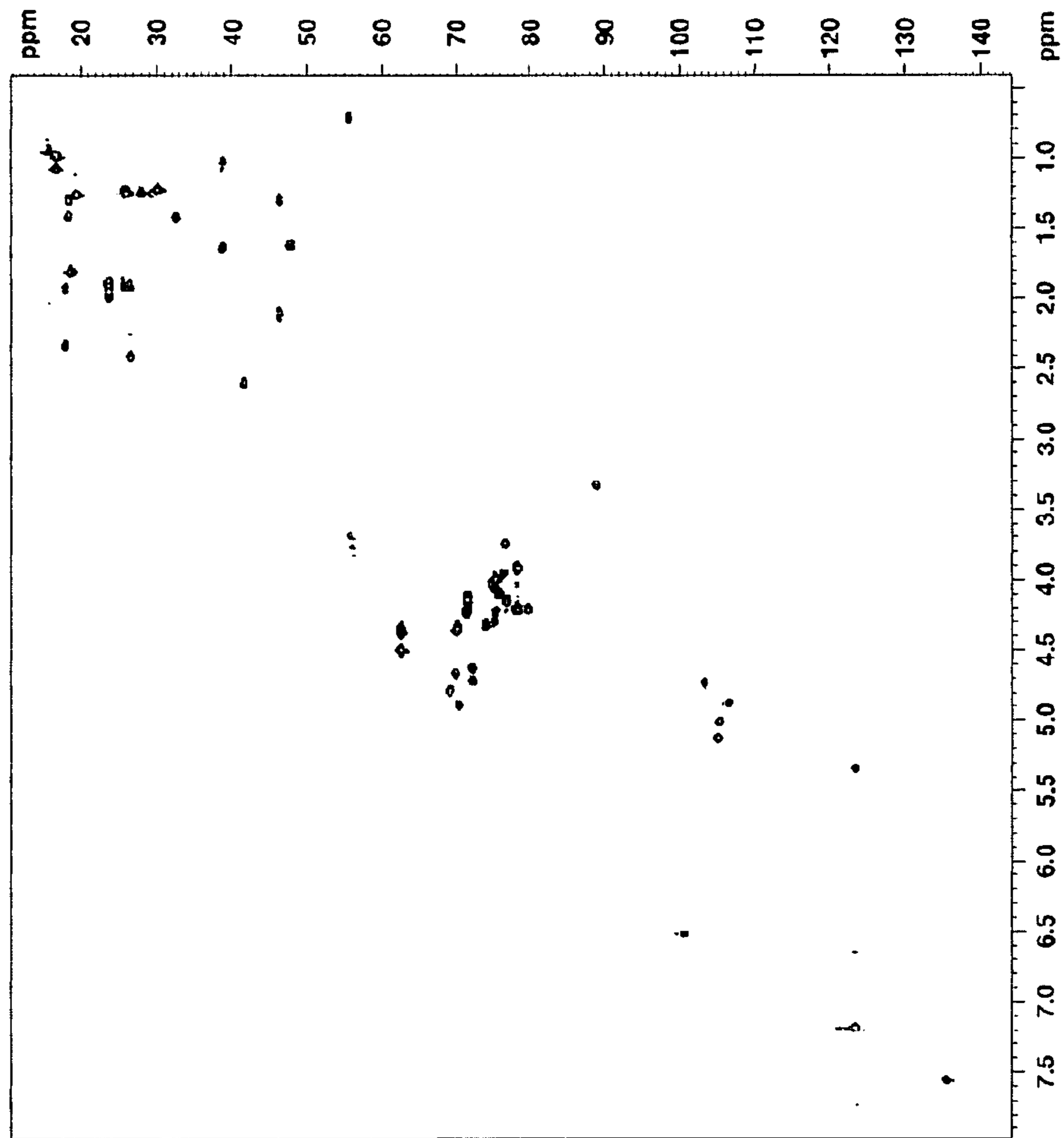
Figure 55 O54-HMQC
