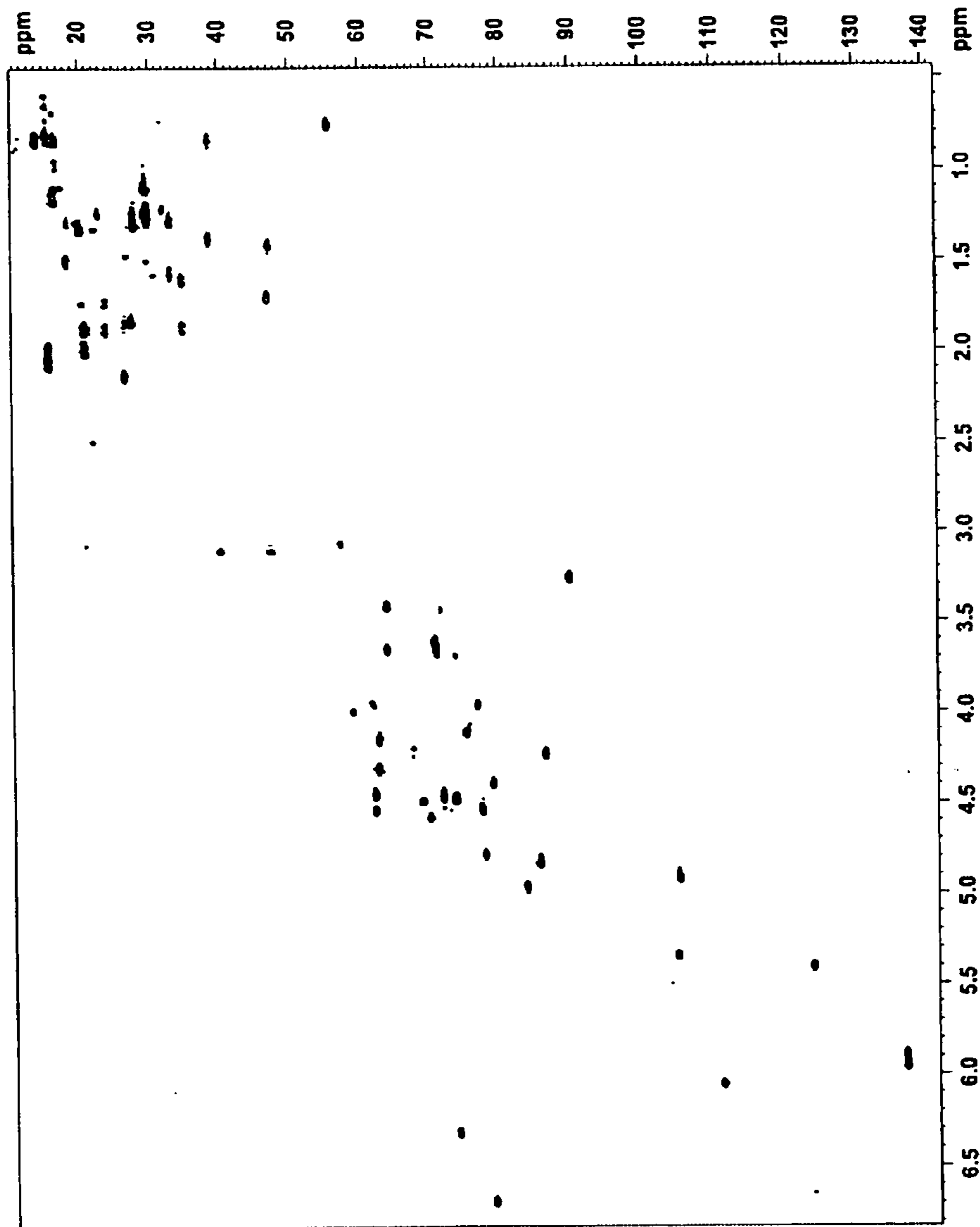
Figure 46 Y10-HMQC-level-1
