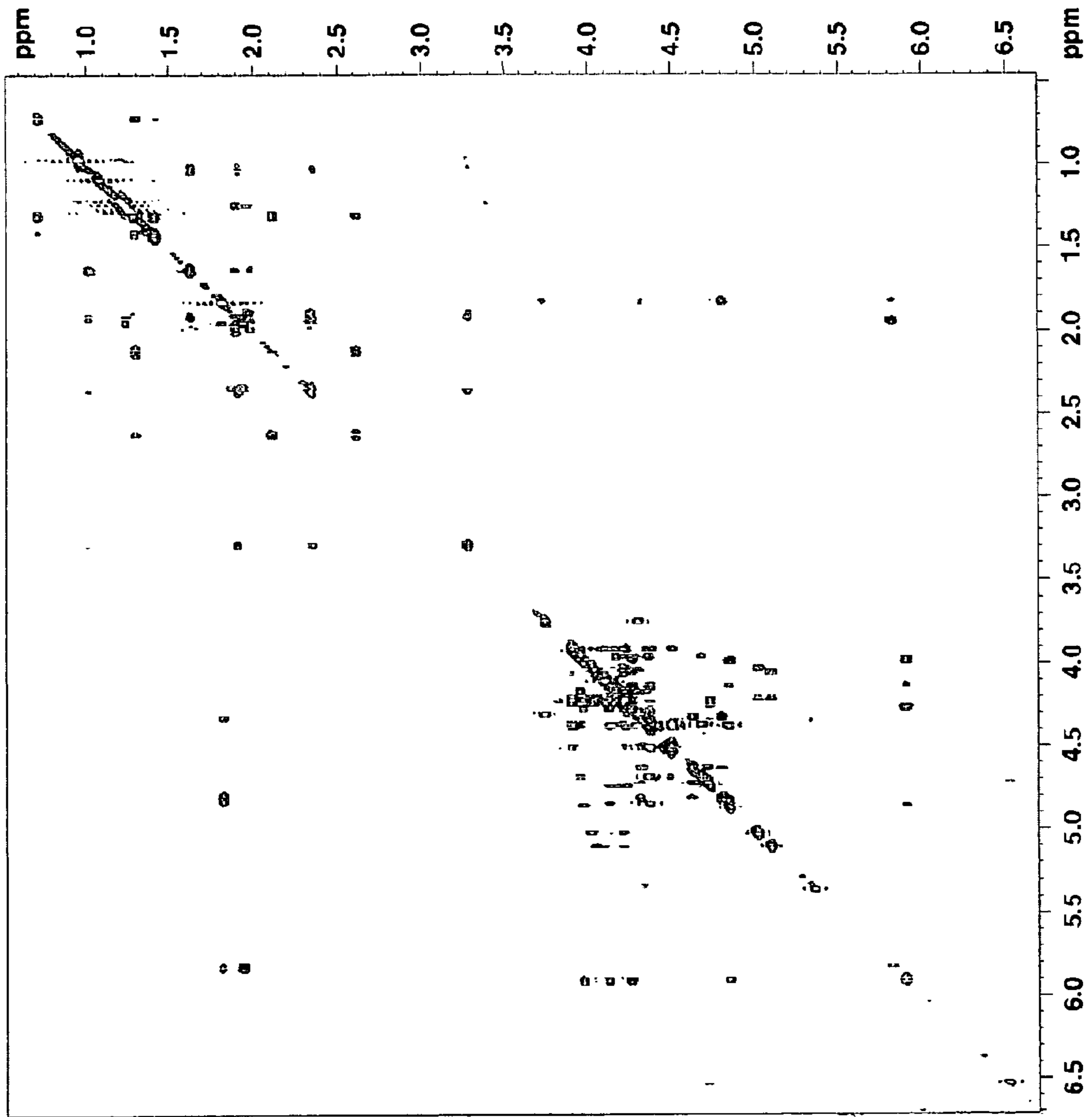
Figure 51 R1-COSY
