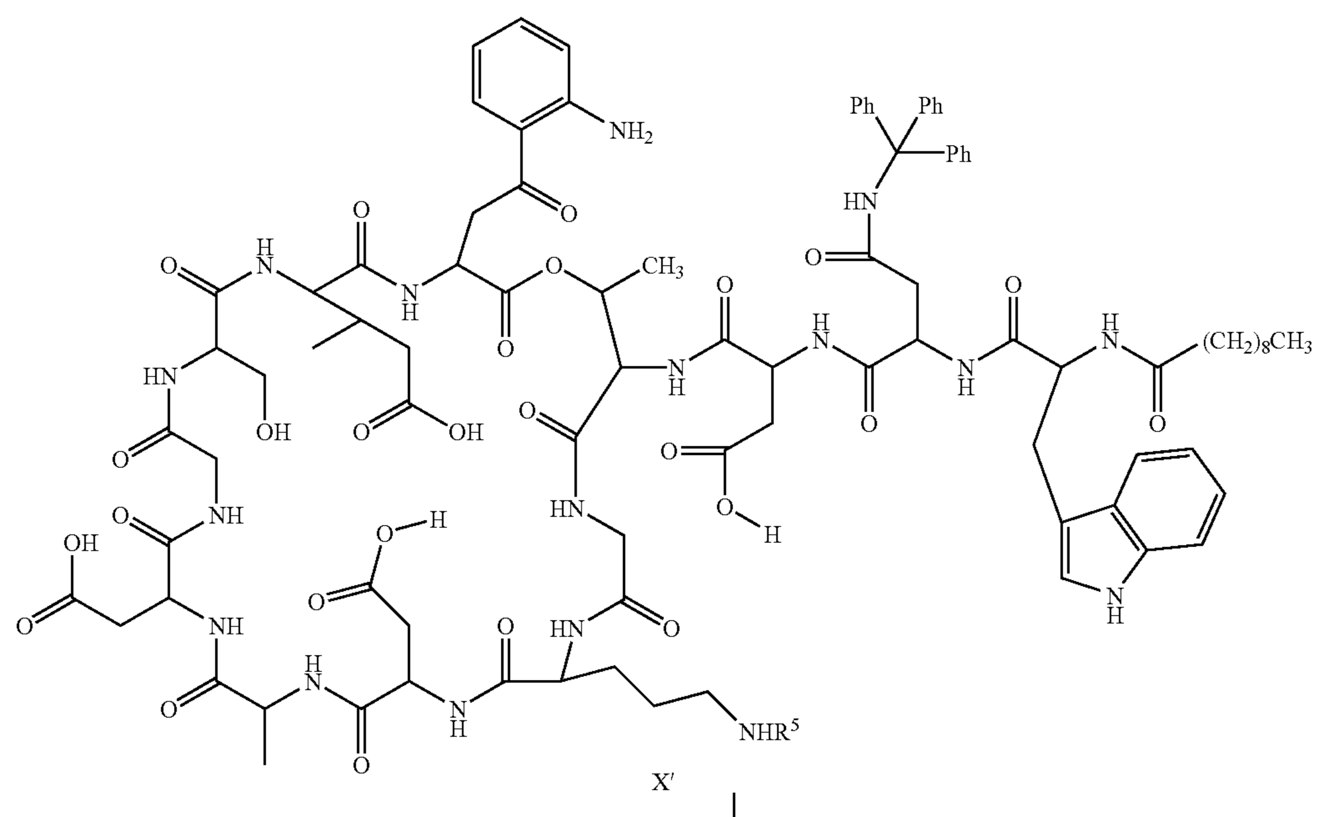
Scheme V
