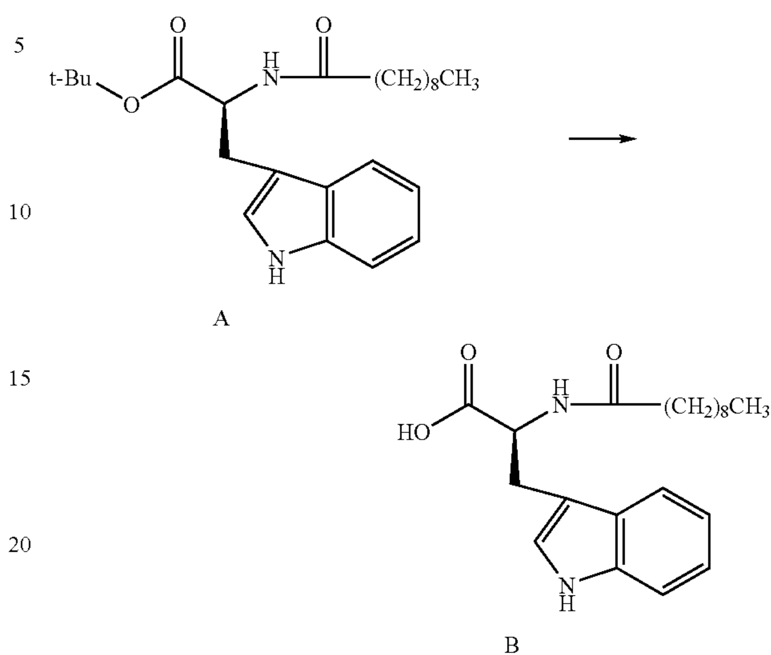
Reaction 2
