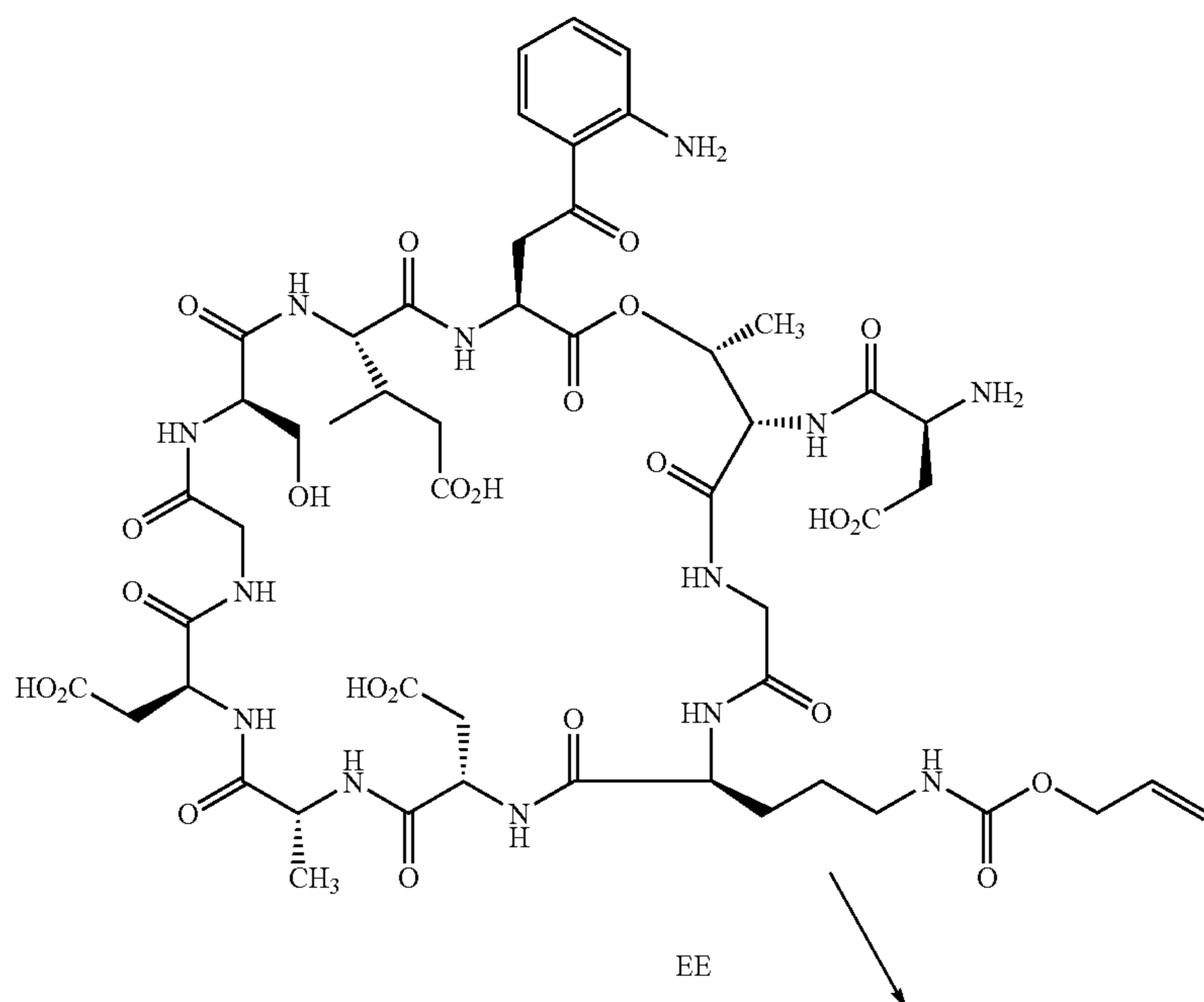
Reaction 1
