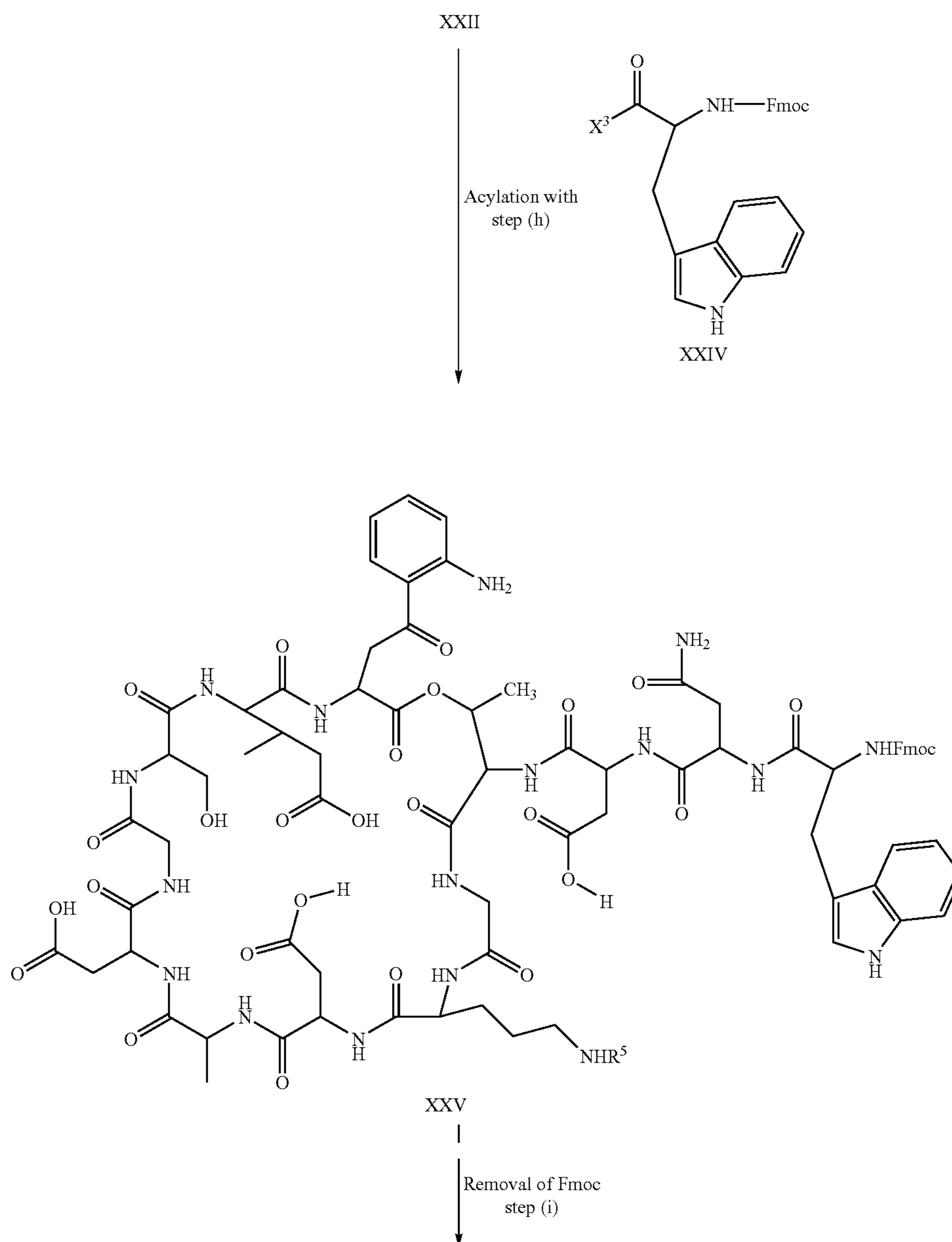
Scheme VII
