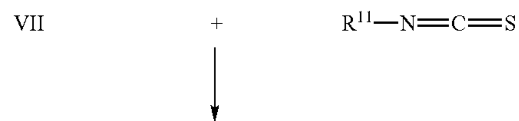
Scheme IV
