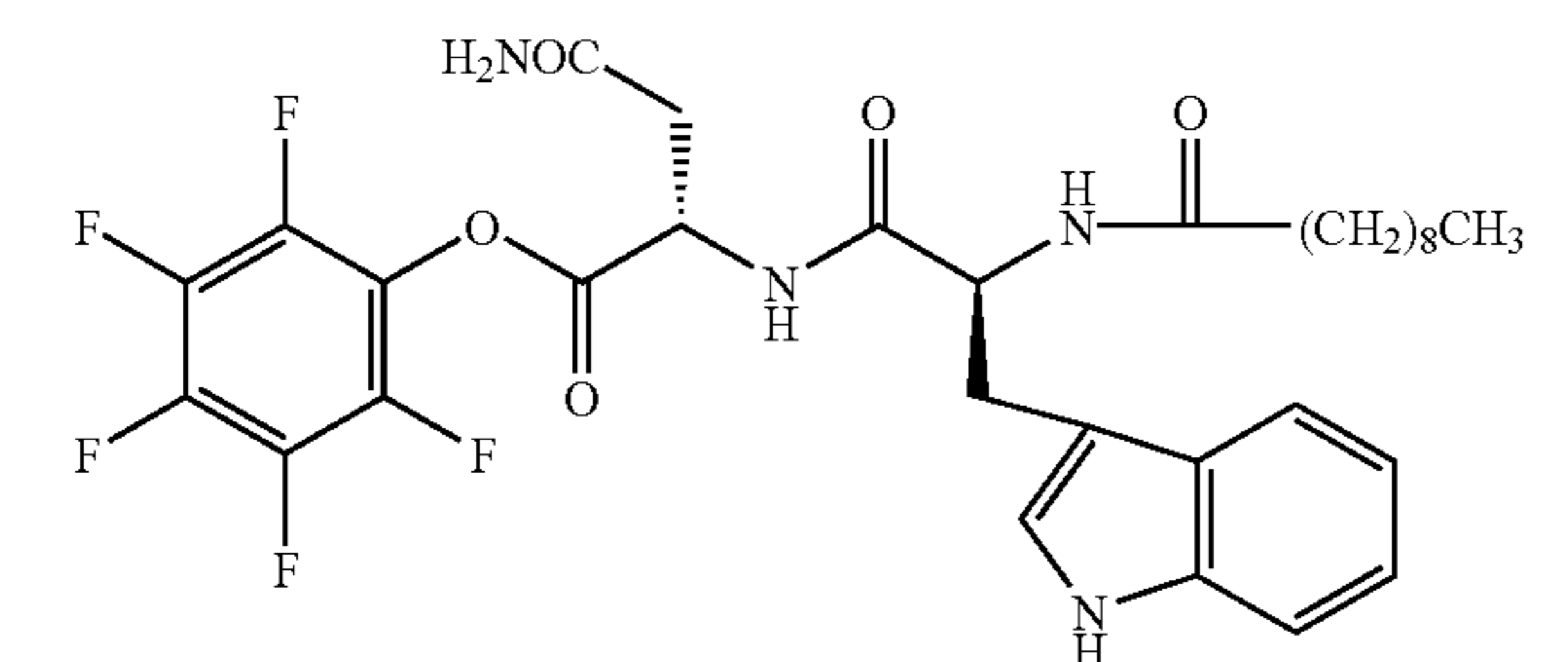
Reaction 1
