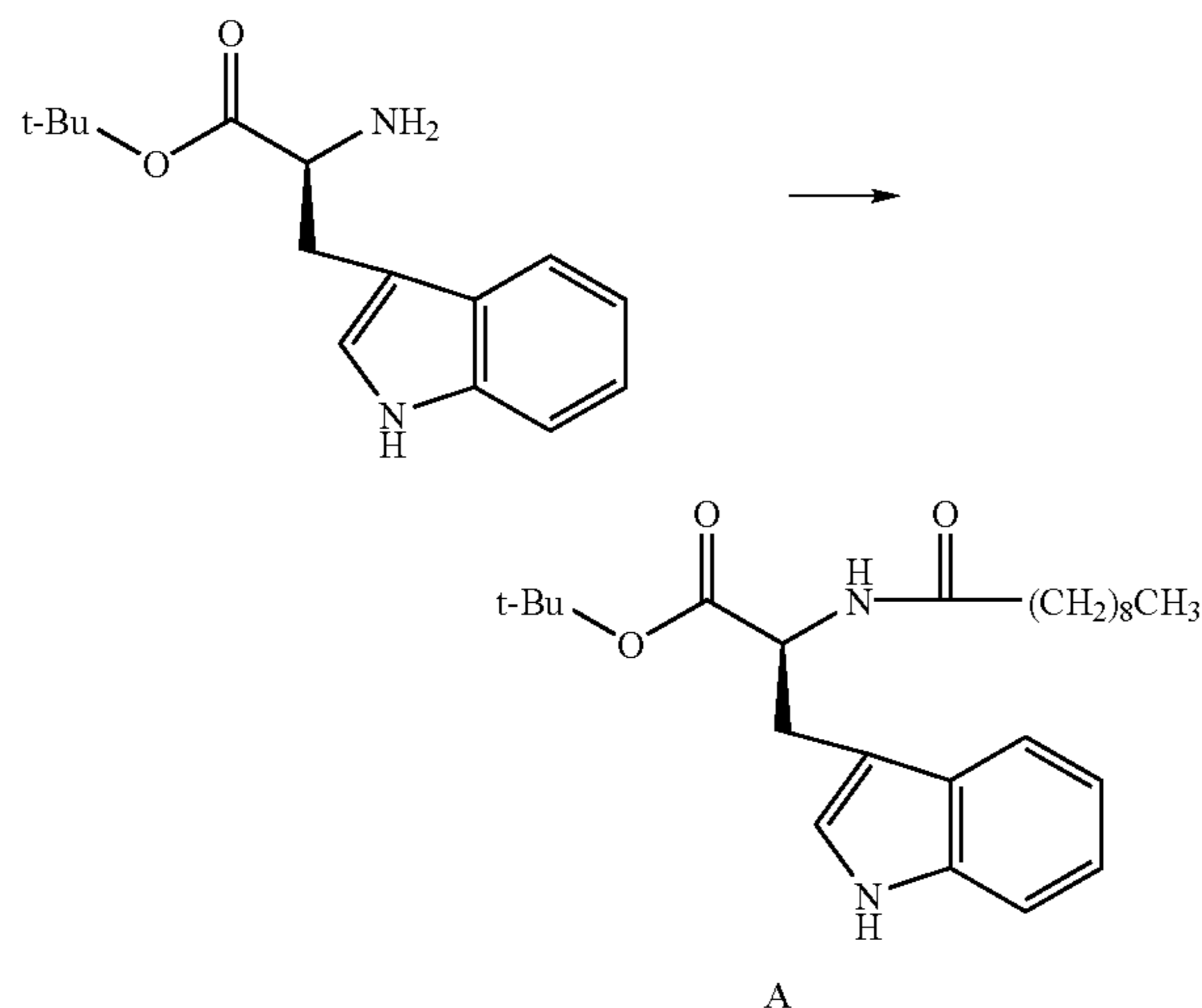
Reaction 1
