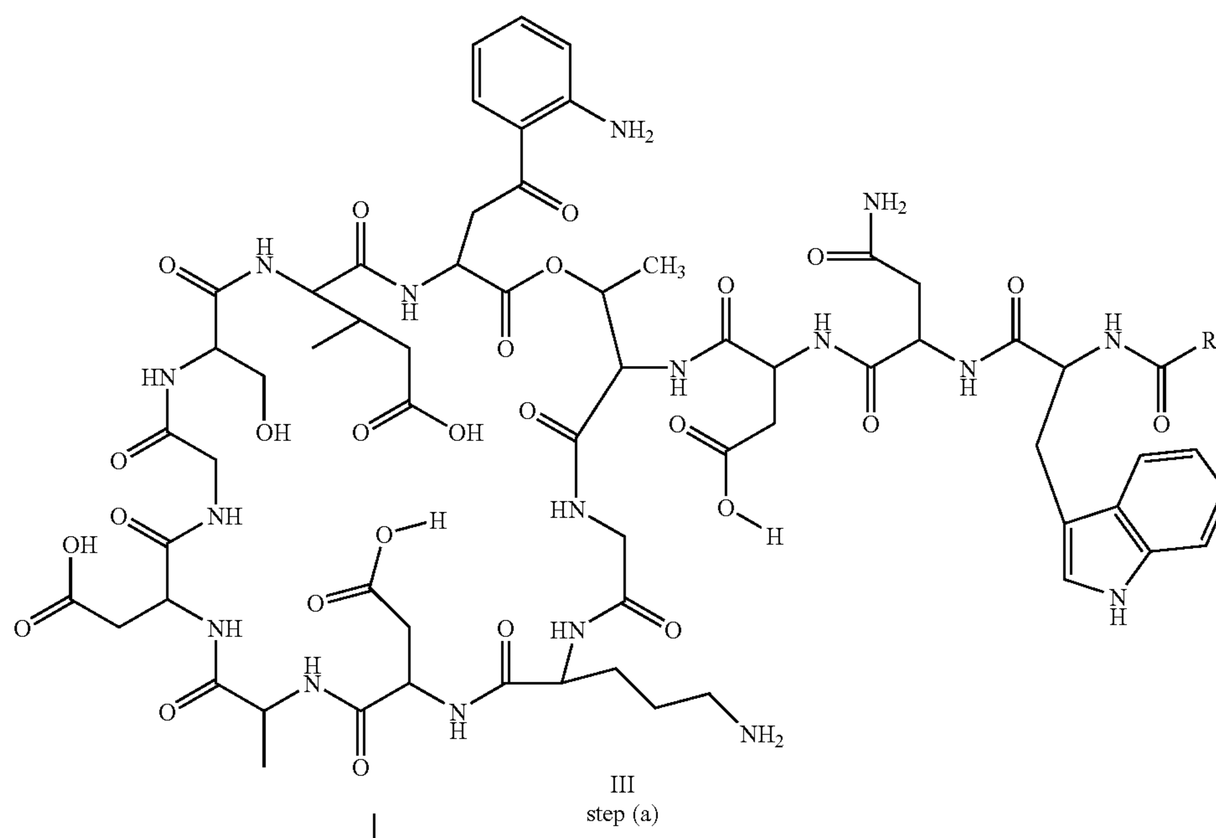
Scheme I
