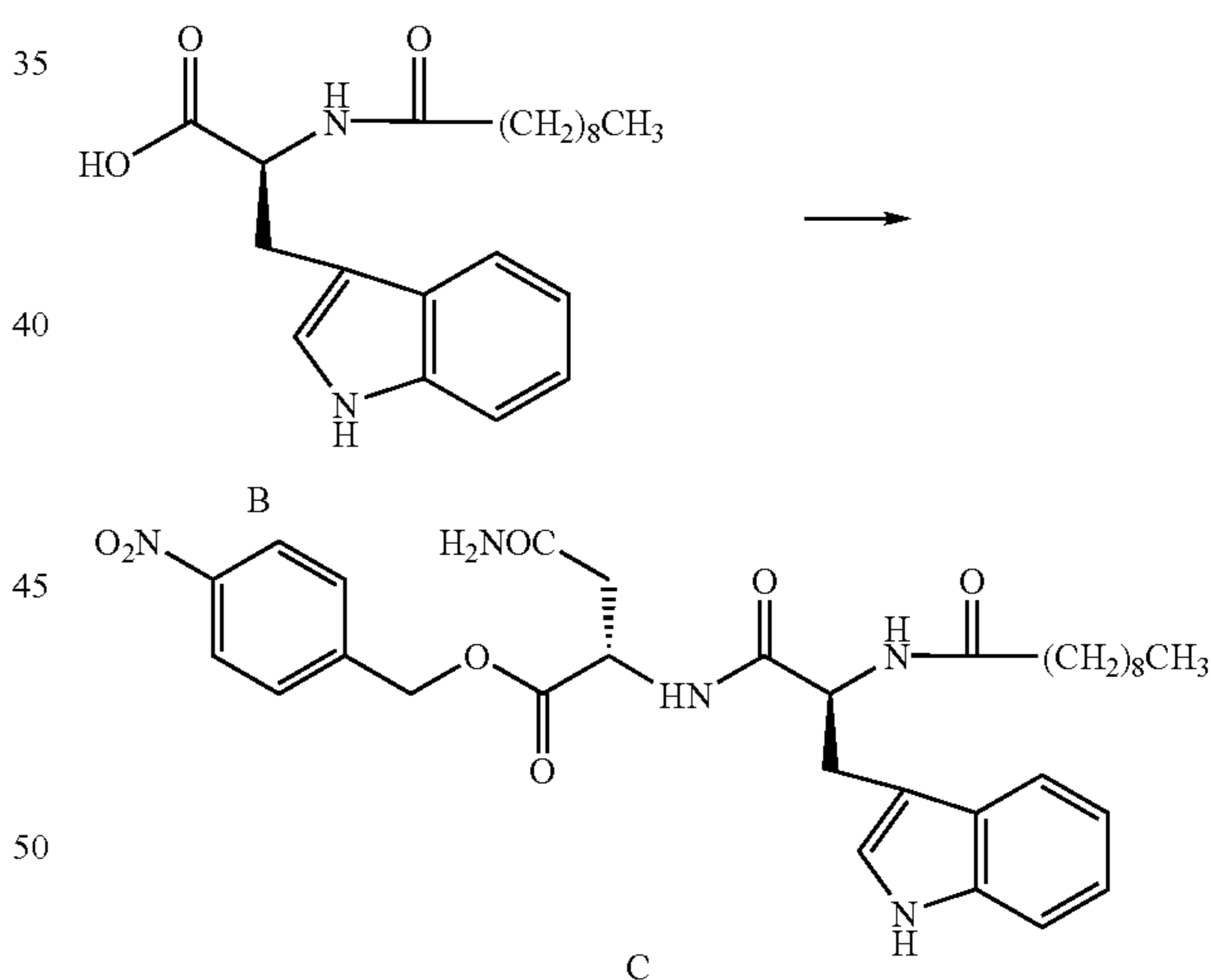
Reaction 3
