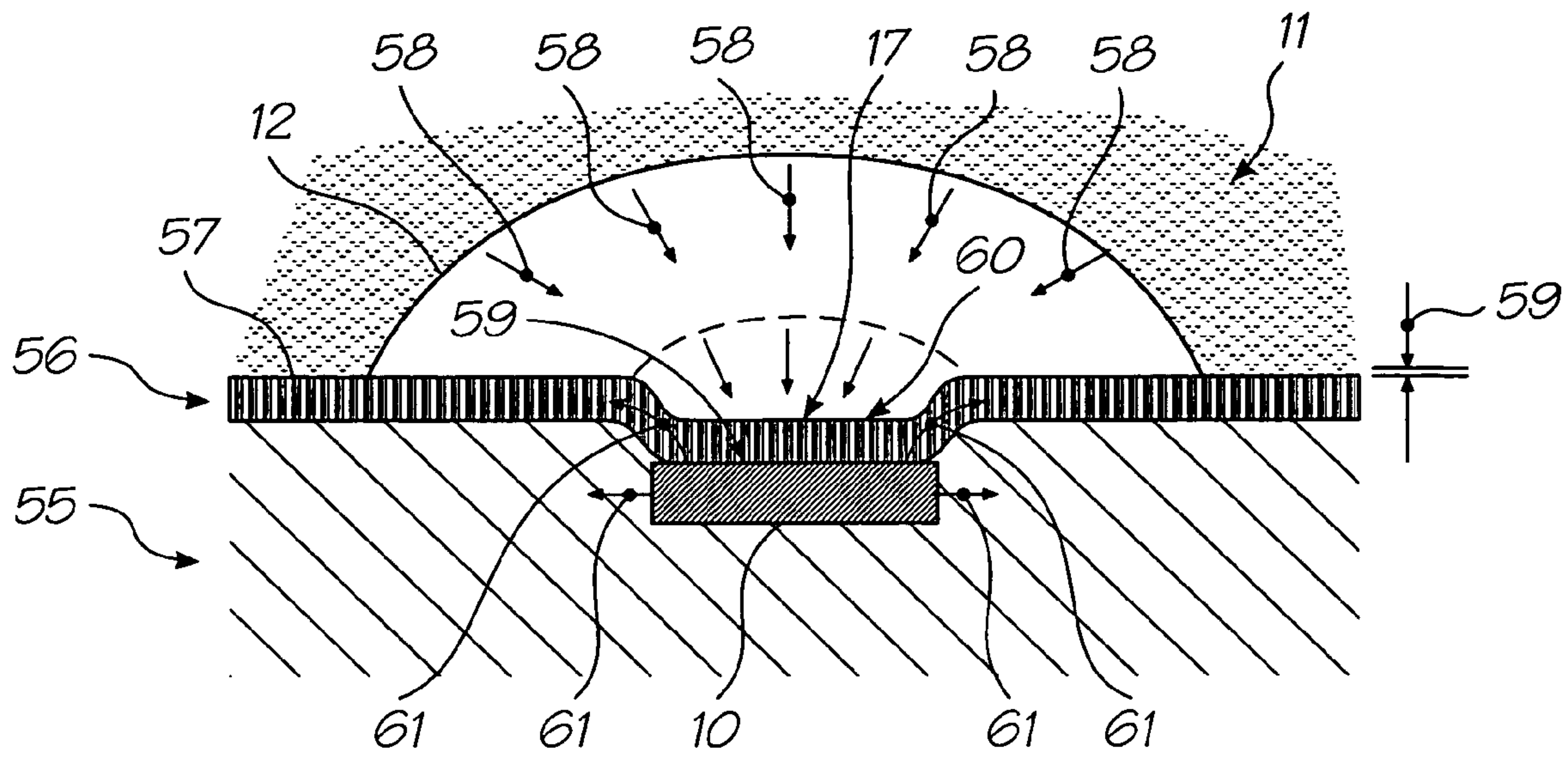
FIG. 57 (PRIOR ART)
