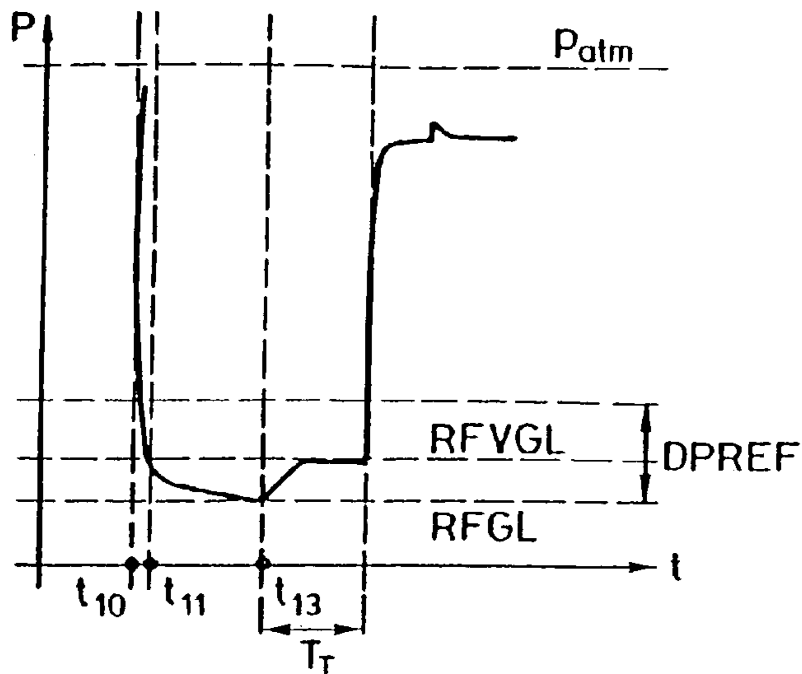
EVAC TEST VENT
