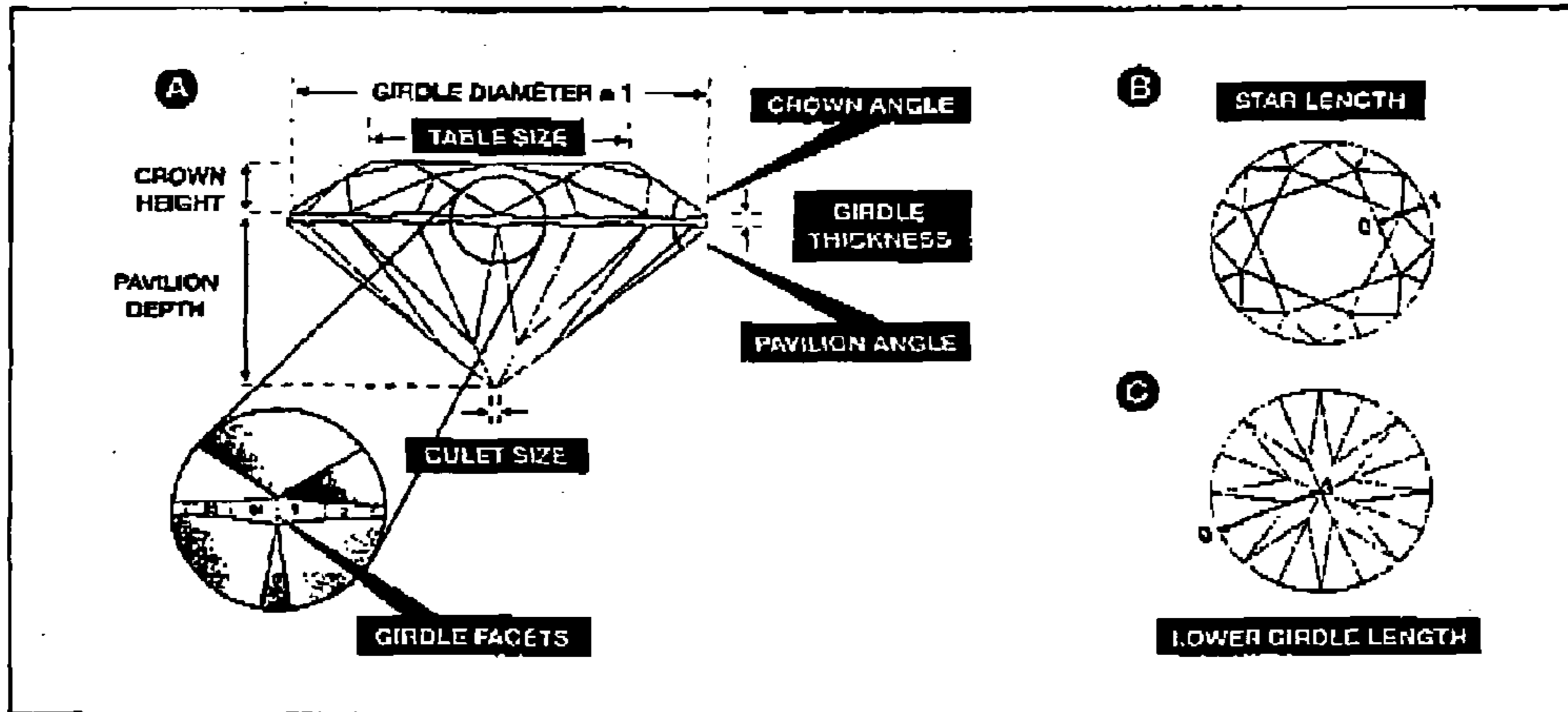
Figure A-1. We used eight parameters—varied across the range given in table 4—to define our geometric model of the round brilliant shape. (A) All linear distances in this profile view can be described as a percentage of the girdle diameter. The enlarged view of the girdle is centered on the position where we measured the girdle thickness. (B) In this view of the table, the star length is shown at 50%, so that the star facets extend halfway from the table to the girdle (when viewed from straight above). (C) In this view of the pavilion, the lower-girdle length is shown at 75%, so that the lower girdle facets extend three-fourths of the distance from the girdle to the culet (when viewed from straight below).
