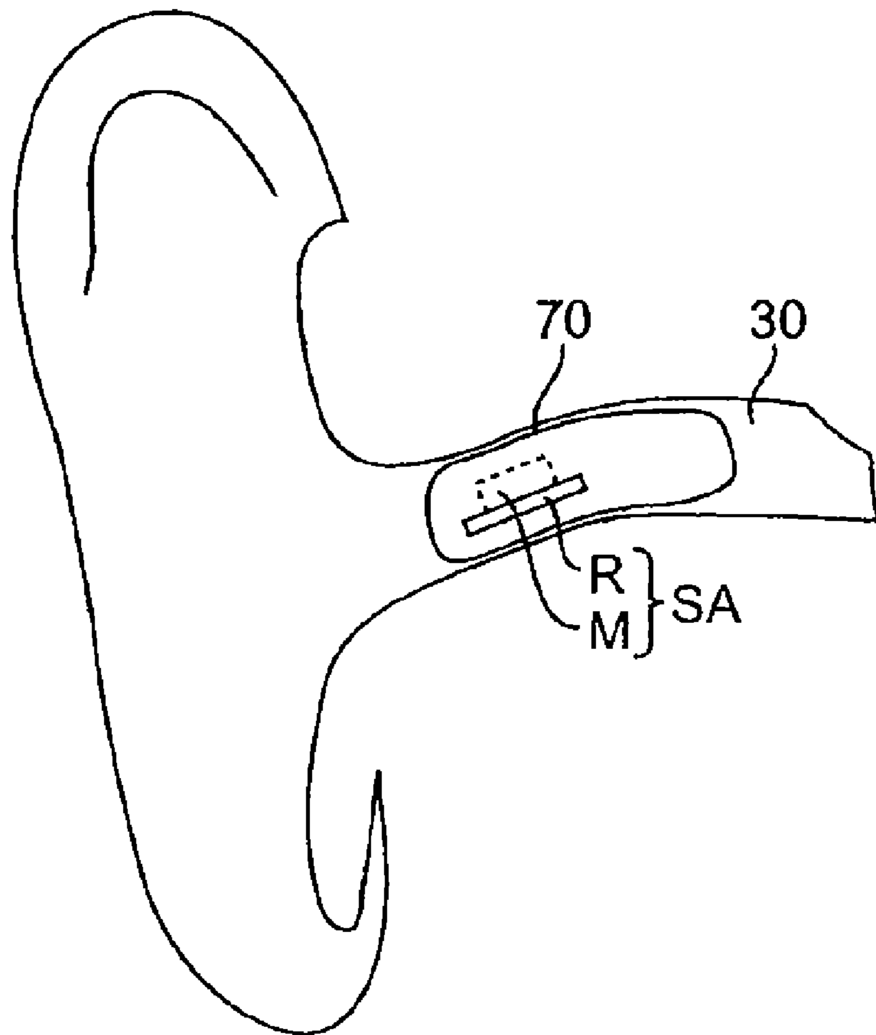
FIG. 3 PRIOR ART
