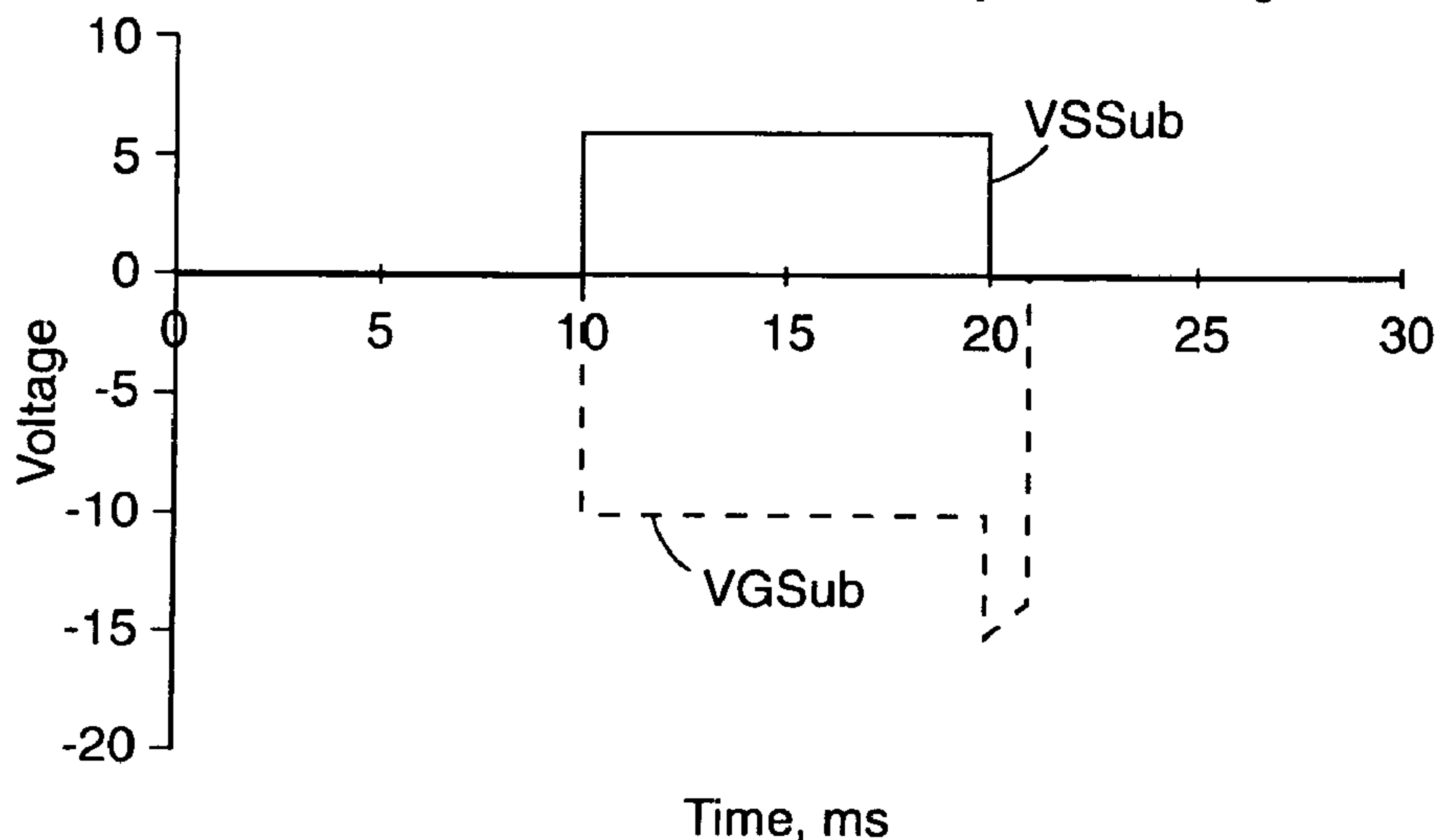
Source erase with delayed gate discharge
