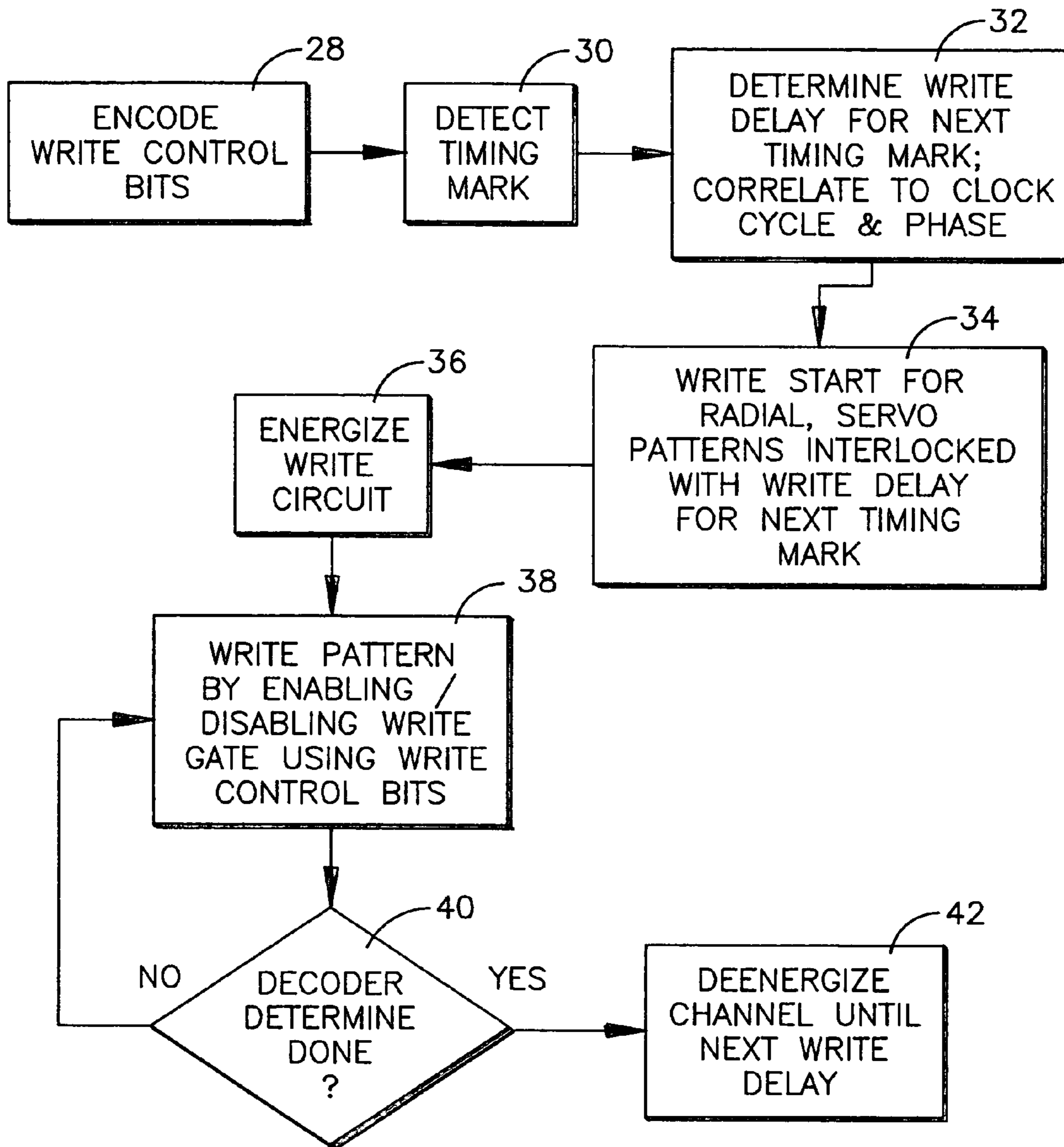
Fig. 3 LOGIC
