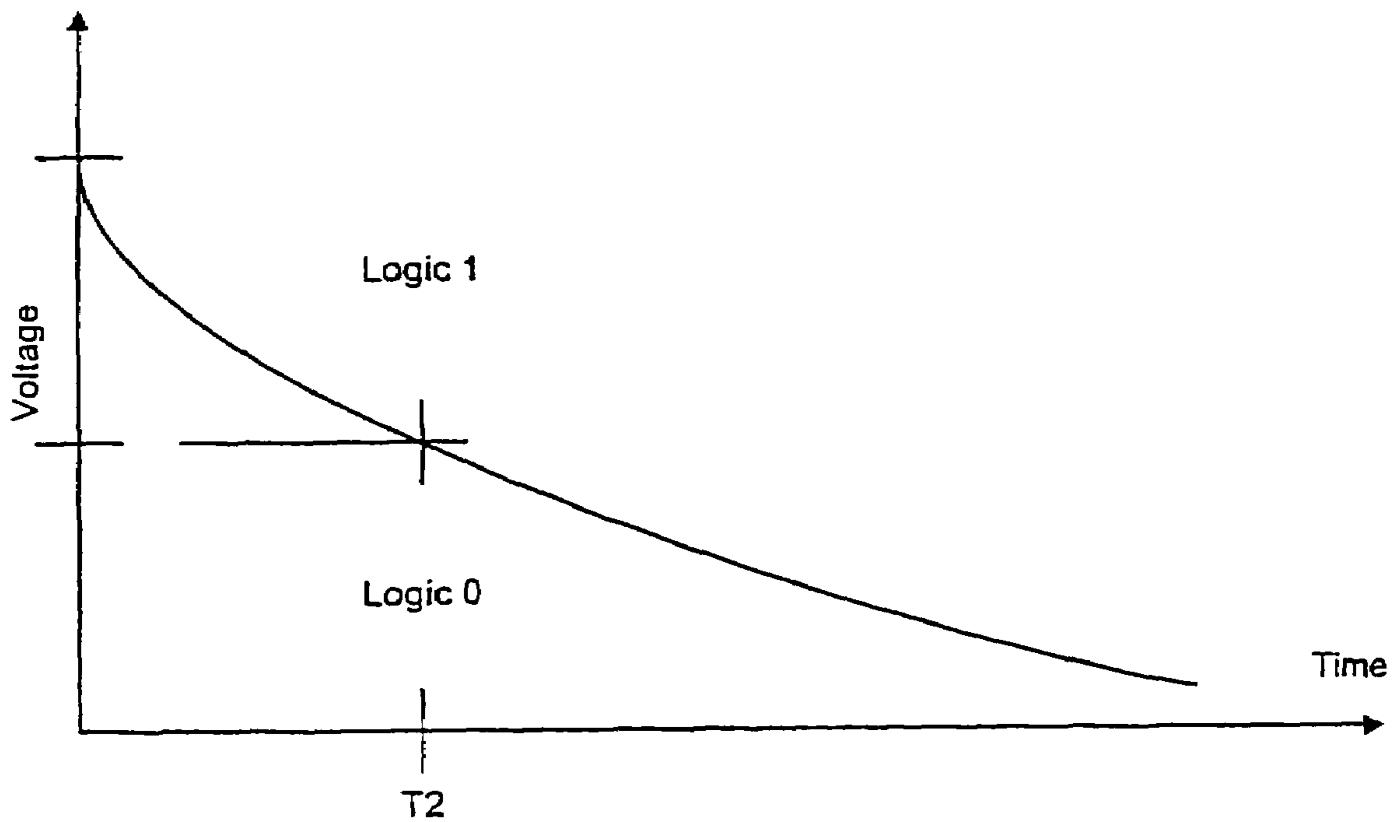
Figure 4(b) Discharge Waveform of Valid DRAM Bit
