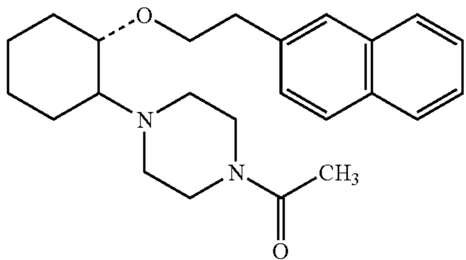
(1R,2R)/(1S,2S)-2-(1-acetylpiperazinyl)-1-(2-naphthenethoxy)cyclohexane
