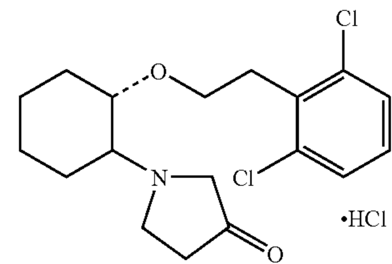
(1R,2R)/(1S,2S)-2-(3-ketopyrrolidinyl)-1-(2,6-dichlorophenethoxy)cyclohexane
