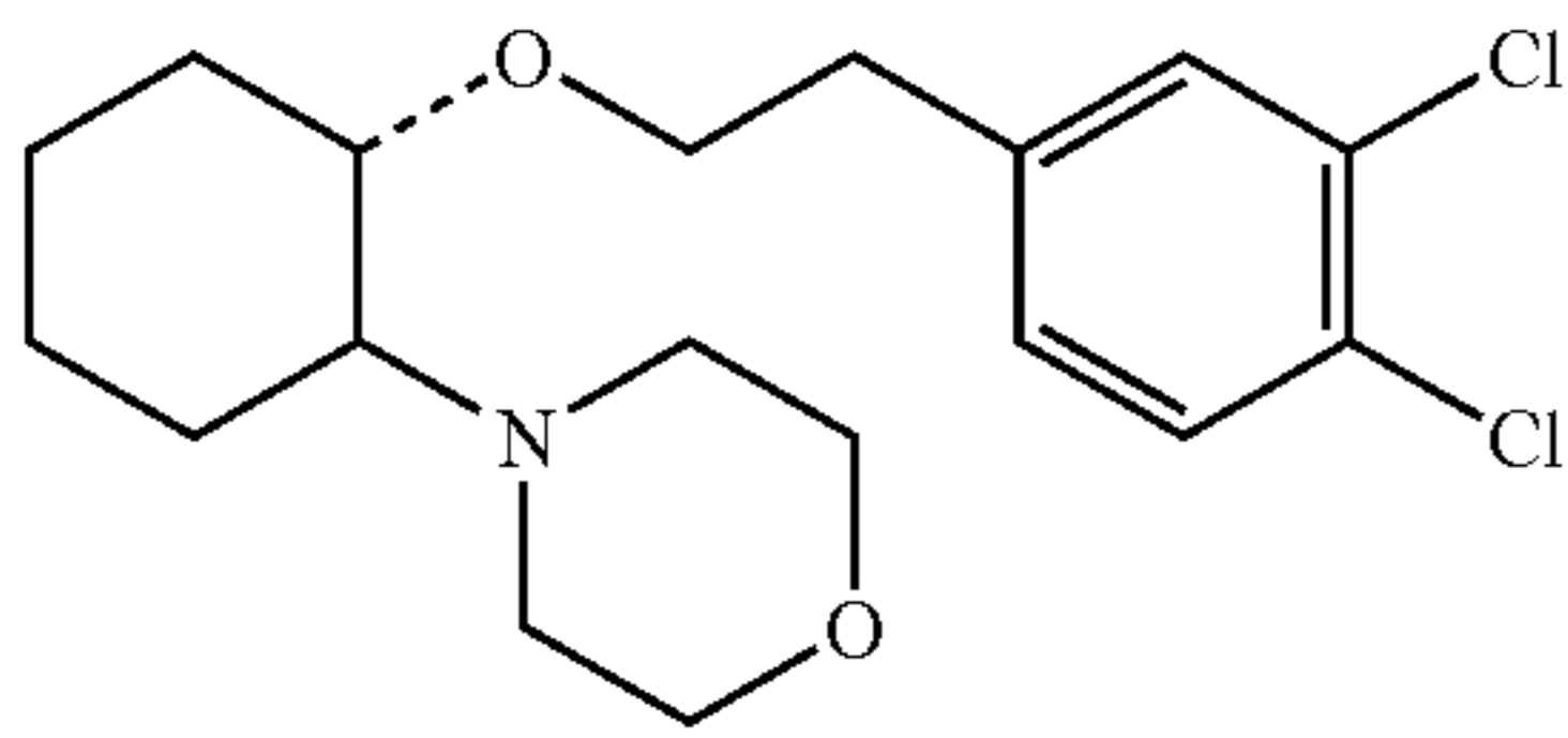
(1R,2R)/(1S,2S)-2-(4-morpholinyl)-1-(3,4-dichlorophenethoxy)cyclohexane
