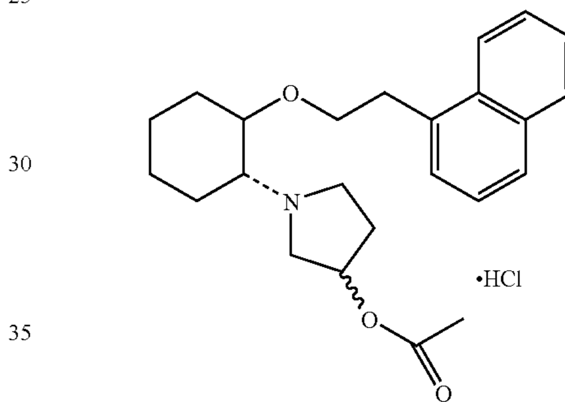
(1R,2R)/(1S,2S)-2-(3-acetoxypyrrrolidinyl)-1-(1-naphthenethoxy)cyclohexane monohydrochloride
