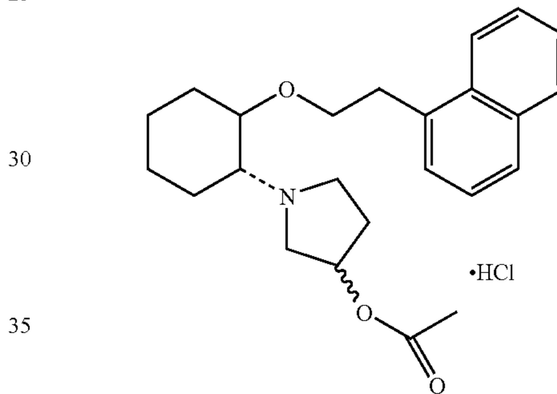
(1R,2R)/(1S,2S)-2-(3-acetoxypyrrrolidinyl)-1-(1-naphthenethoxy)cyclohexane monohydrochloride
