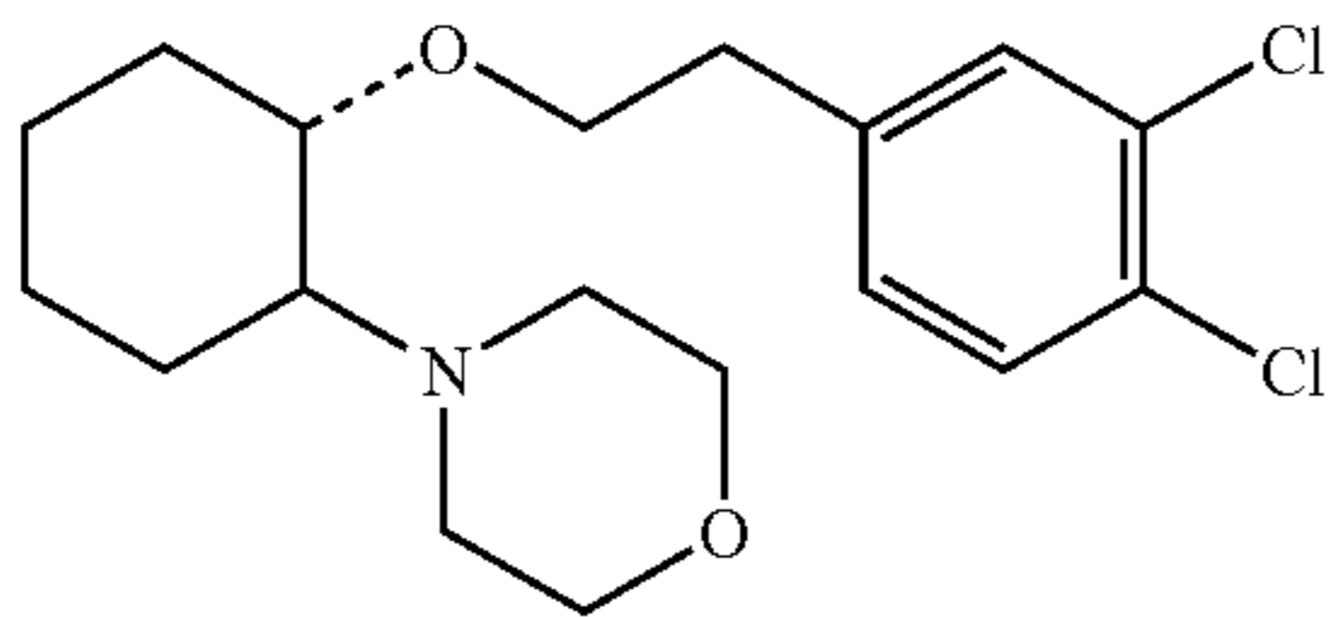
(1R,2R)/(1S,2S)-2-(4-morpholinyl)-1-(3,4-dichlorophenethoxy)cyclohexane
