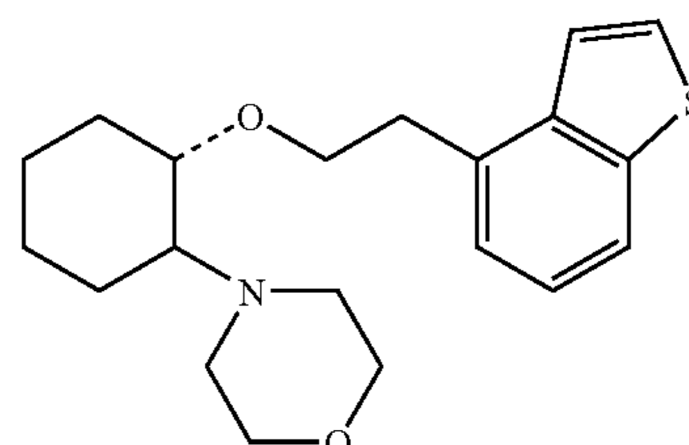
(1R,2R)/(1S,2S)-[2-(4-morpholinyl)-1-(2-benzo[b]thiophen-4-yl)]cyclohexane
