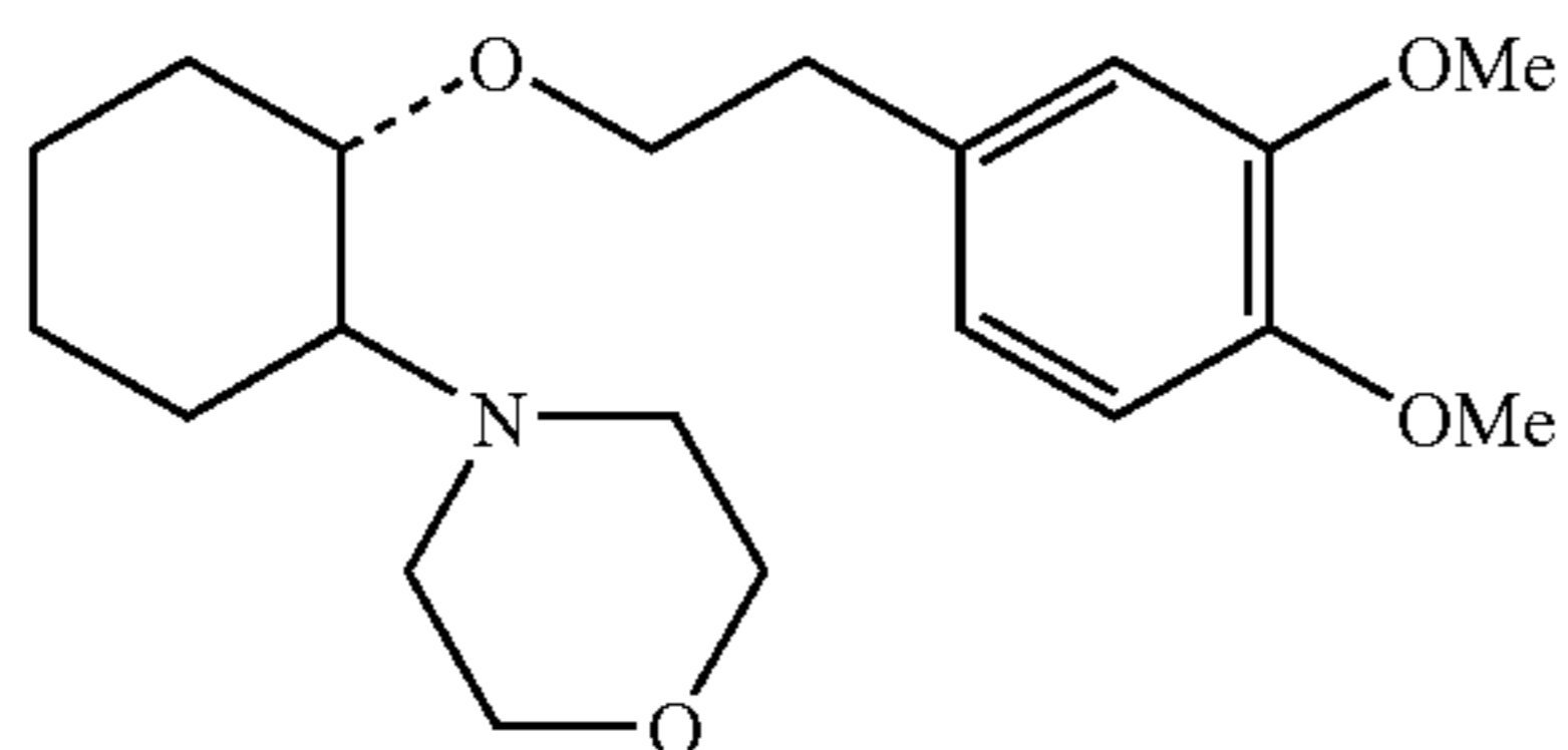
(1R,2R)/(1S,2S)-[2-(4-morpholinyl)-1-(3,4-dimethoxyphenethoxy)]cyclohexane
