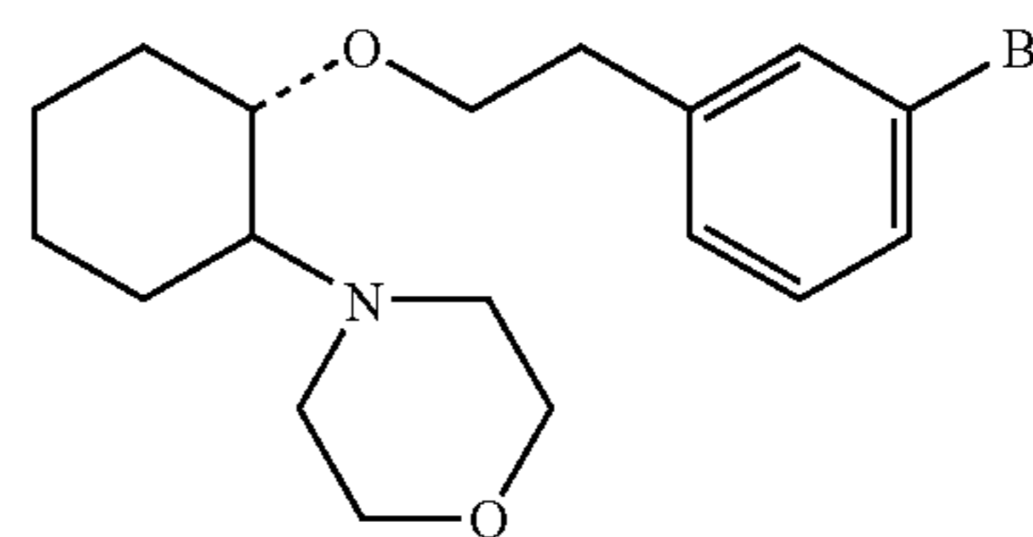
(1R,2R)/(1S,2S)-[2-(4-morpholinyl)-1-(3-bromophenethoxy)]cyclohexane
