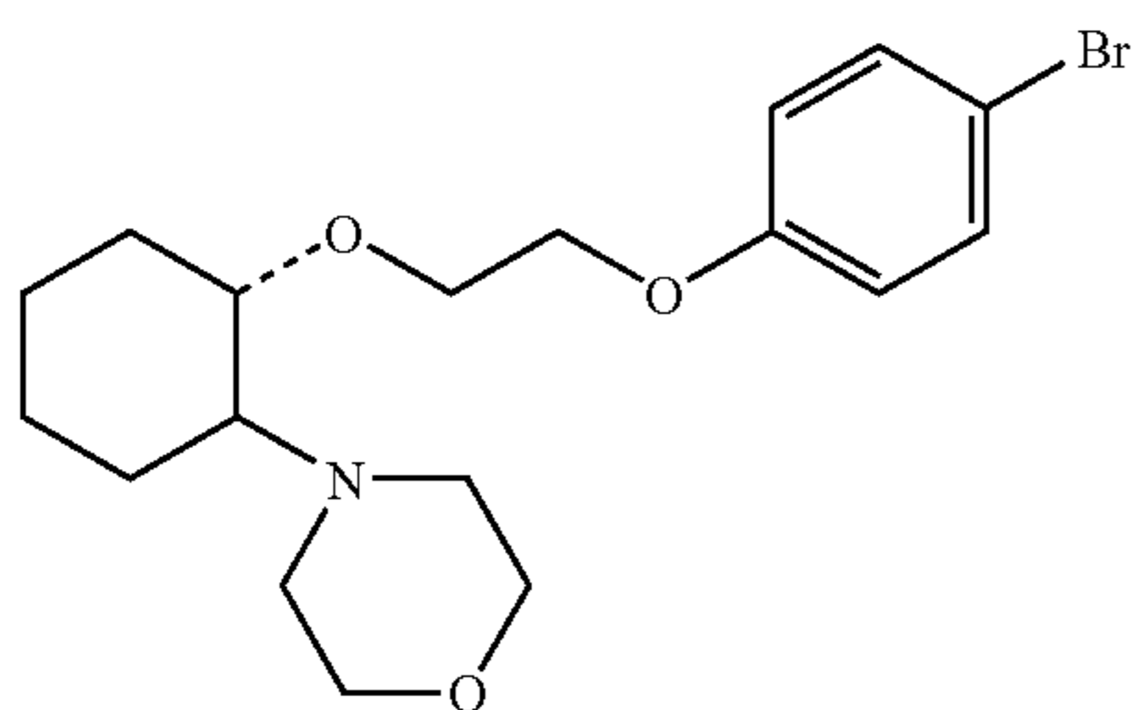
(1R,2R)/(1S,2S)-[2-(4-morpholinyl)-1-[2-(4-bromophenoxy)ethoxy]]cyclohexane
