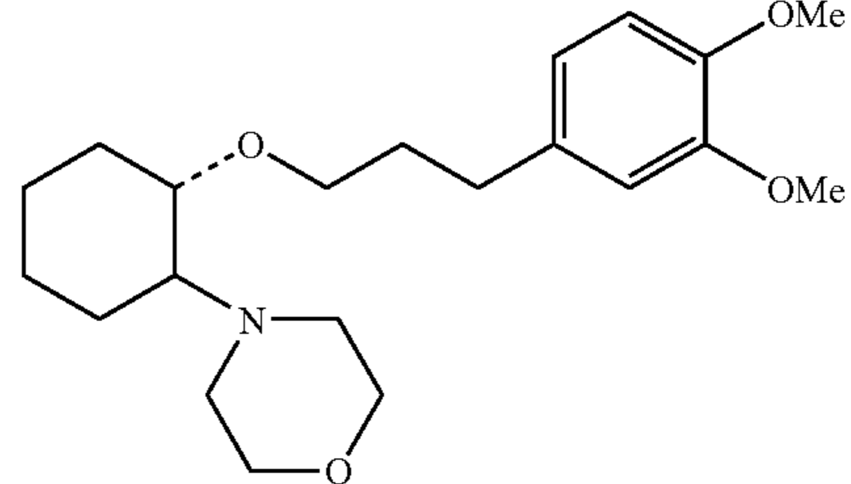
(1R,2R)/(1S,2S)-[2-(4-morpholinyl)-1-(3-(3,4-dimethoxyphenyl)propoxy)]cyclohexane
