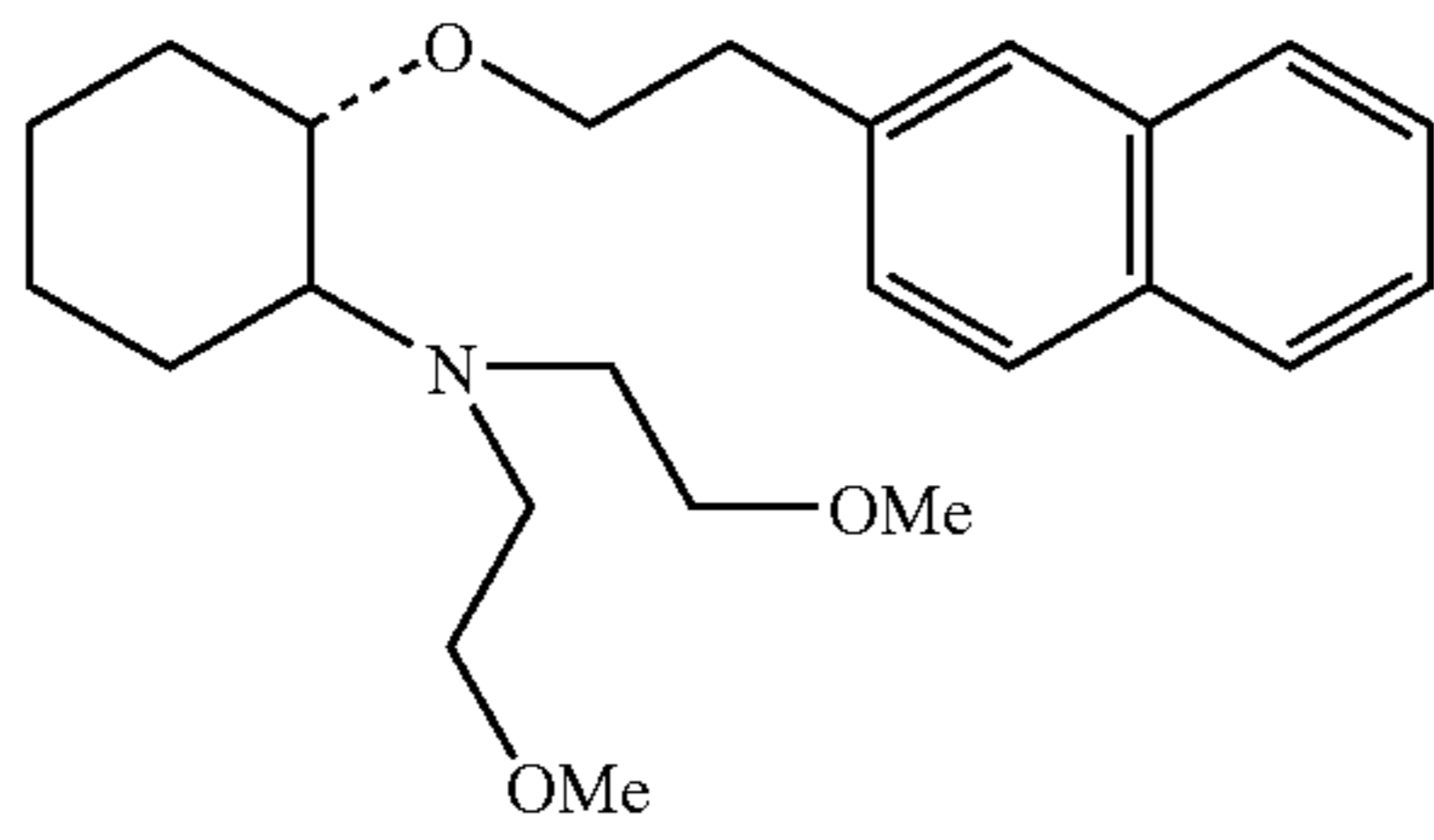
(1R,2R)/(1S,2S)-[2-[bis(2-methoxyethyl)aminy]-1-(2-naphthenethoxy)]cyclohexane
