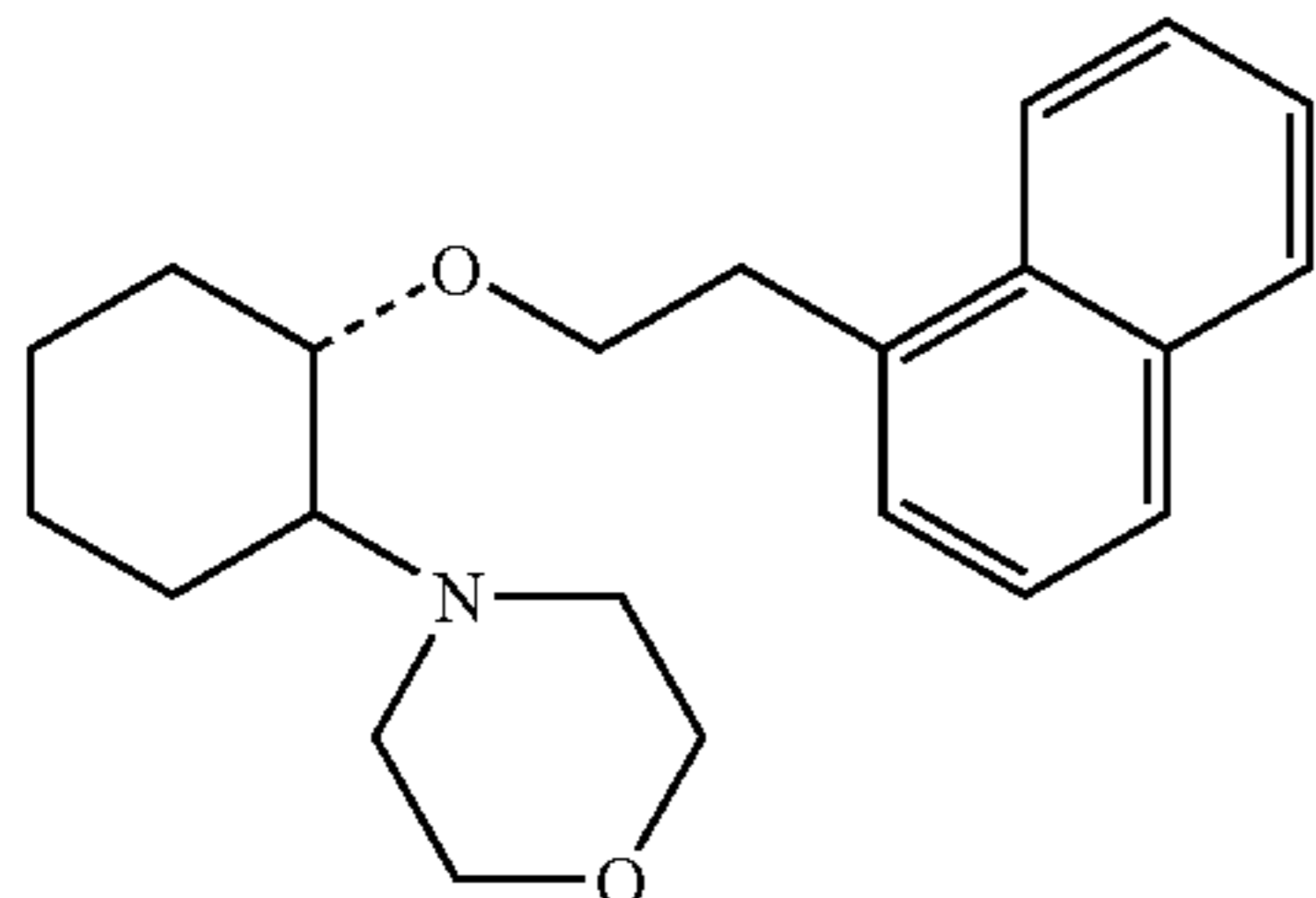
(1R,2R)/(1S,2S)-[2-(4-morpholinyl)-1-(1-naphthenethoxy)]cyclohexane
