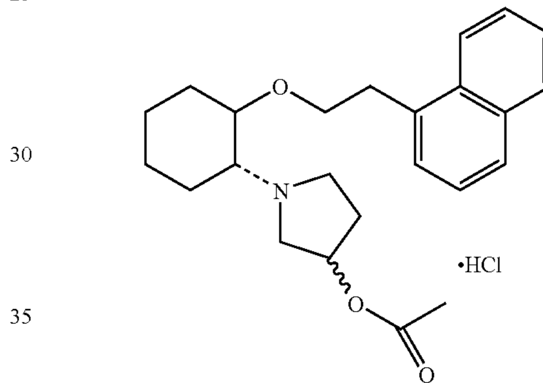
(1R,2R)/(1S,2S)-2-(3-acetoxypyrrrolidinyl)-1-(1-naphthenethoxy)cyclohexane monohydrochloride
