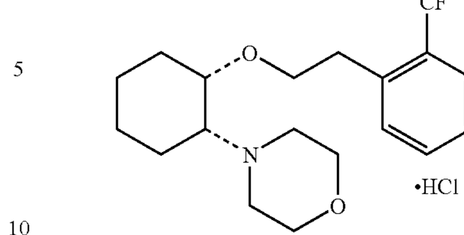
(1R,2S)/(1S,2R)-2-(4-morpholinyl)-1-[(2-trifluoromethyl)phenethoxy]cyclohexane monohydrochloride
