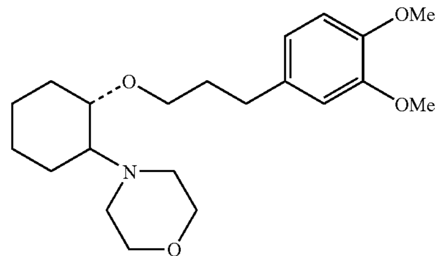
(1R,2R)/(1S,2S)-[2-(4-morpholinyl)-1-(3-(3,4-dimethoxyphenyl)propoxy)]cyclohexane
