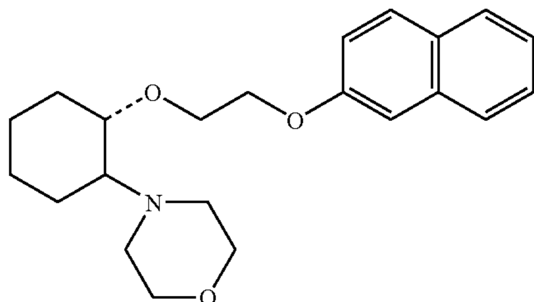
(1R,2R)/(1S,2S)-[2-(4-morpholinyl)-1-[2-(2-naphthoxy)ethoxy]]cyclohexane
