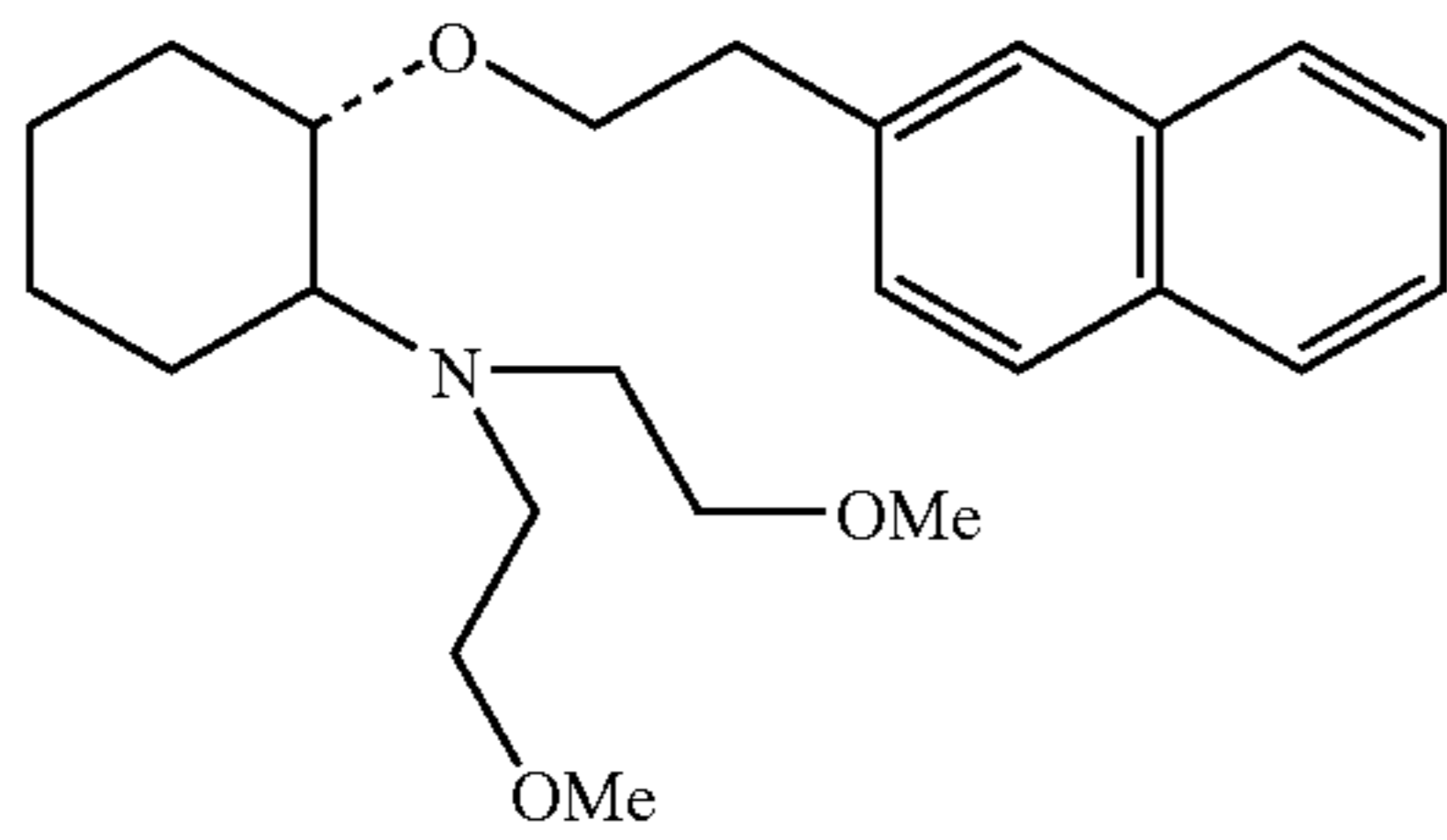
(1R,2R)/(1S,2S)-[2-[bis(2-methoxyethyl)aminy]-1-(2-naphthenethoxy)]cyclohexane
