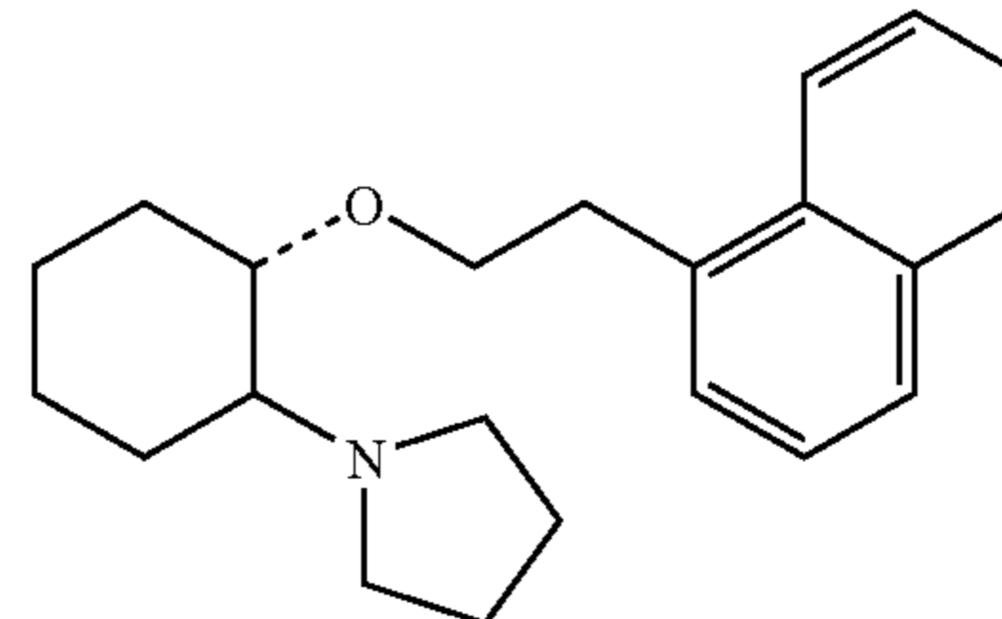
(1R,2R)/(1S,2S)-[2-(1-pyrrolidinyl)-1-(1-naphthenethoxy)]cyclohexane
