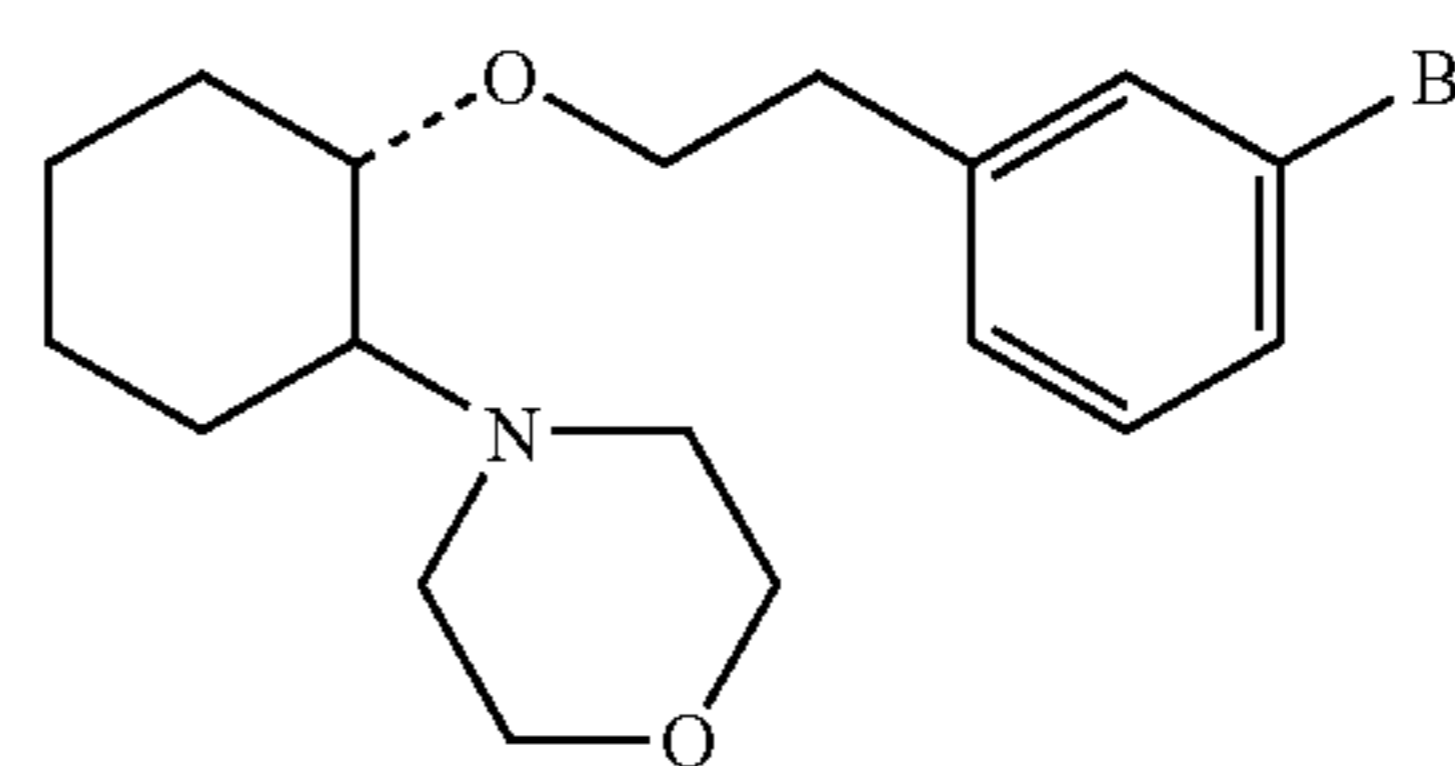
(1R,2R)/(1S,2S)-[2-(4-morpholinyl)-1-(3-bromophenethoxy)]cyclohexane
