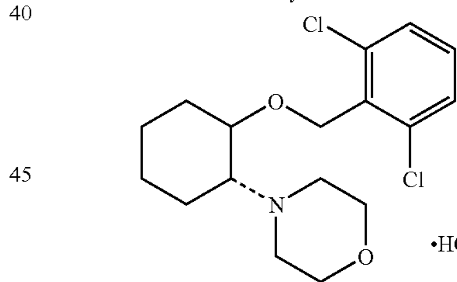
(1R,2R)/(1S,2S)-2-(4-morpholinyl)-1-[(2,6-dichlorophenyl)methoxy]cyclohexane monohydrochloride
