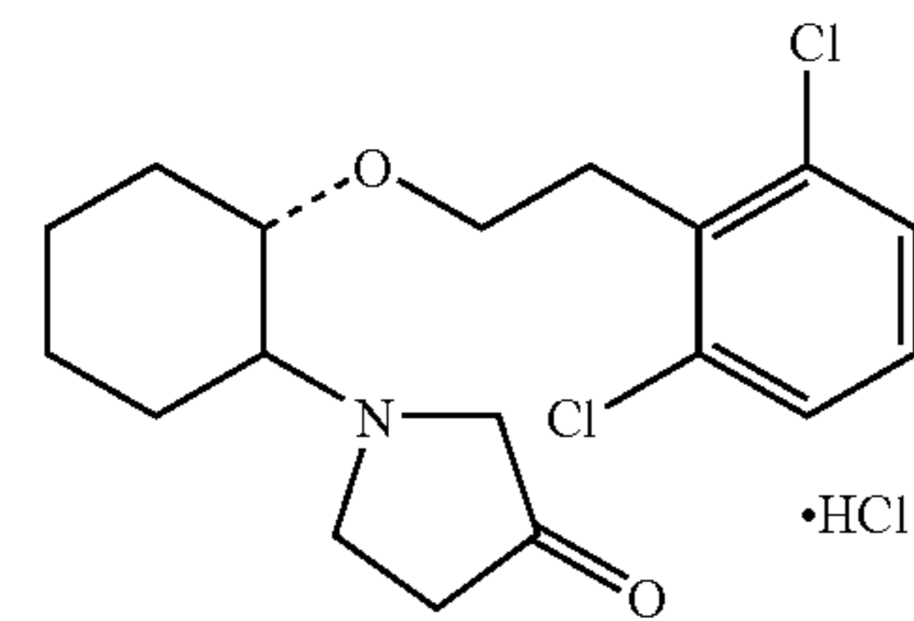
(1R,2R)/(1S,2S)-2-(3-ketopyrrolidinyl)-1-(2,6-dichlorophenethoxy)cyclohexane
