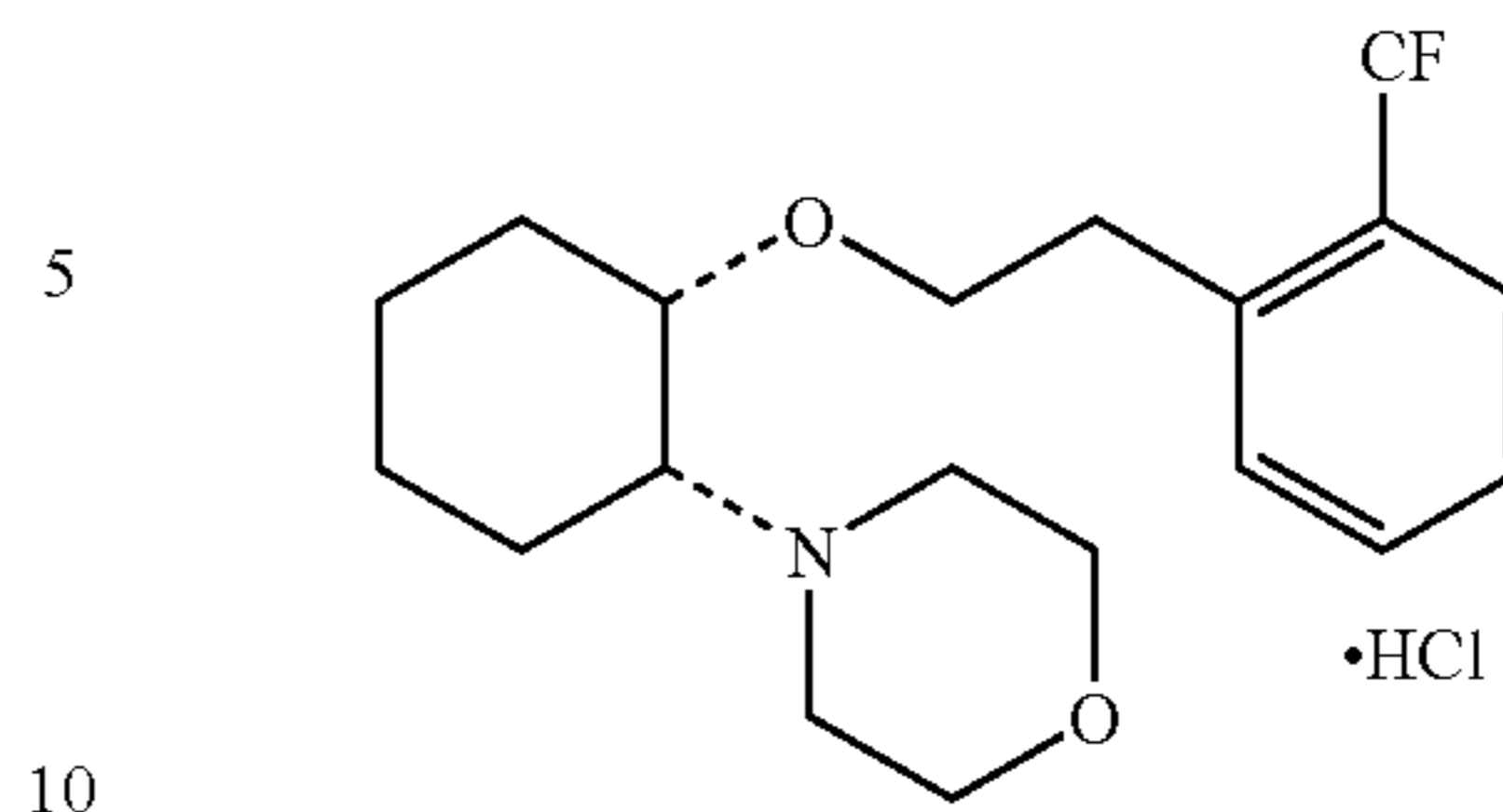
(1R,2S)/(1S,2R)-2-(4-morpholinyl)-1-[(2-trifluoromethyl)phenethoxy]cyclohexane monohydrochloride
