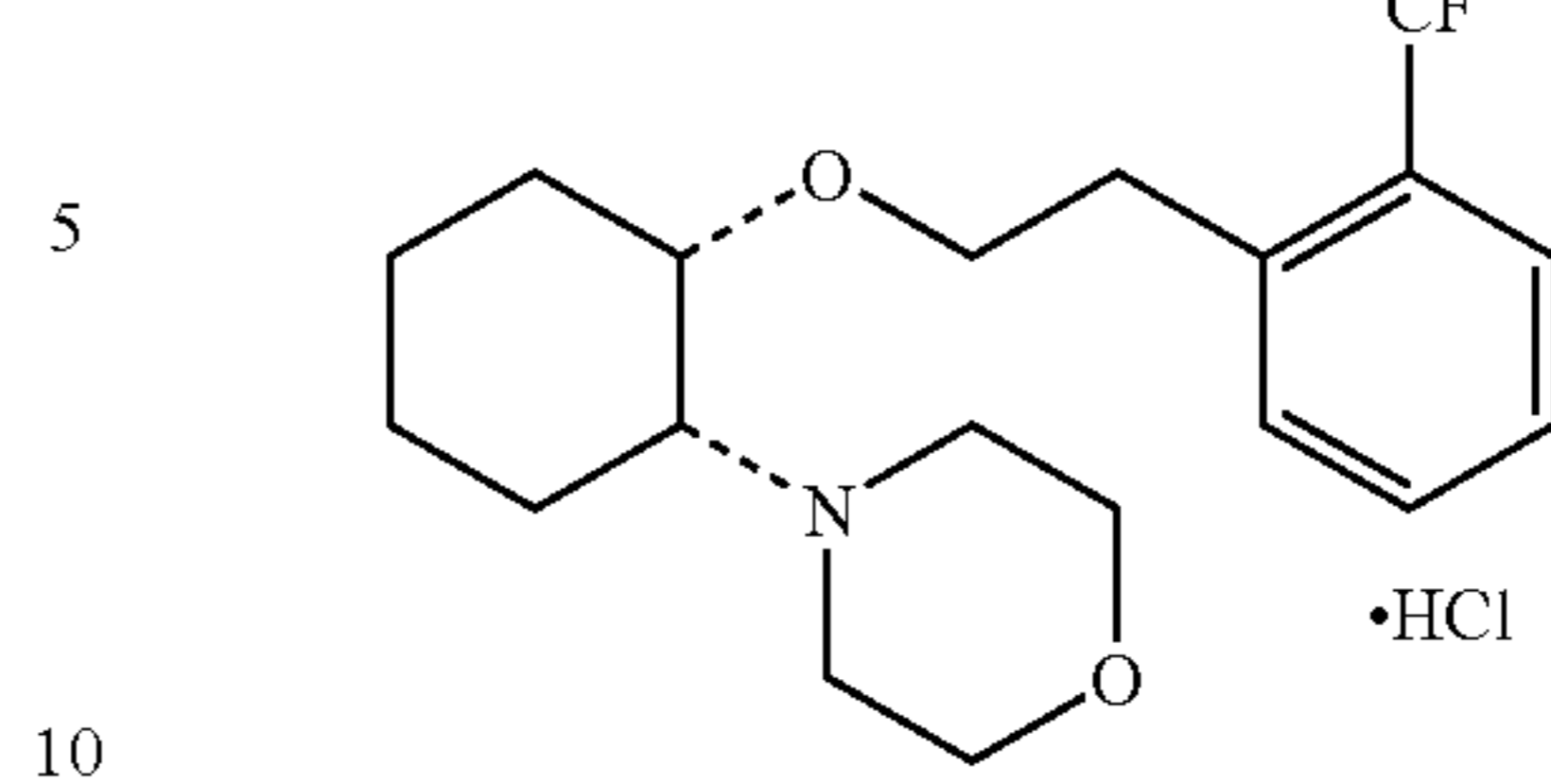
(1R,2S)/(1S,2R)-2-(4-morpholinyl)-1-[(2-trifluoromethyl)phenethoxy]cyclohexane monohydrochloride
