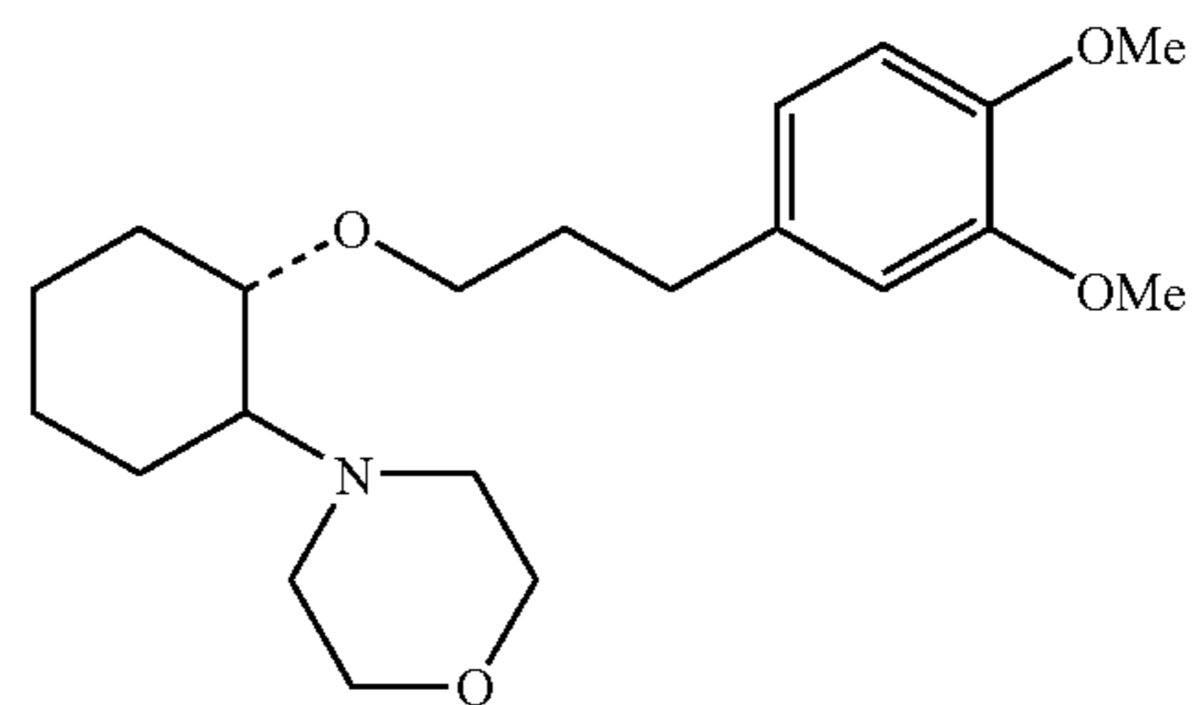
(1R,2R)/(1S,2S)-[2-(4-morpholinyl)-1-(3-(3,4-dimethoxyphenyl)propoxy)]cyclohexane
