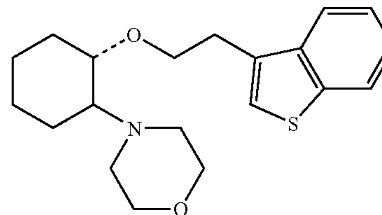
(1R,2R)/(1S,2S)-[2-(4-morpholinyl)-1-(2-benzo[b]thiophen-3-yl)]cyclohexane
