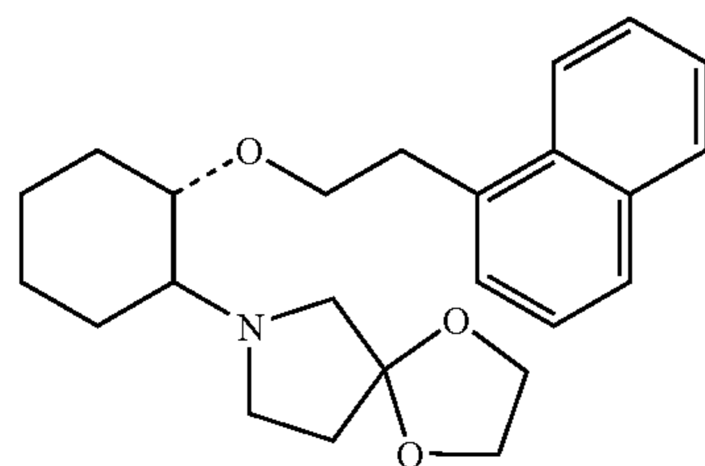
(1R,2R)/(1S,2S)-2-[1,4-dioxo-7-azaspiro[4.4]non-7-yl]-1-(1-naphthenethoxy)cyclohexane
