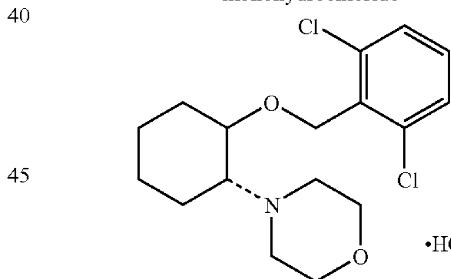
(1R,2R)/(1S,2S)-2-(4-morpholinyl)-1-[(2,6-dichlorophenyl)methoxy]cyclohexane monohydrochloride
