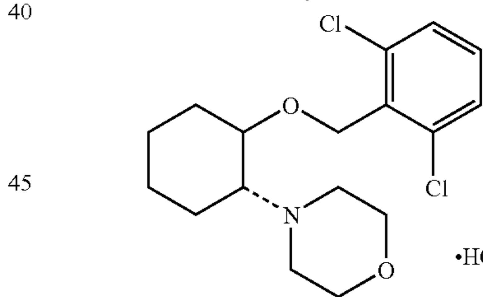
(1R,2R)/(1S,2S)-2-(4-morpholinyl)-1-[(2,6-dichlorophenyl)methoxy]cyclohexane monohydrochloride
