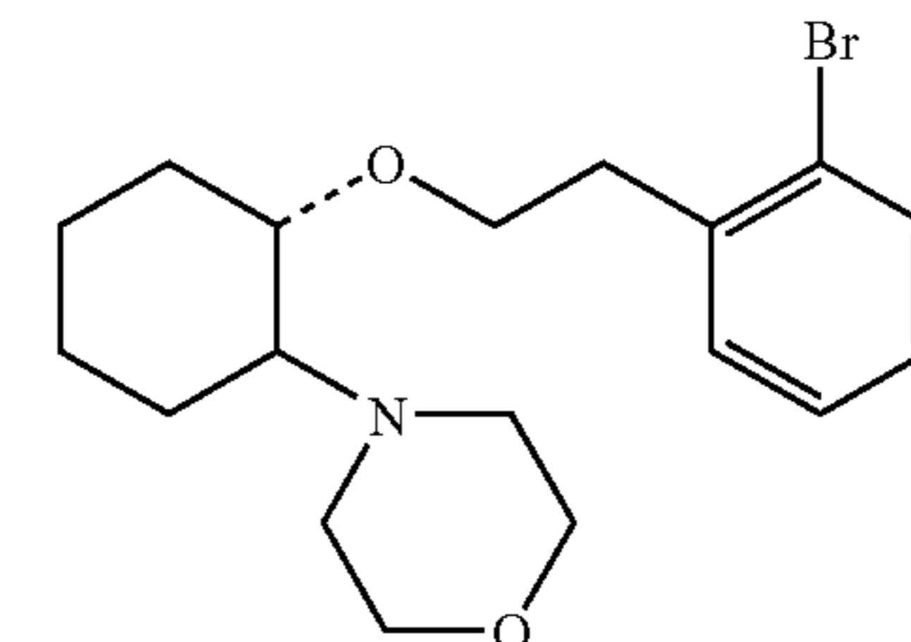
(1R,2R)/(1S,2S)-[2-(4-morpholinyl)-1-(2-bromophenethoxy)]cyclohexane
