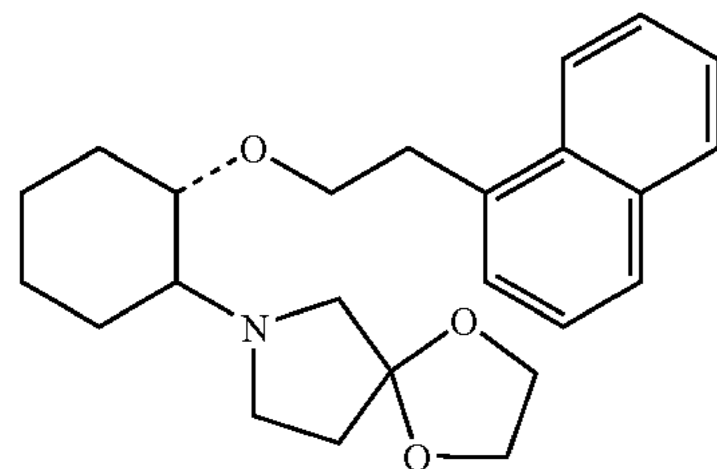
(1R,2R)/(1S,2S)-2-[1,4-dioxo-7-azaspiro[4.4]non-7-yl]-1-(1-naphthenethoxy)cyclohexane
