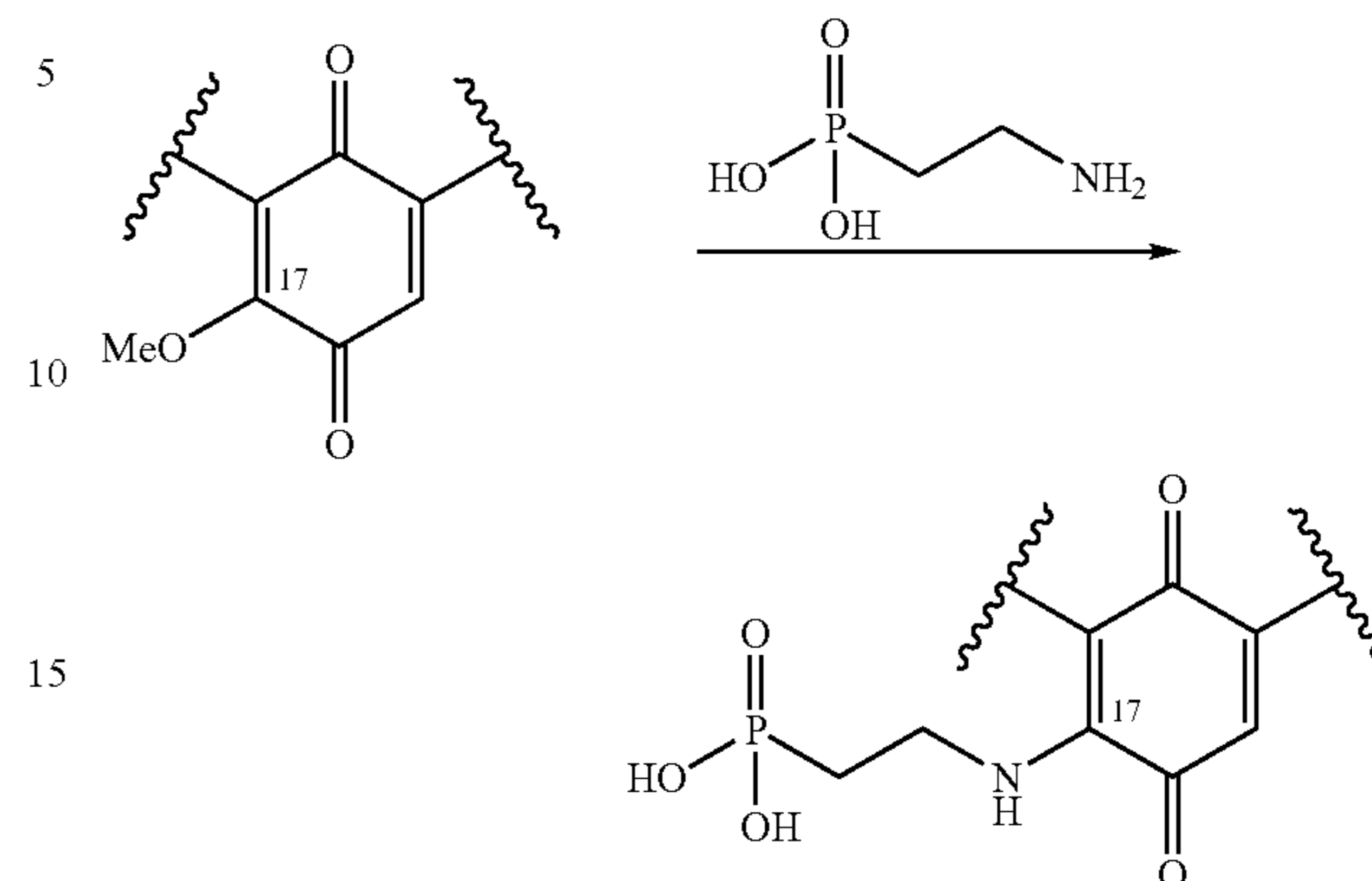
Scheme 4
