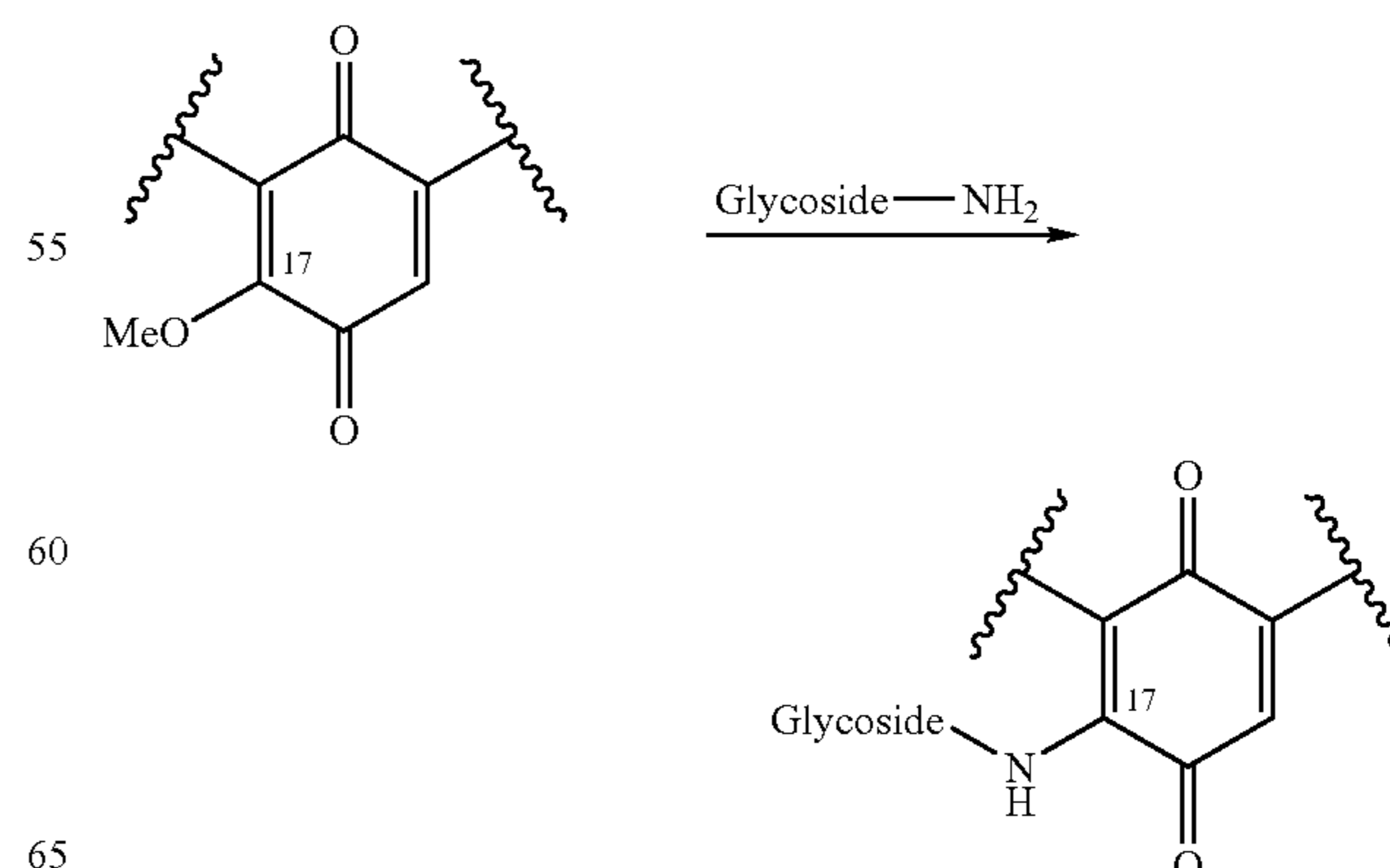
Scheme 5
