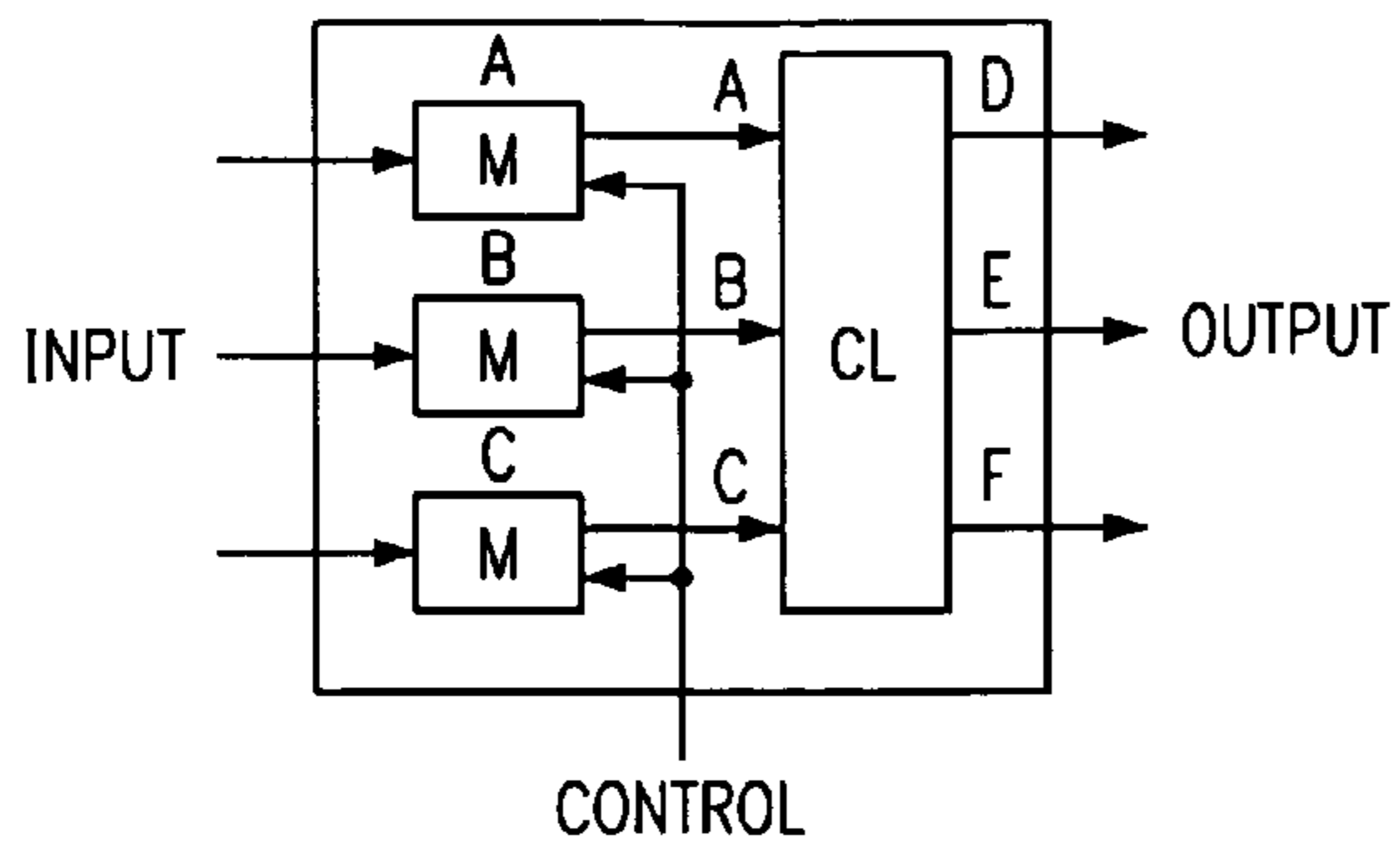
FIG. 1 (PRIOR ART)
