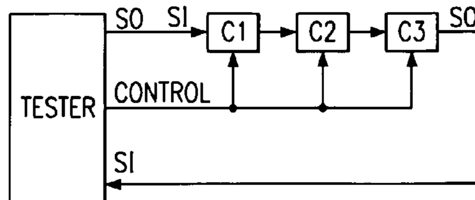
FIG. 5 (PRIOR ART)
