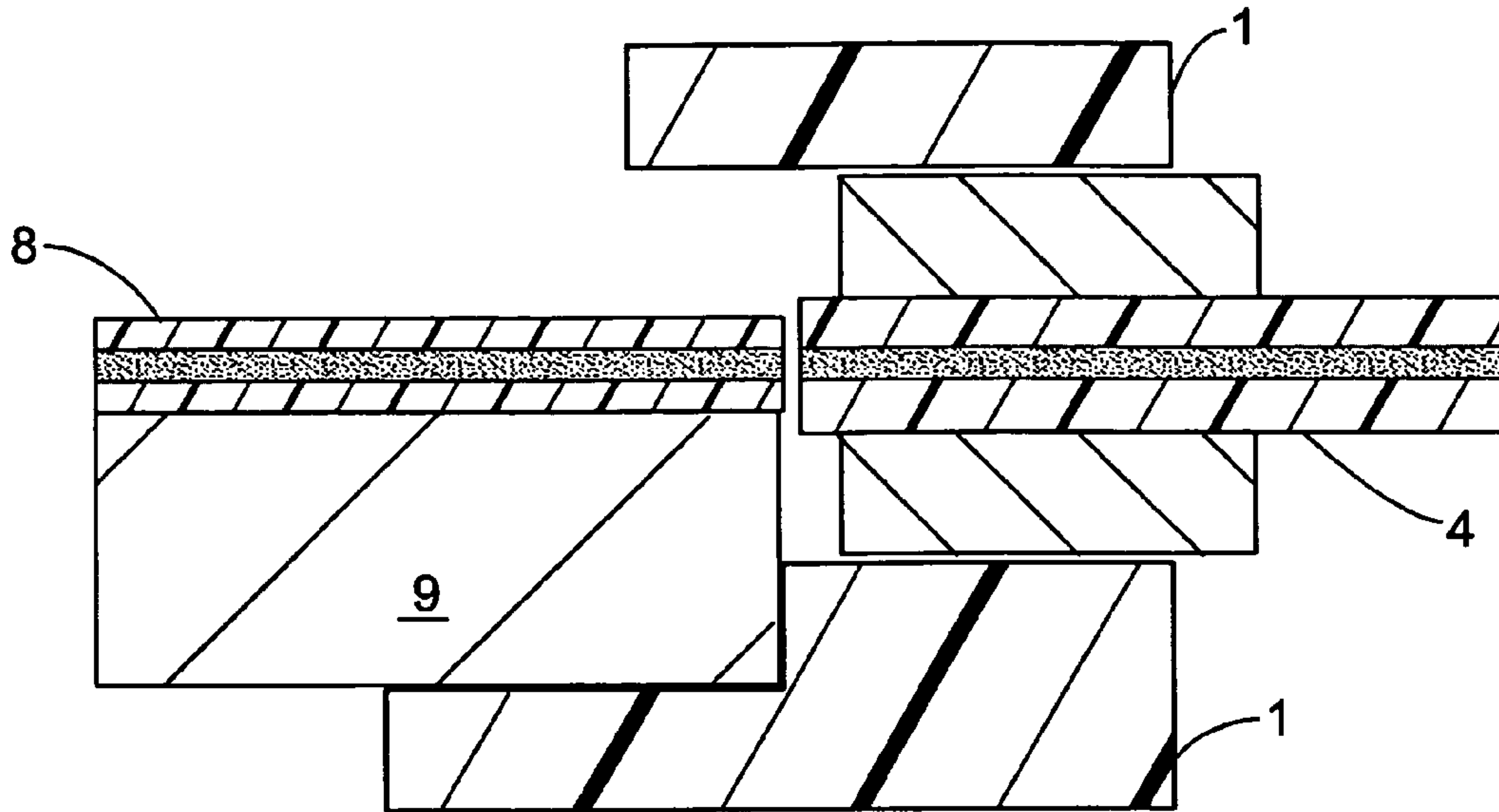
FIG. 1 (PRIOR ART)
