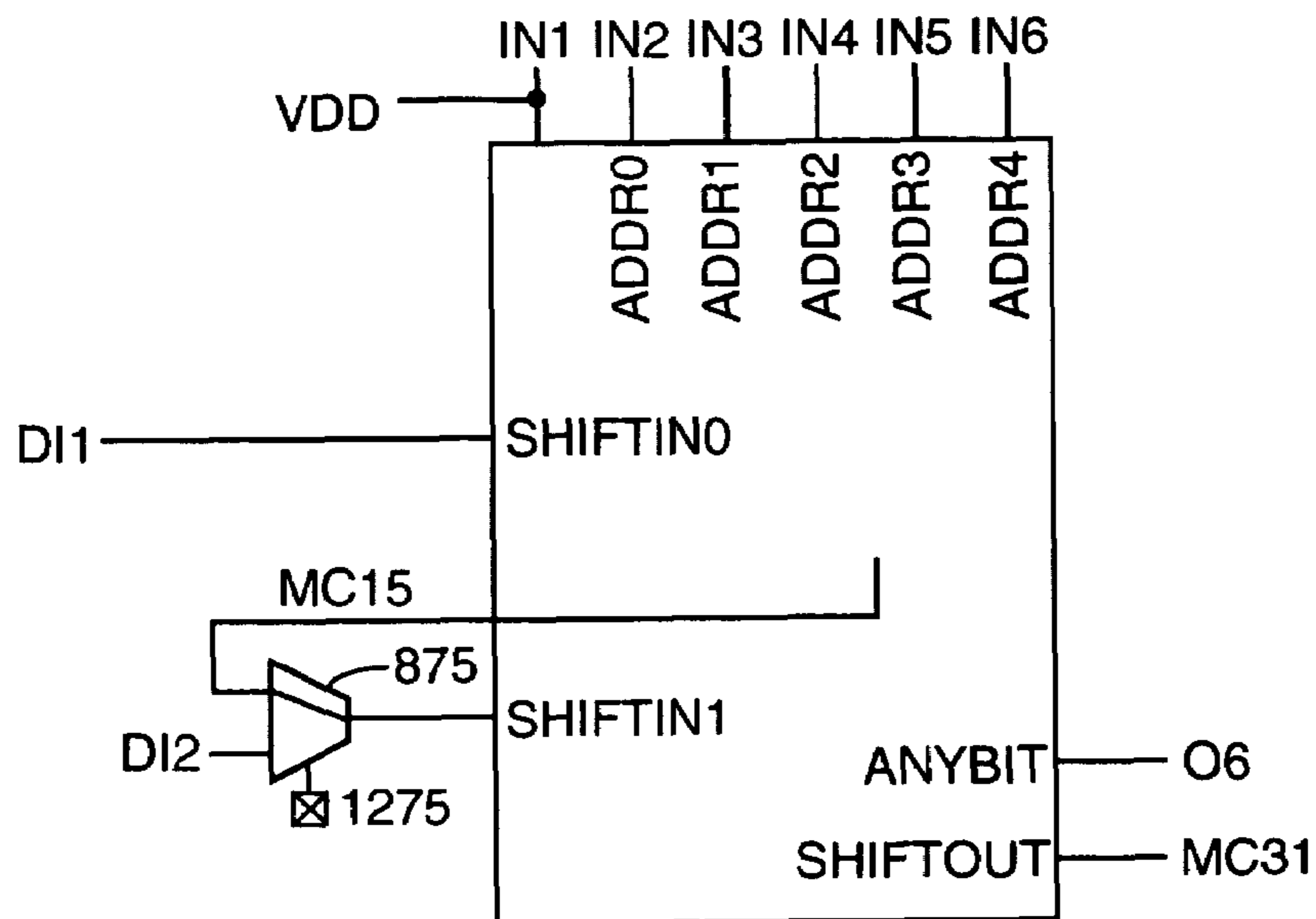
FIG. 12 (32x1 SRL)
