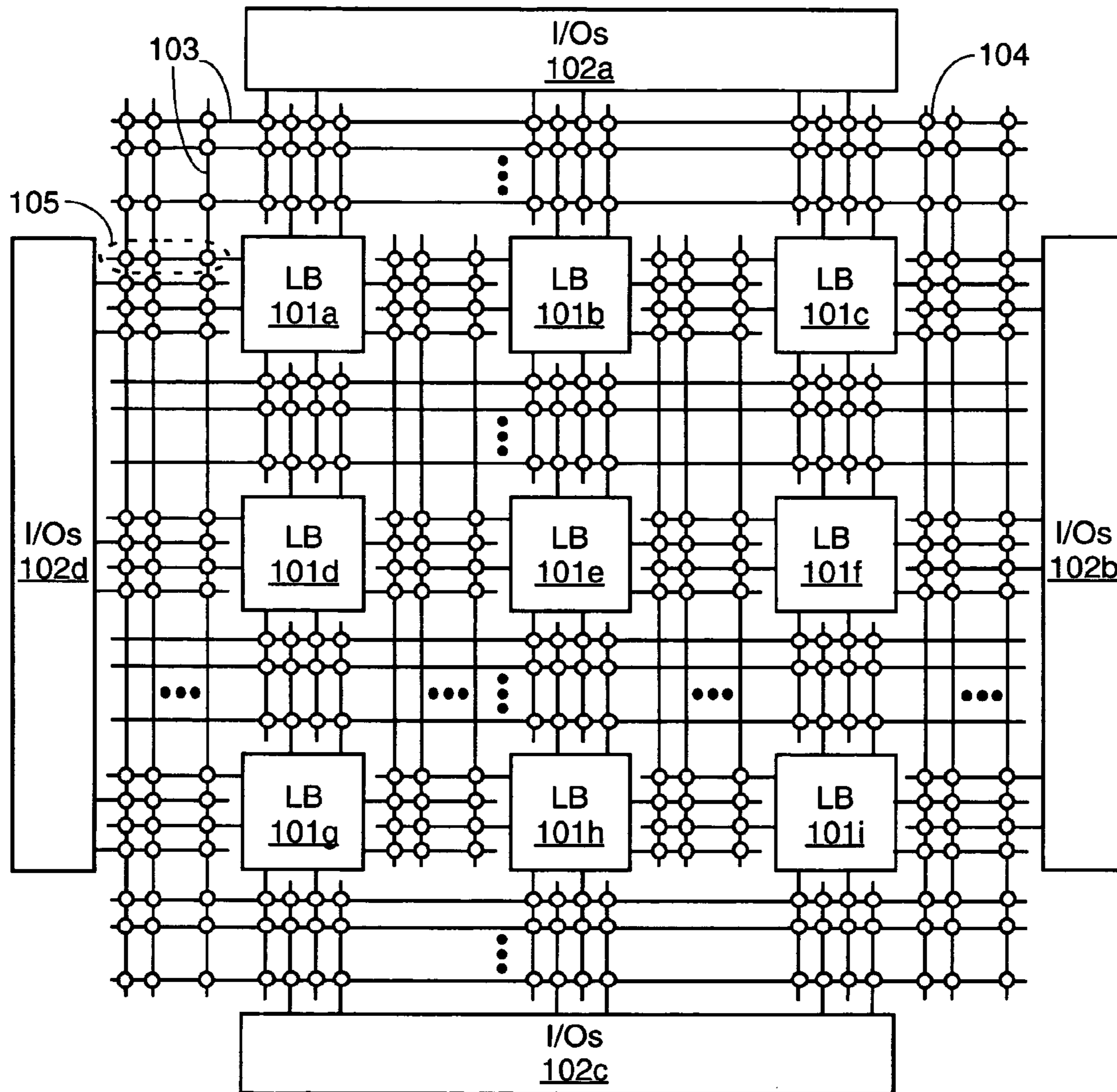
FIG. 1 (Prior Art)
