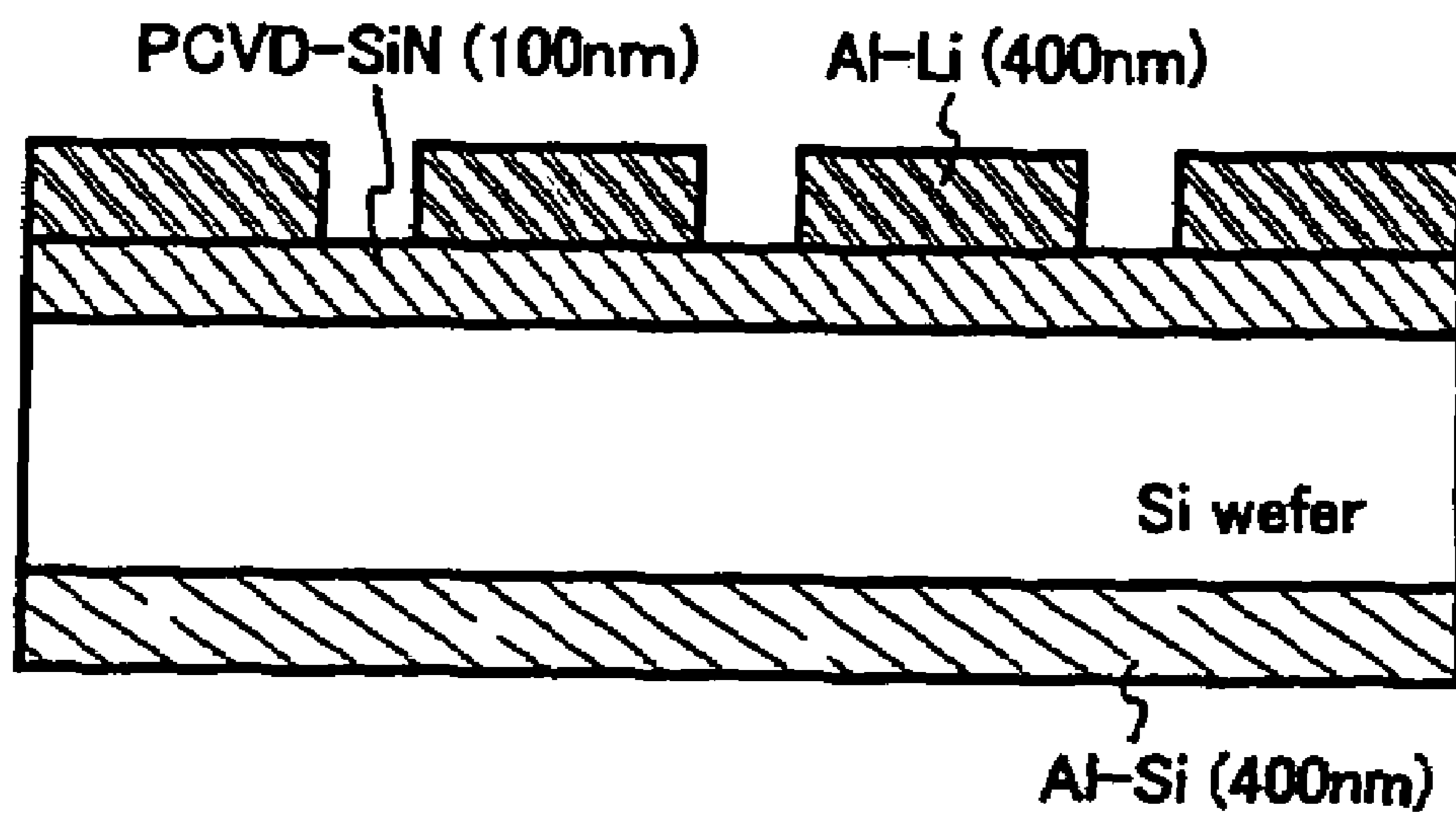
(A) MOS structure using PCVD-SiN film
