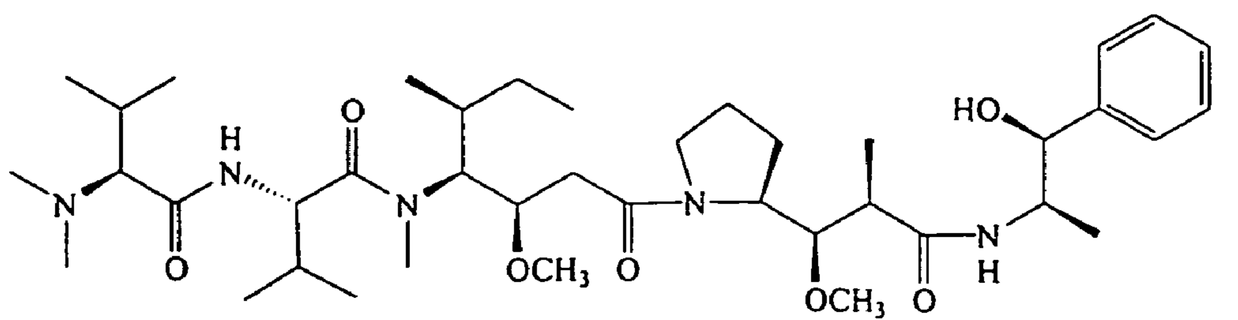
(29a, auristatin E)
