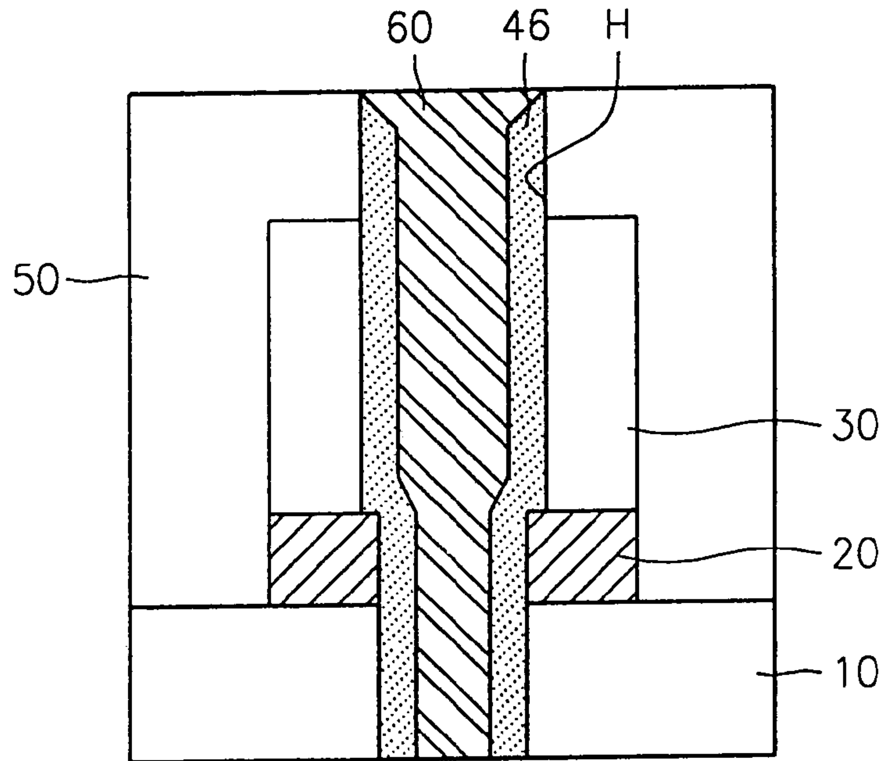
FIG. 3 (PRIOR ART)
