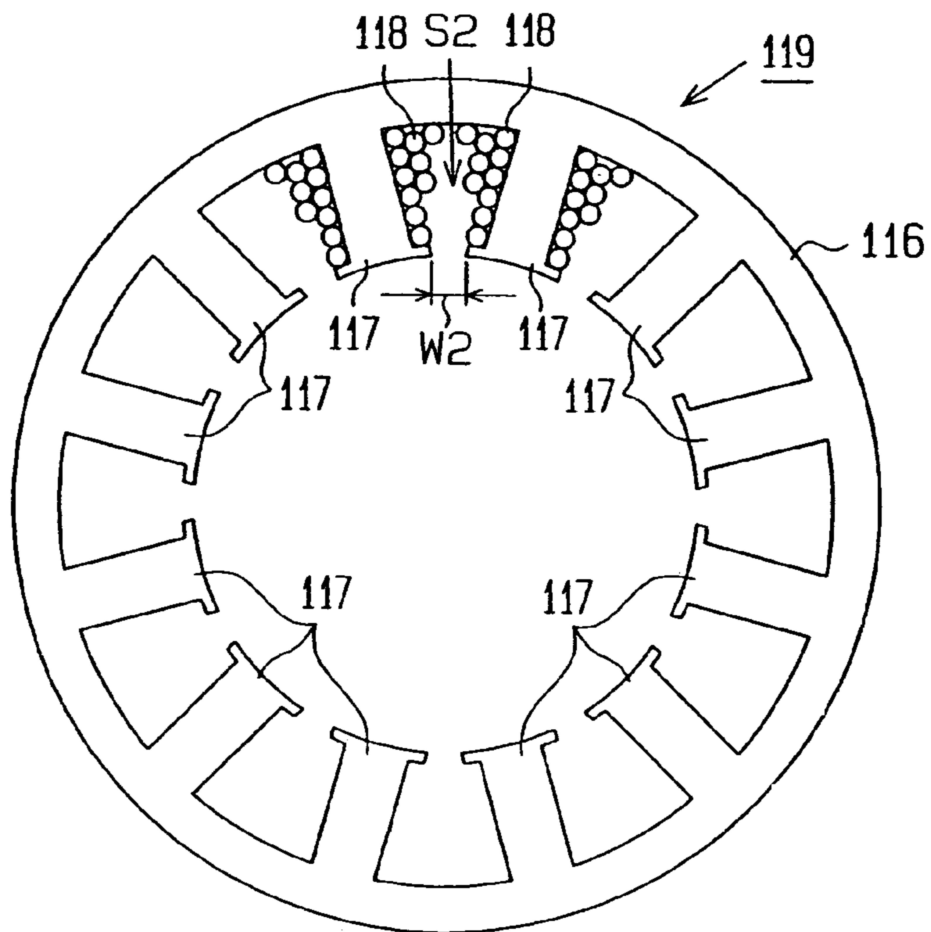
Fig. 69 (Prior Art)
