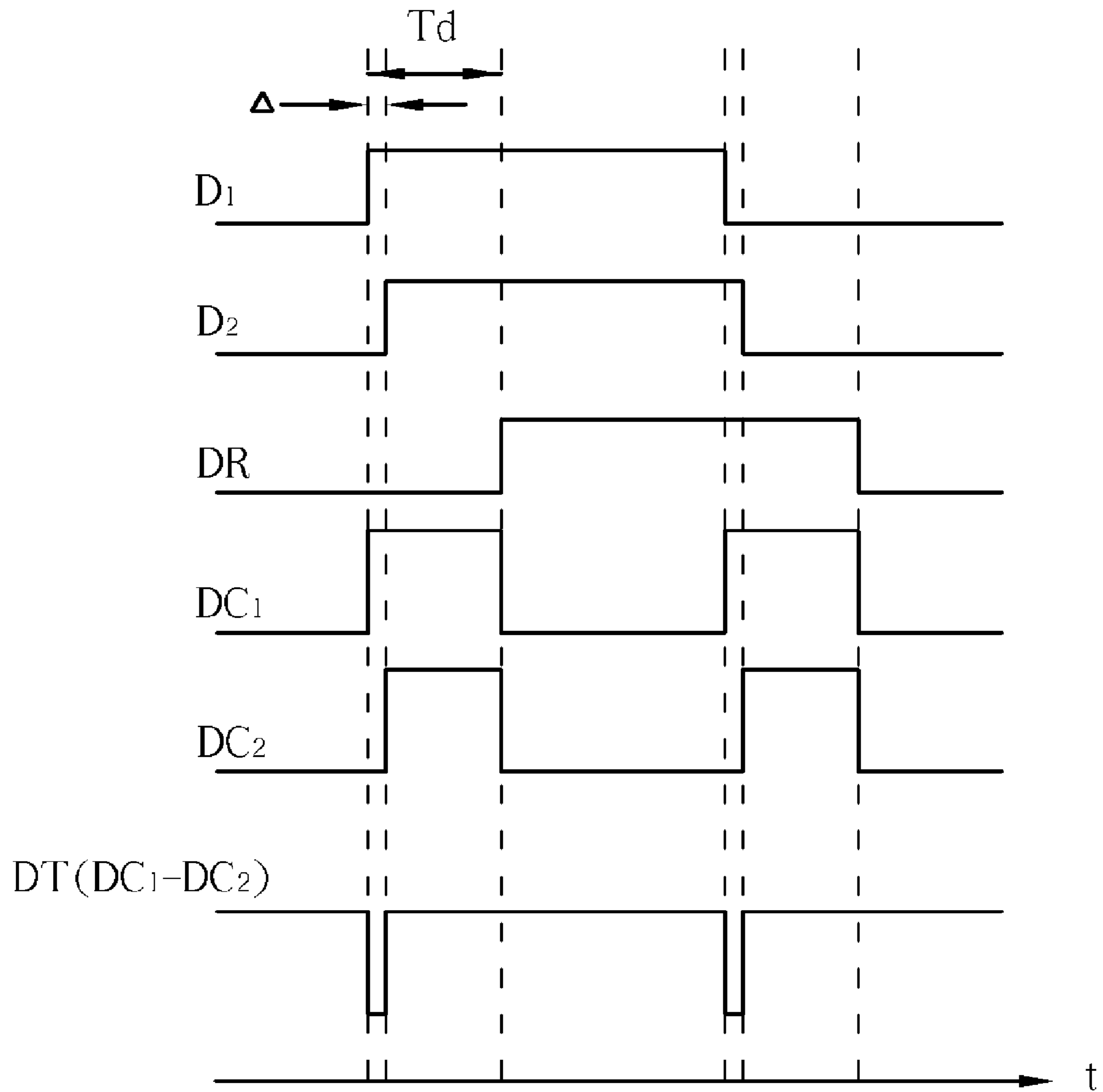
Fig. 4 Prior Art
