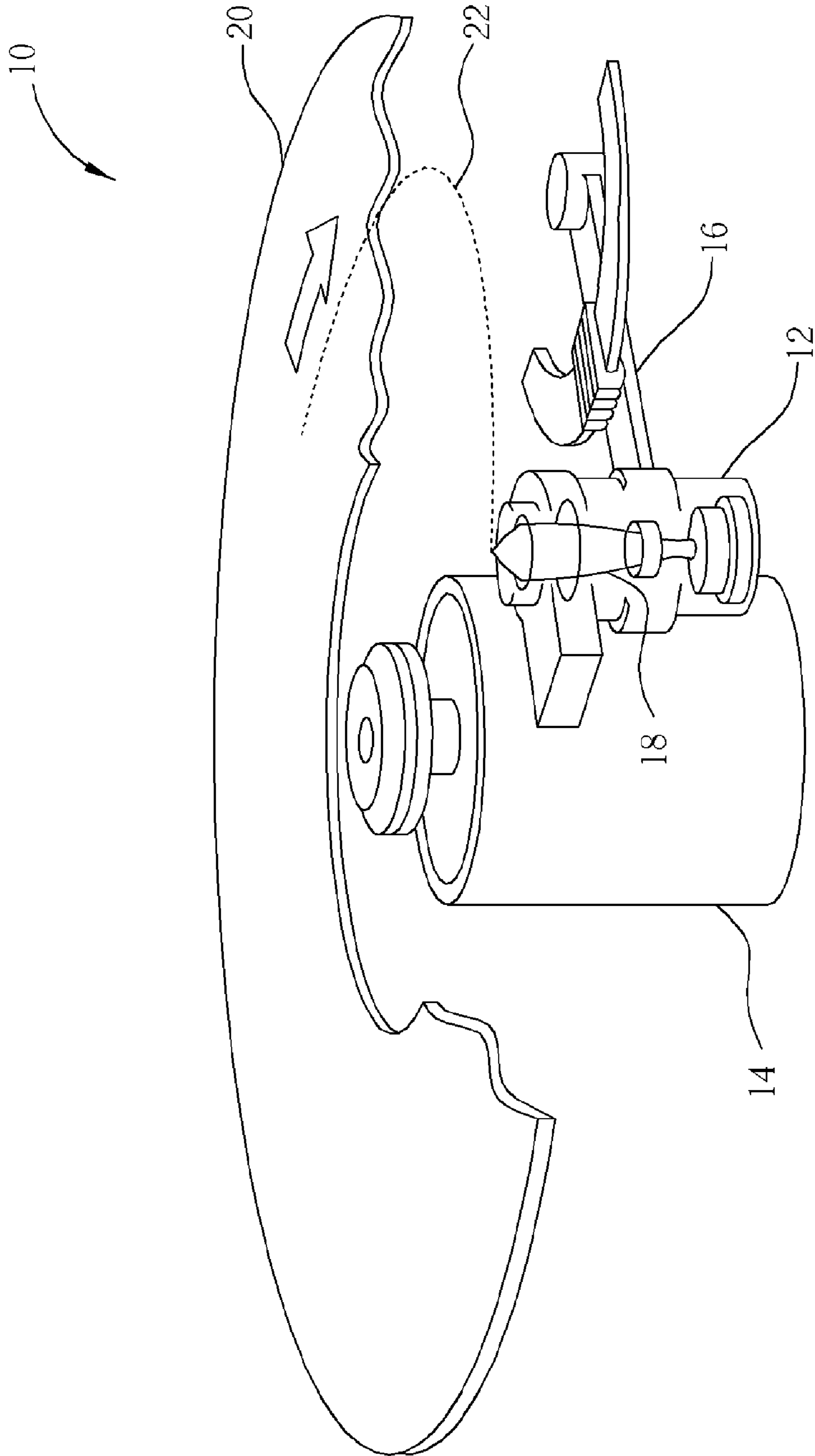
Fig. 1 Prior Art
