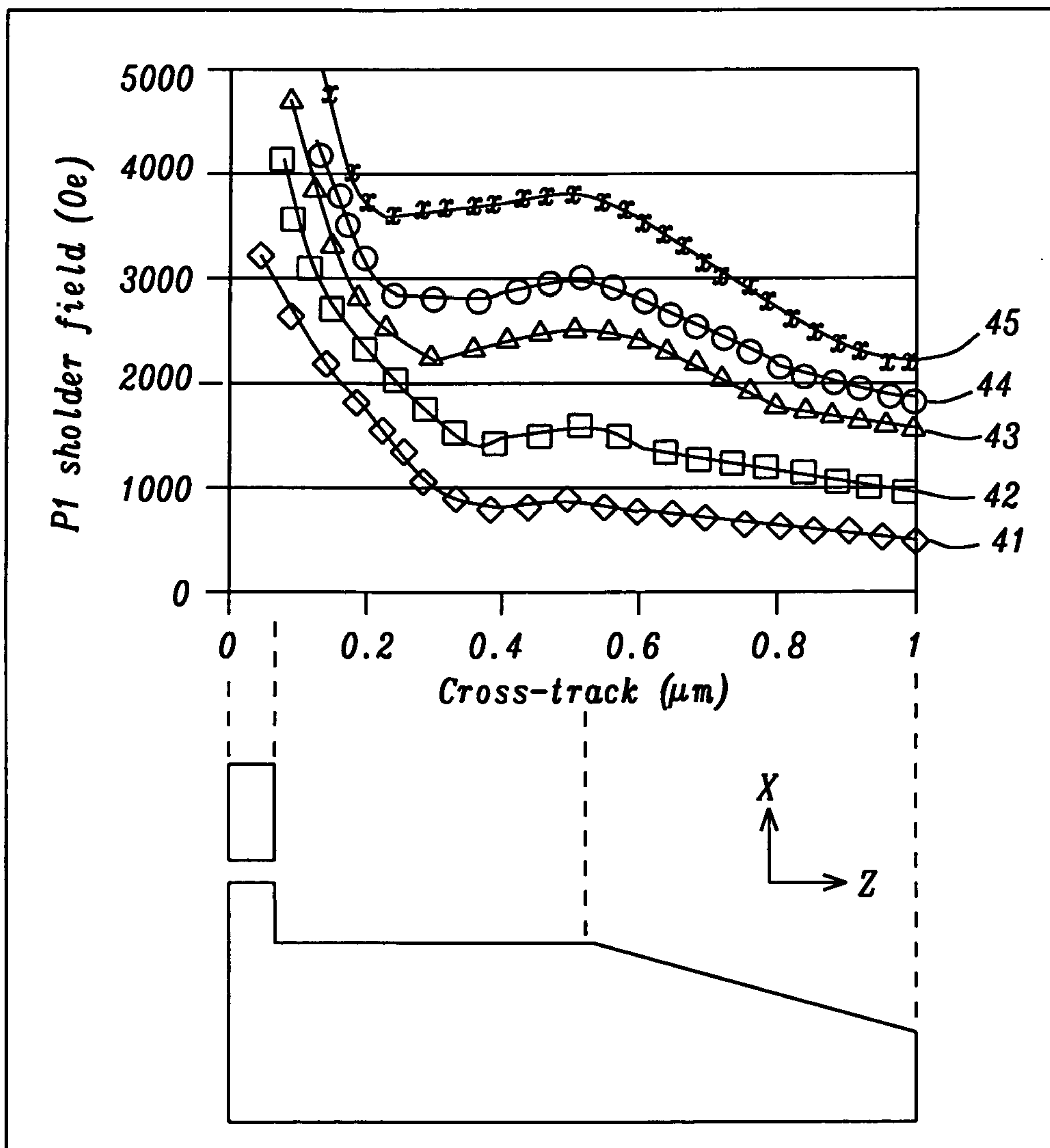
FIG. 4 - Prior Art
