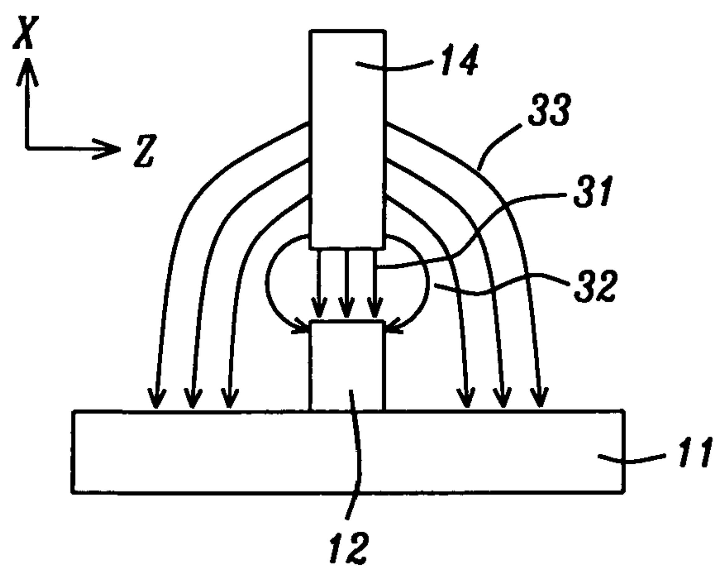
FIG. 3 - Prior Art
