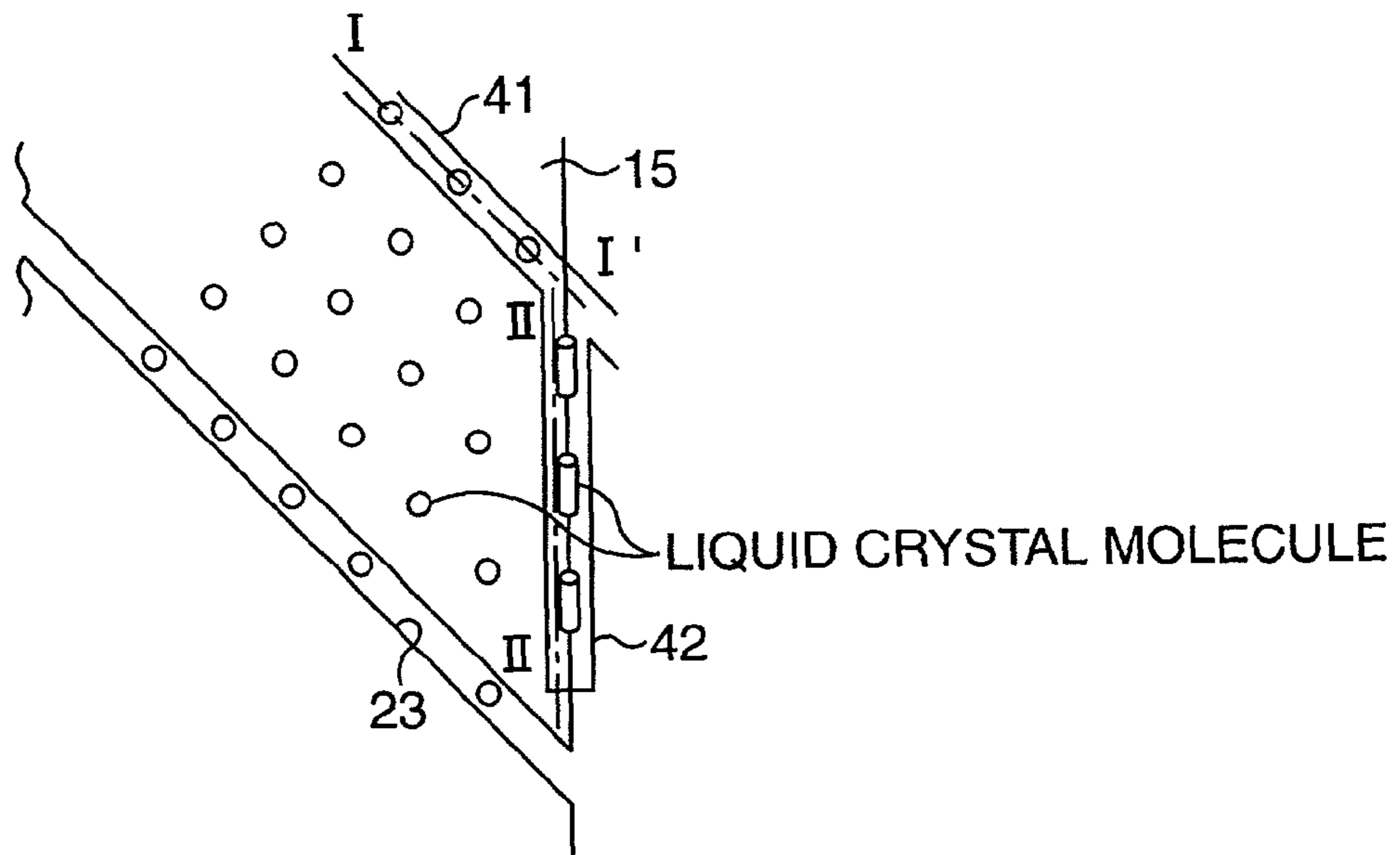
PLANE VIEW
