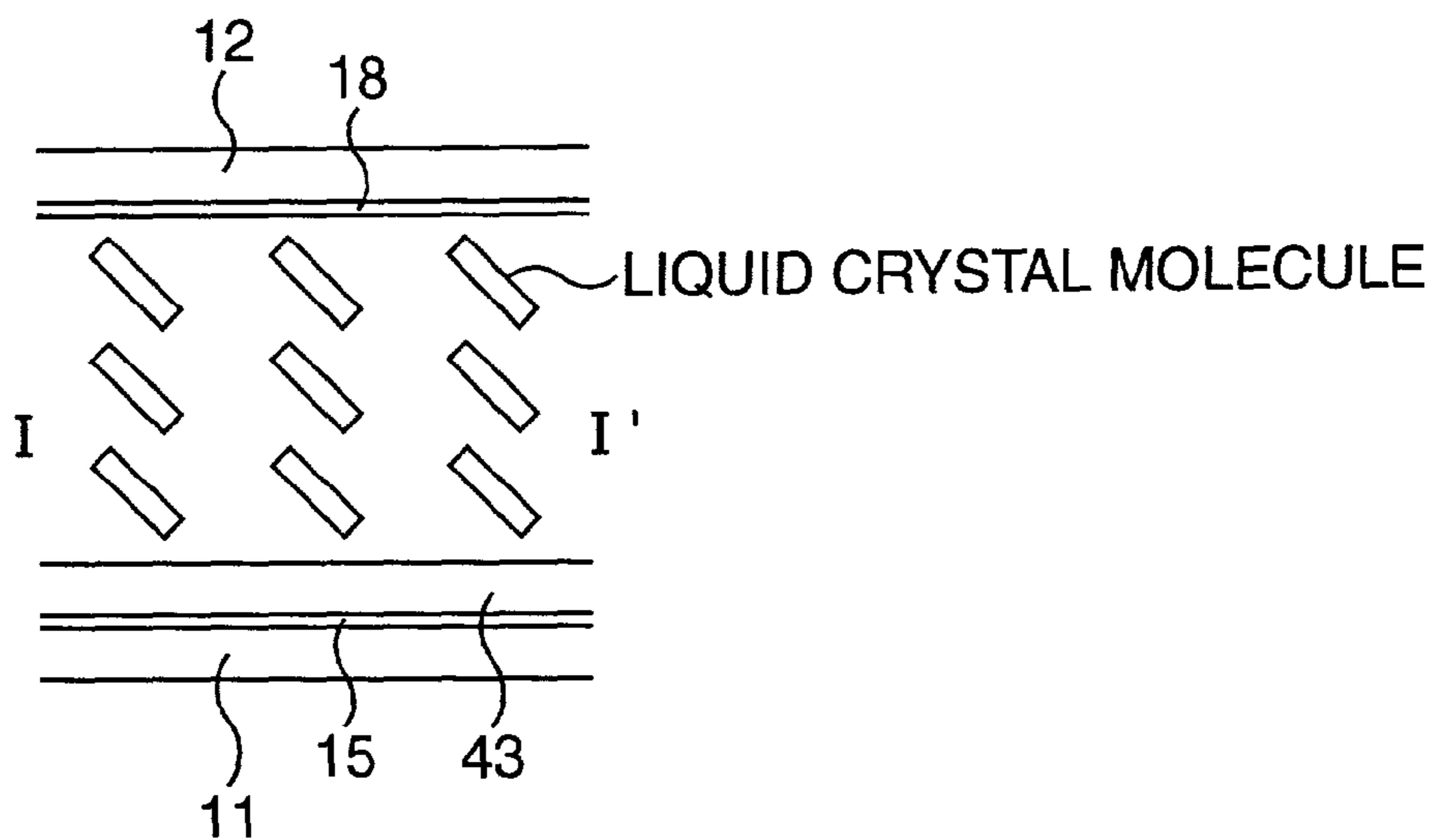
SECTIONAL VIEW
