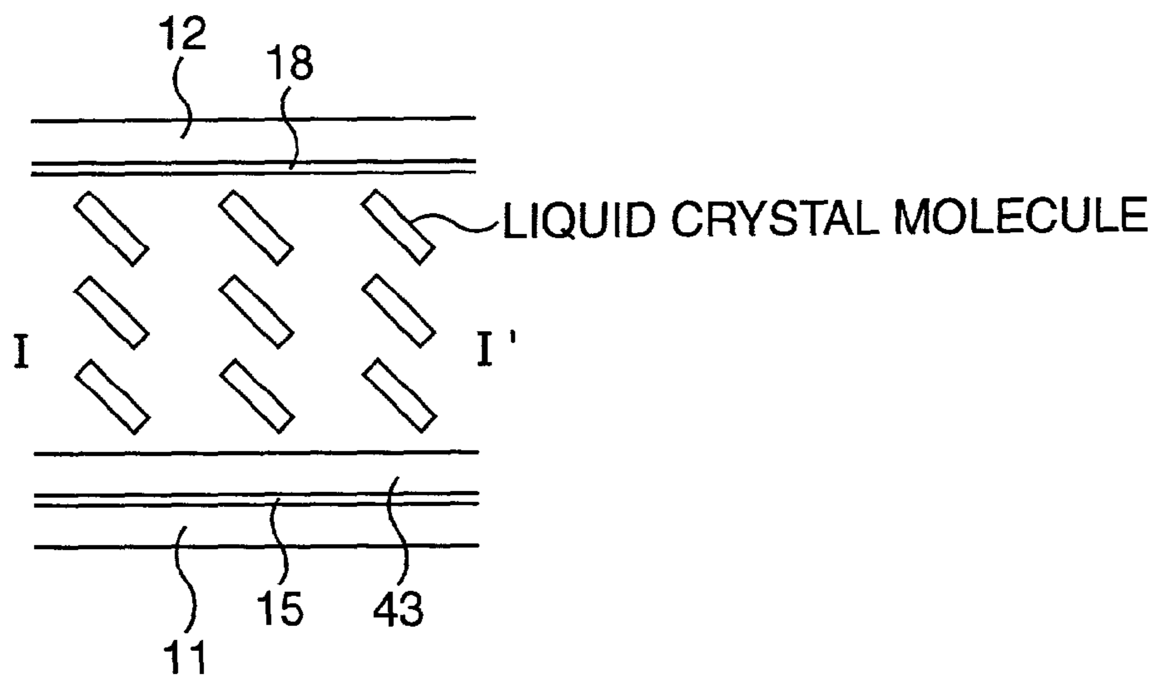
SECTIONAL VIEW
