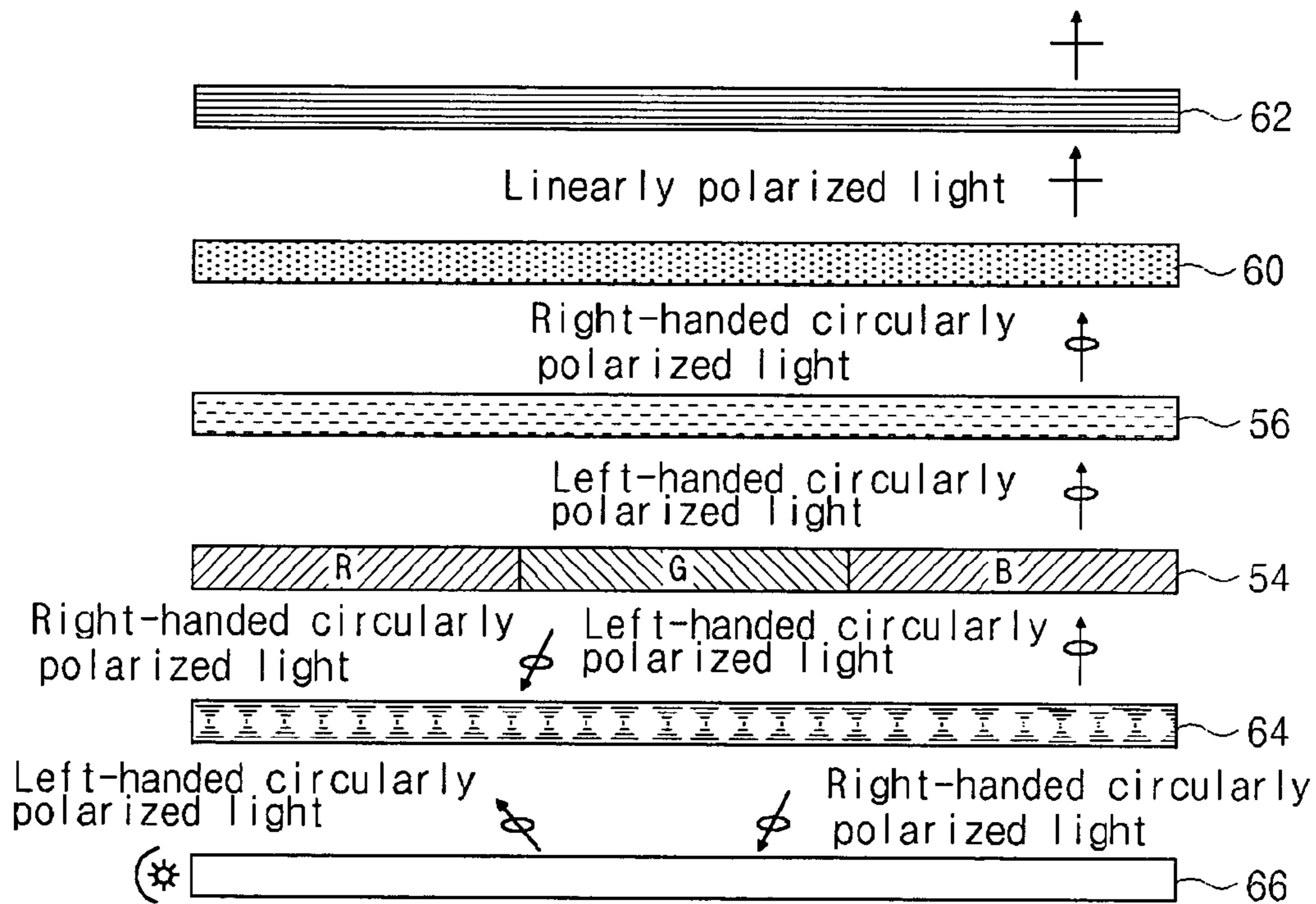
(related art) FIG. 3
