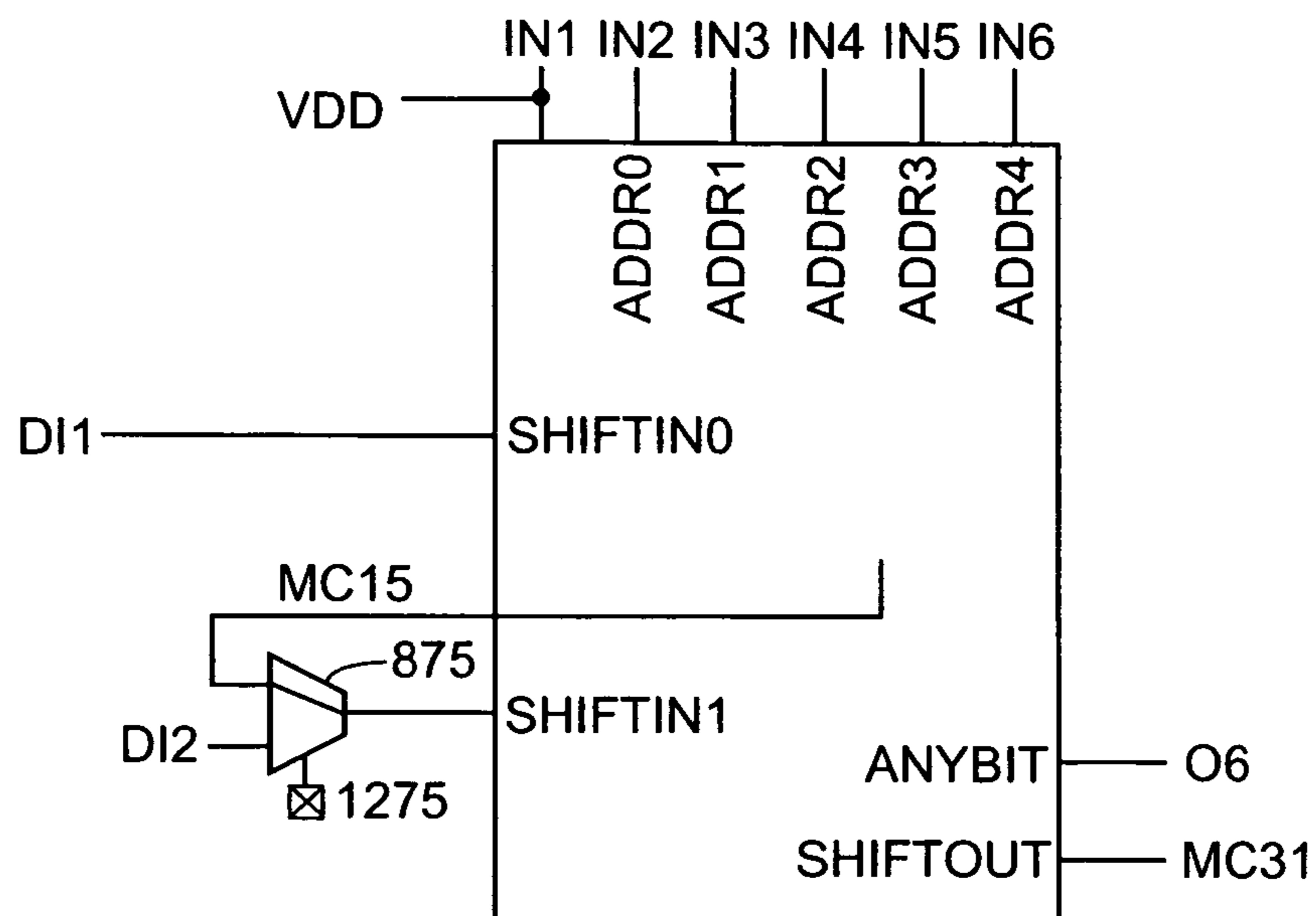
FIG. 12 (32x1 SRL)
