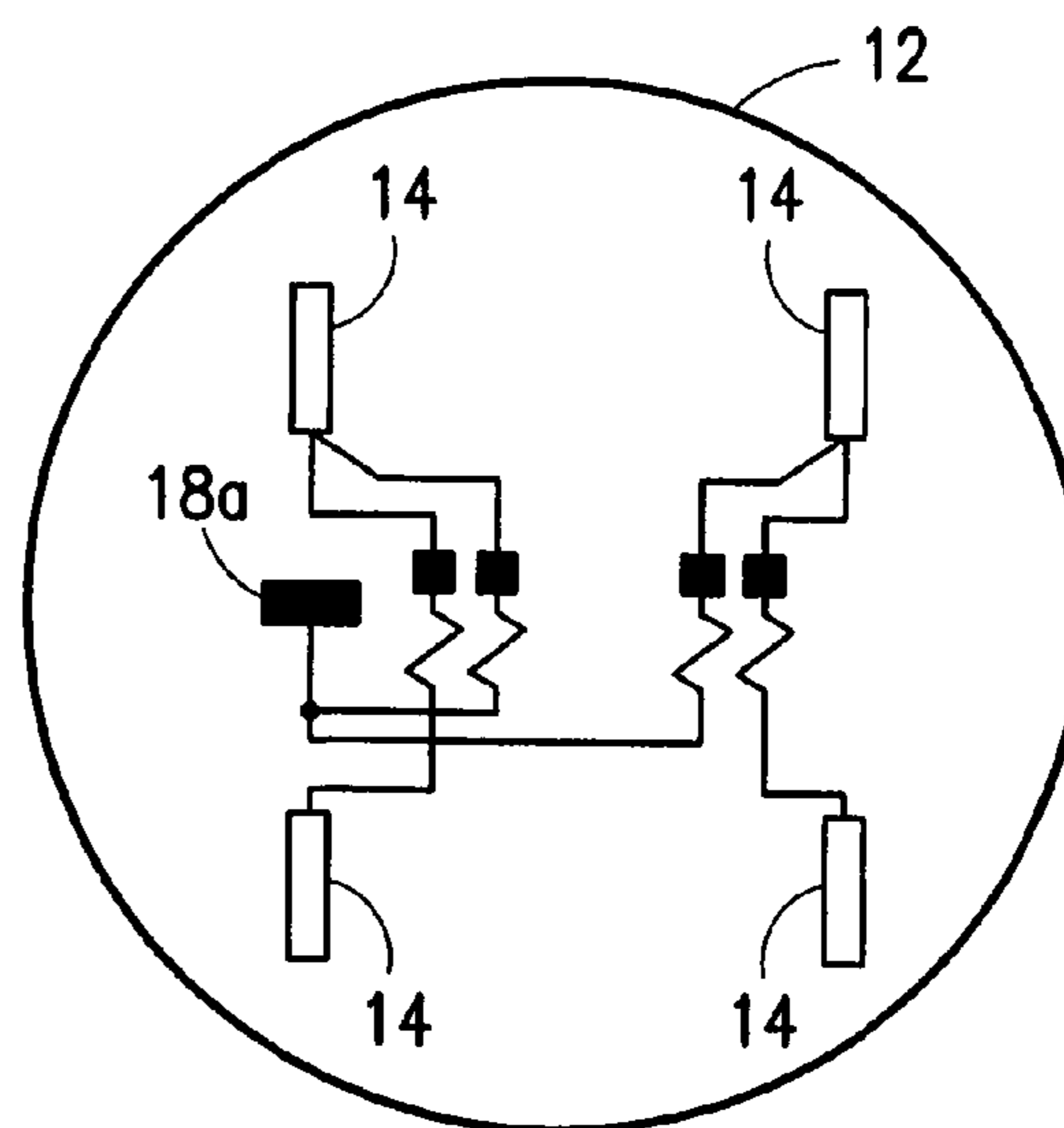
2-Element 3 - Wire FORM 25S FIG. 1b
