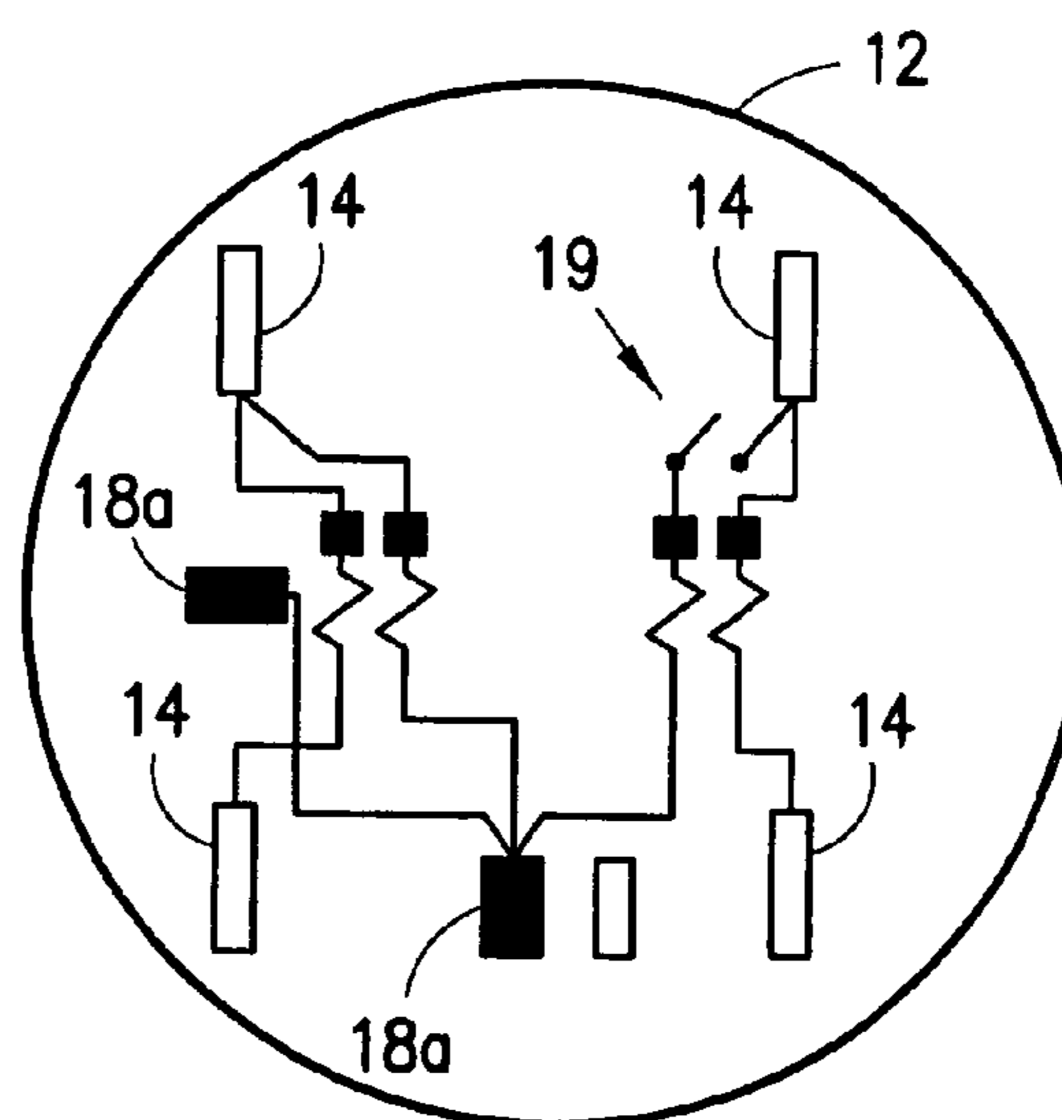
2-Element 3 - Wire FORM 12S FIG. 1d
