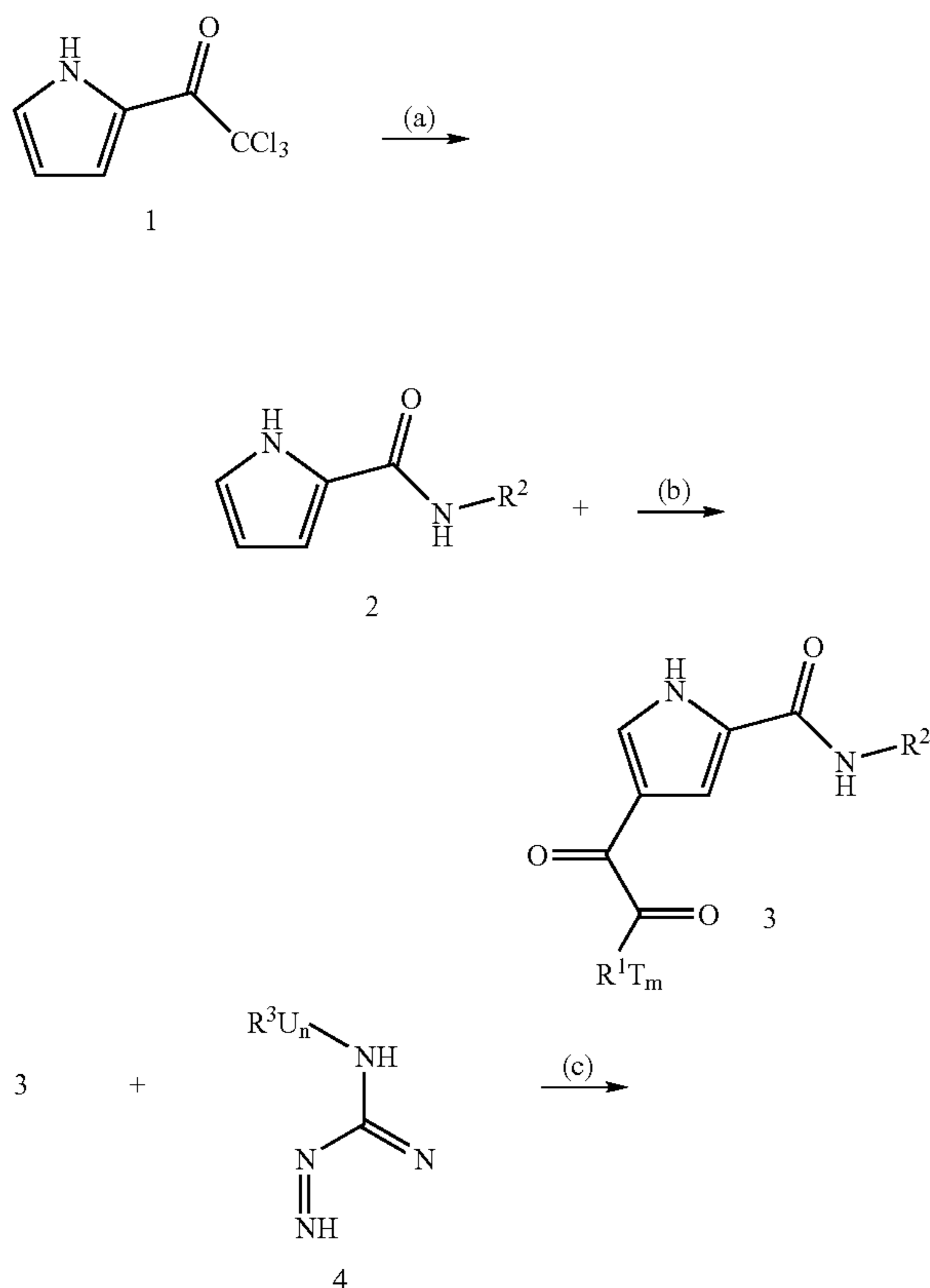
Scheme XI
