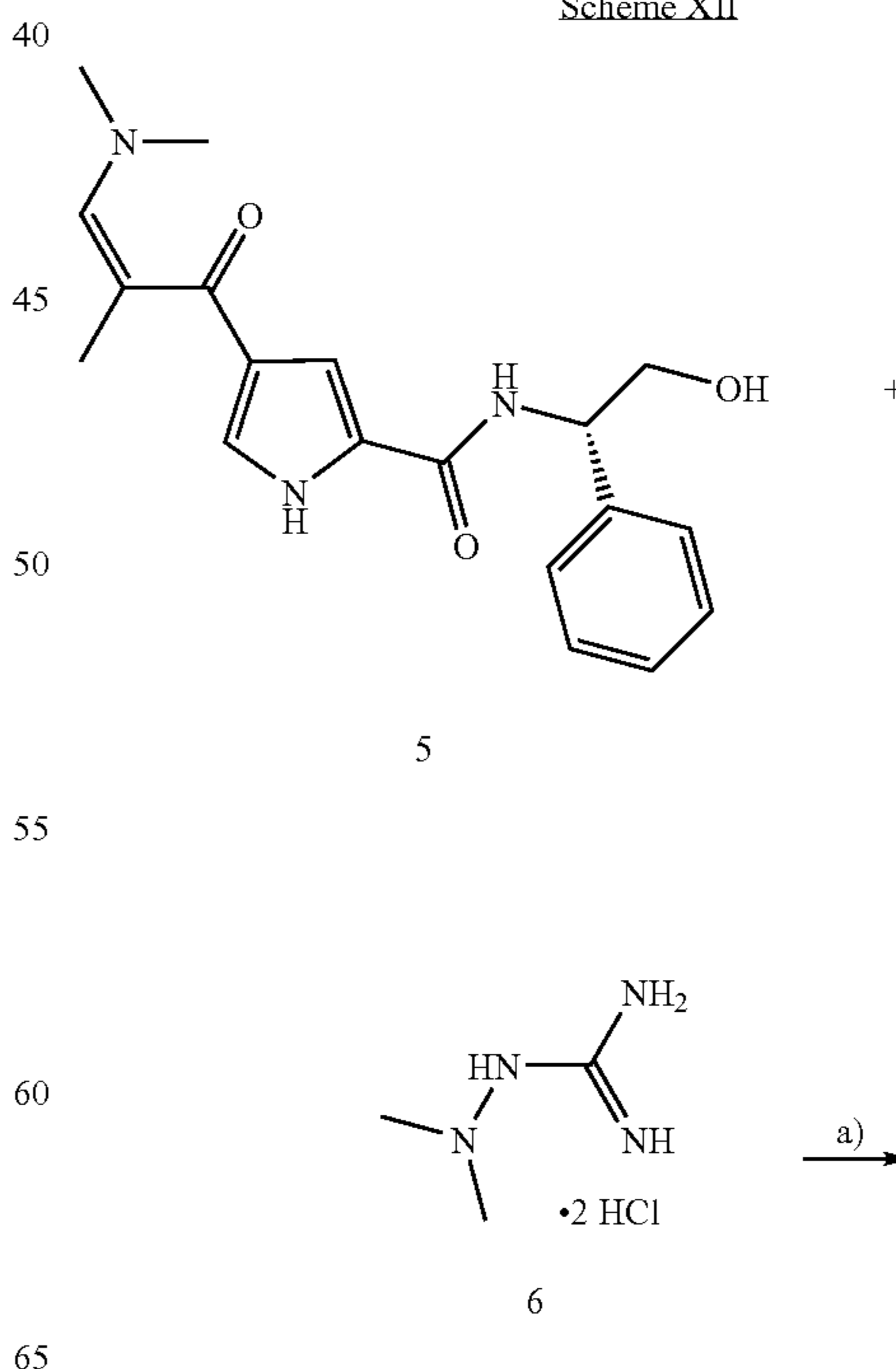
Scheme XII
