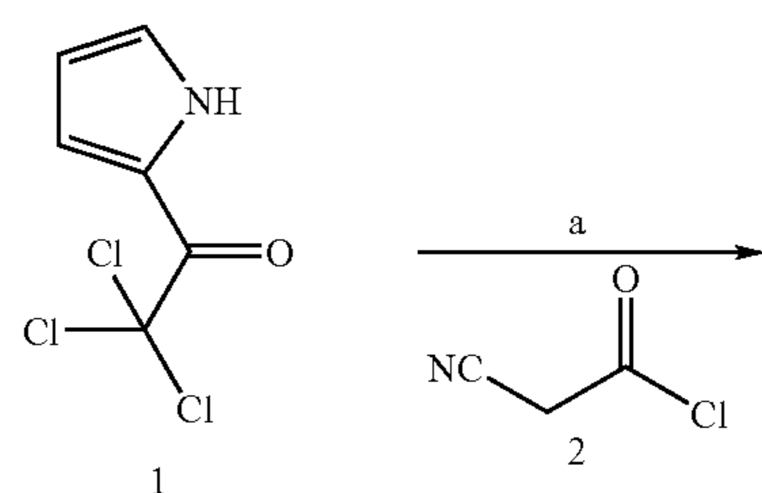
Scheme III
