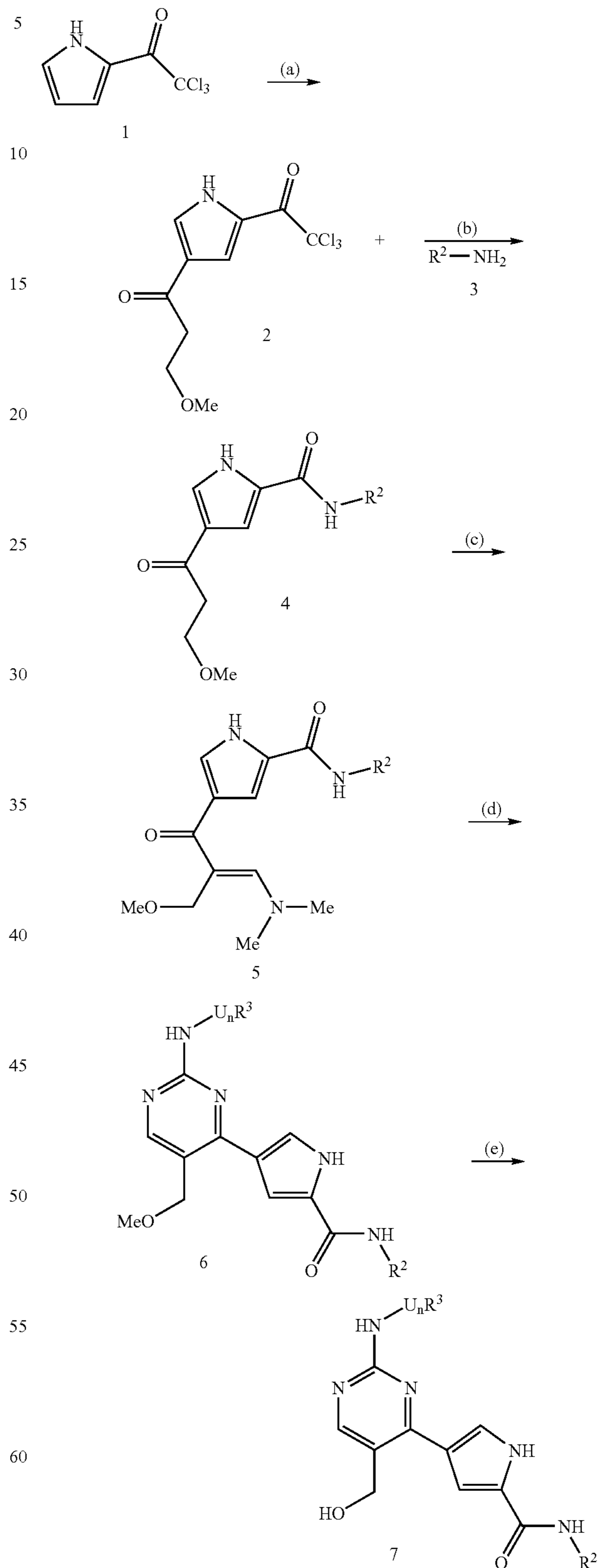
Scheme X
