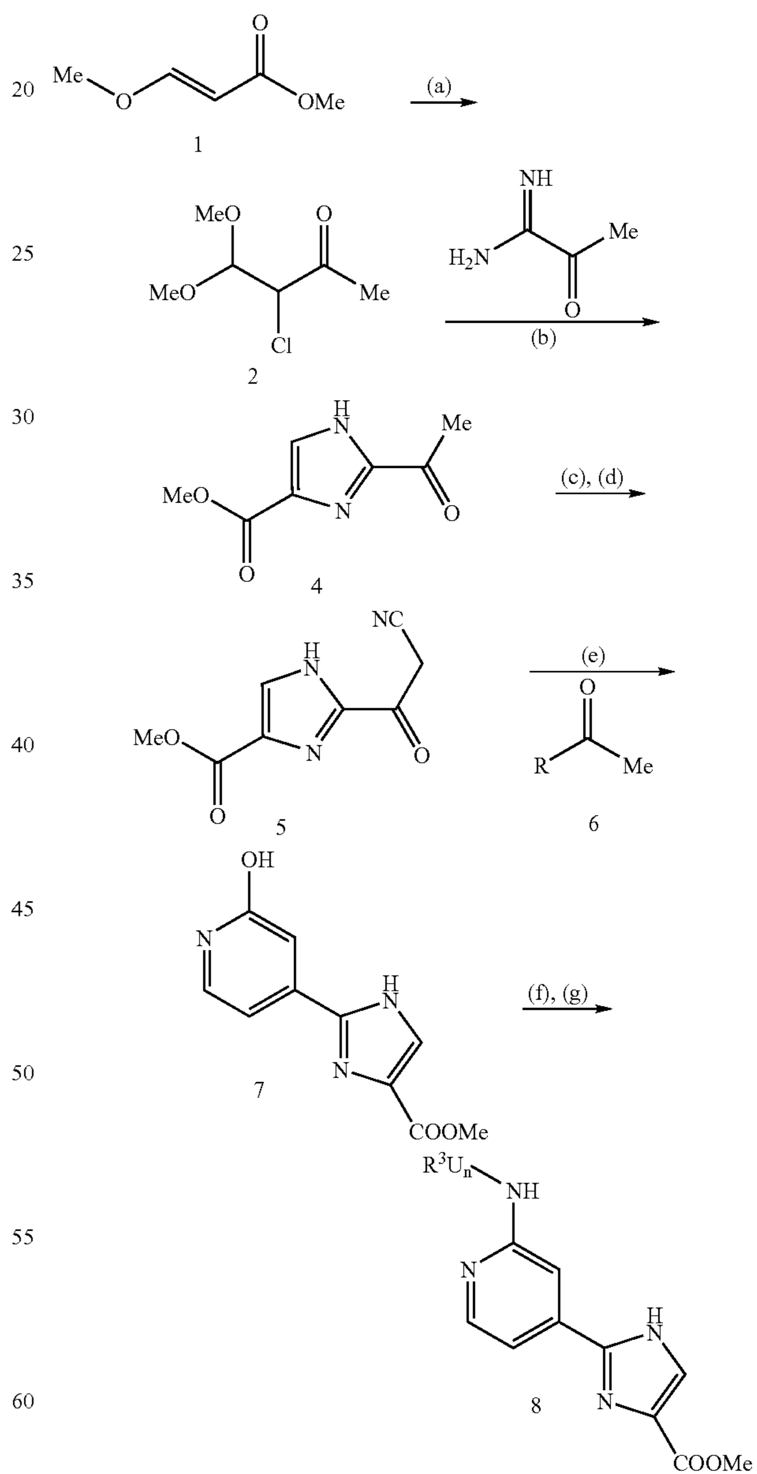
Scheme V
