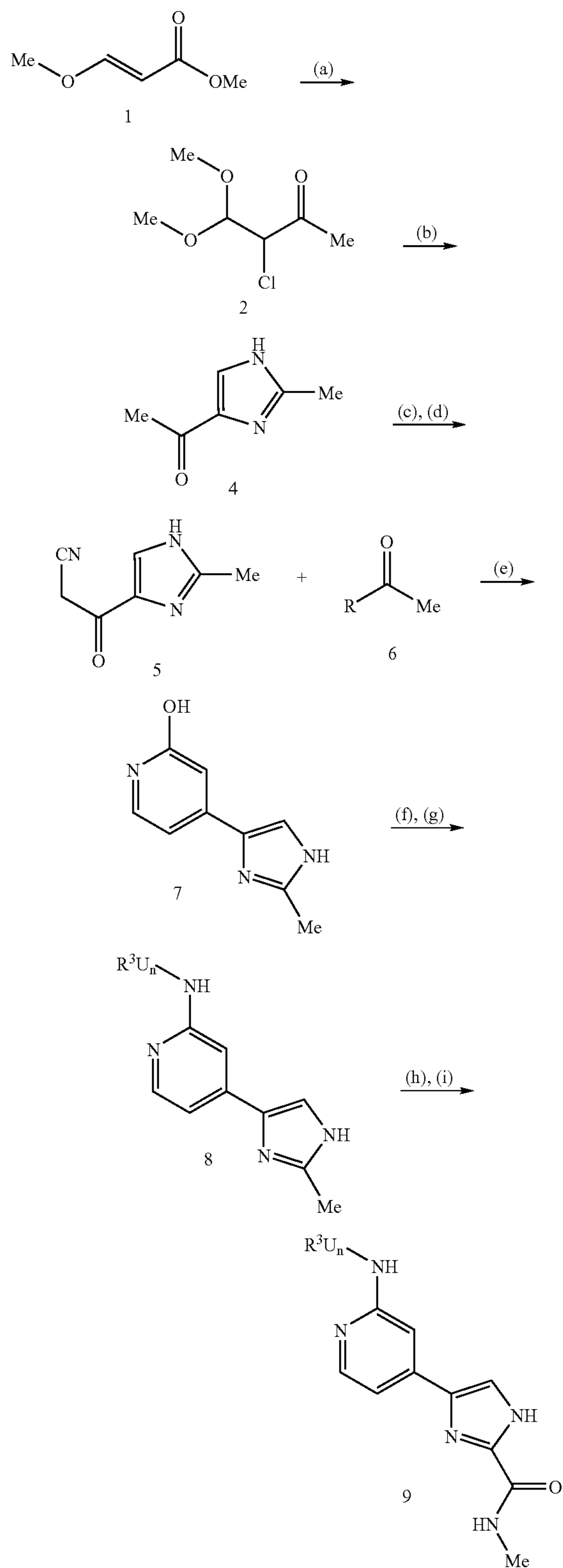
Scheme IV
