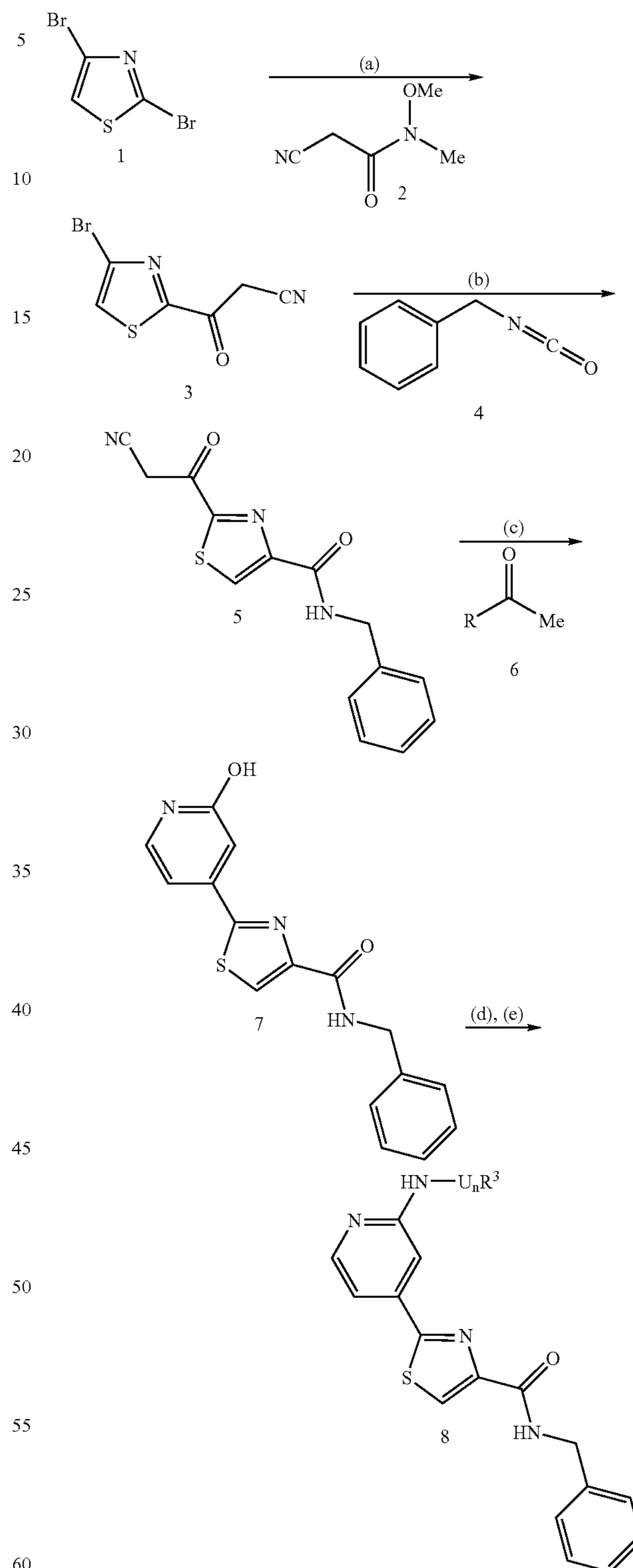
Scheme VIII
