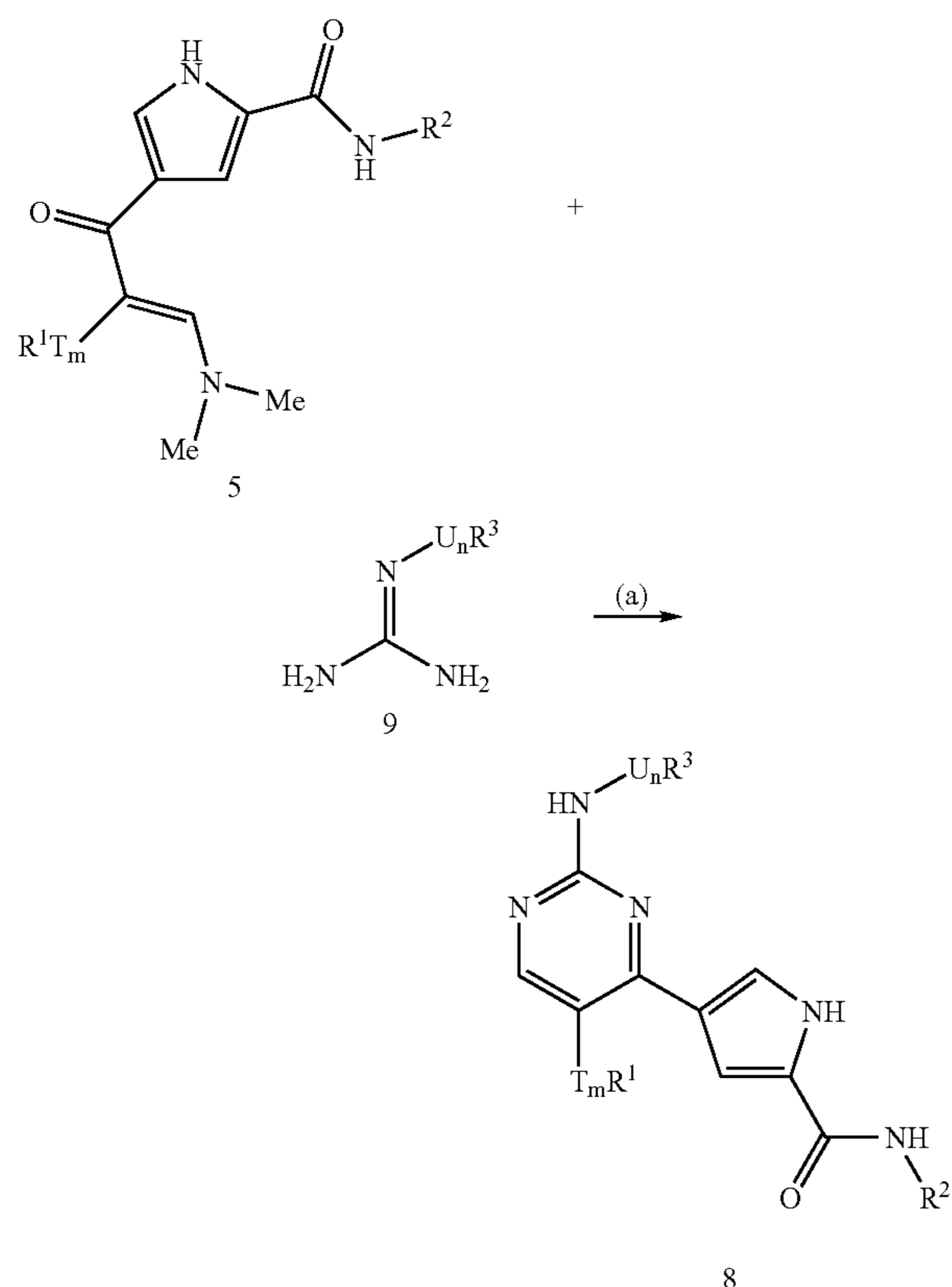
Scheme II
