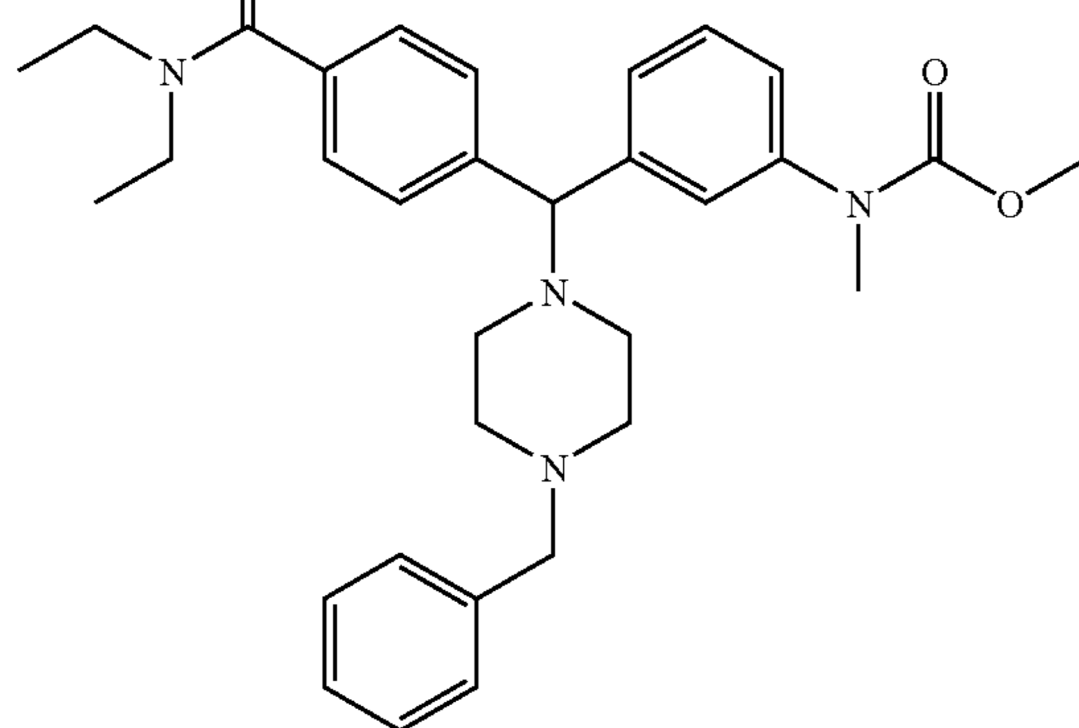
Compound 17
