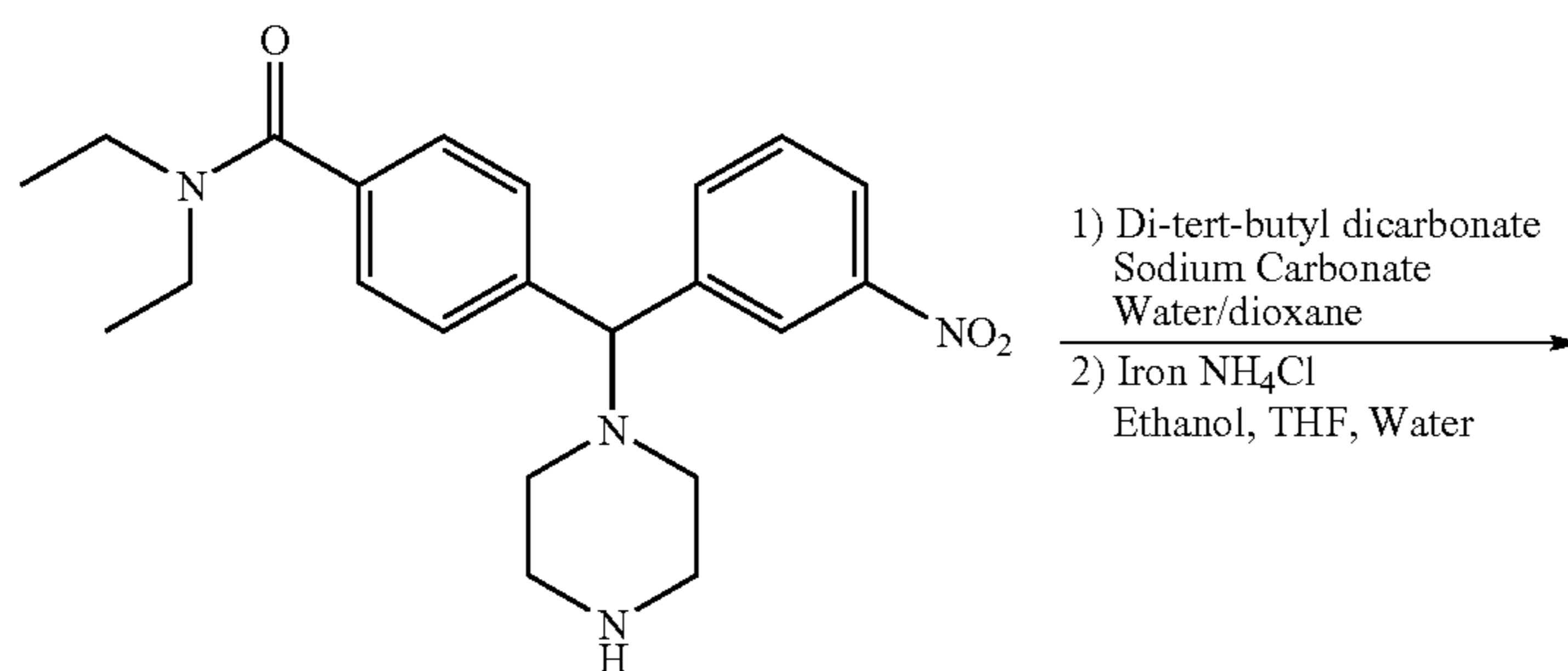
Scheme 7
