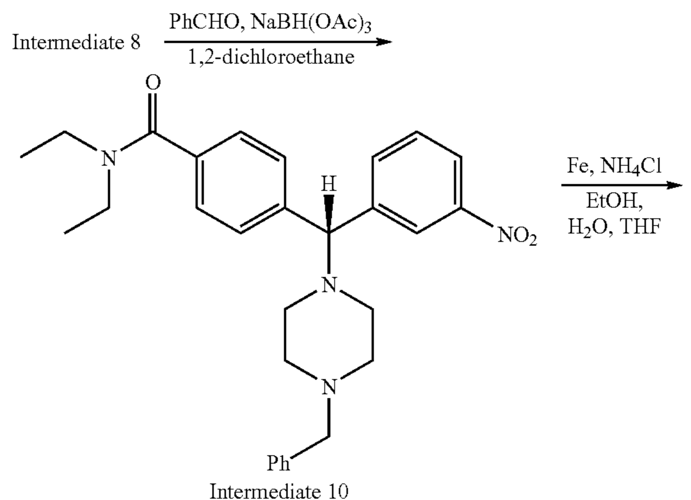
Scheme 5
