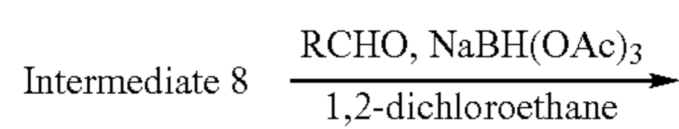
Scheme 6
