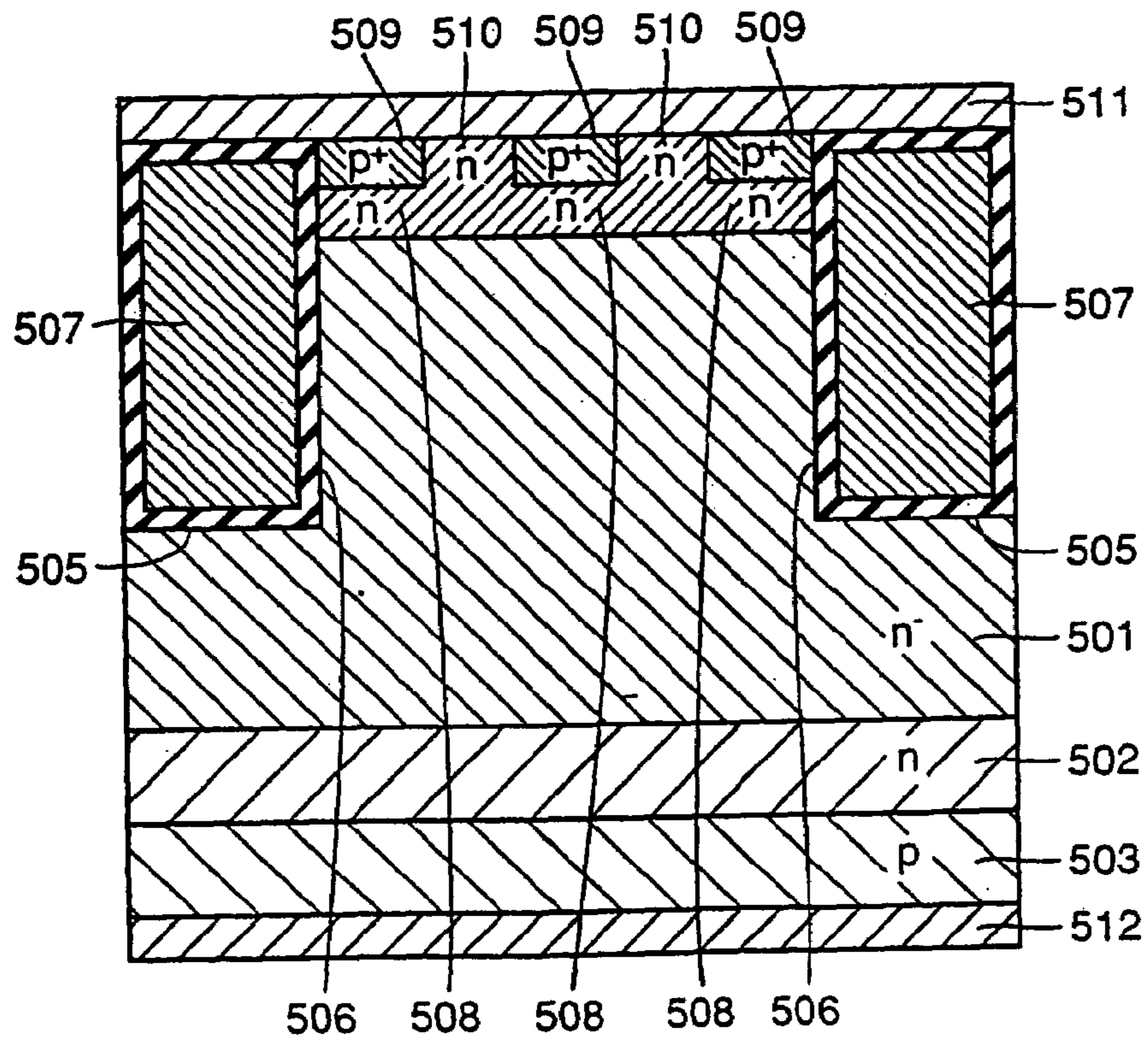
FIG. 102 PRIOR ART
