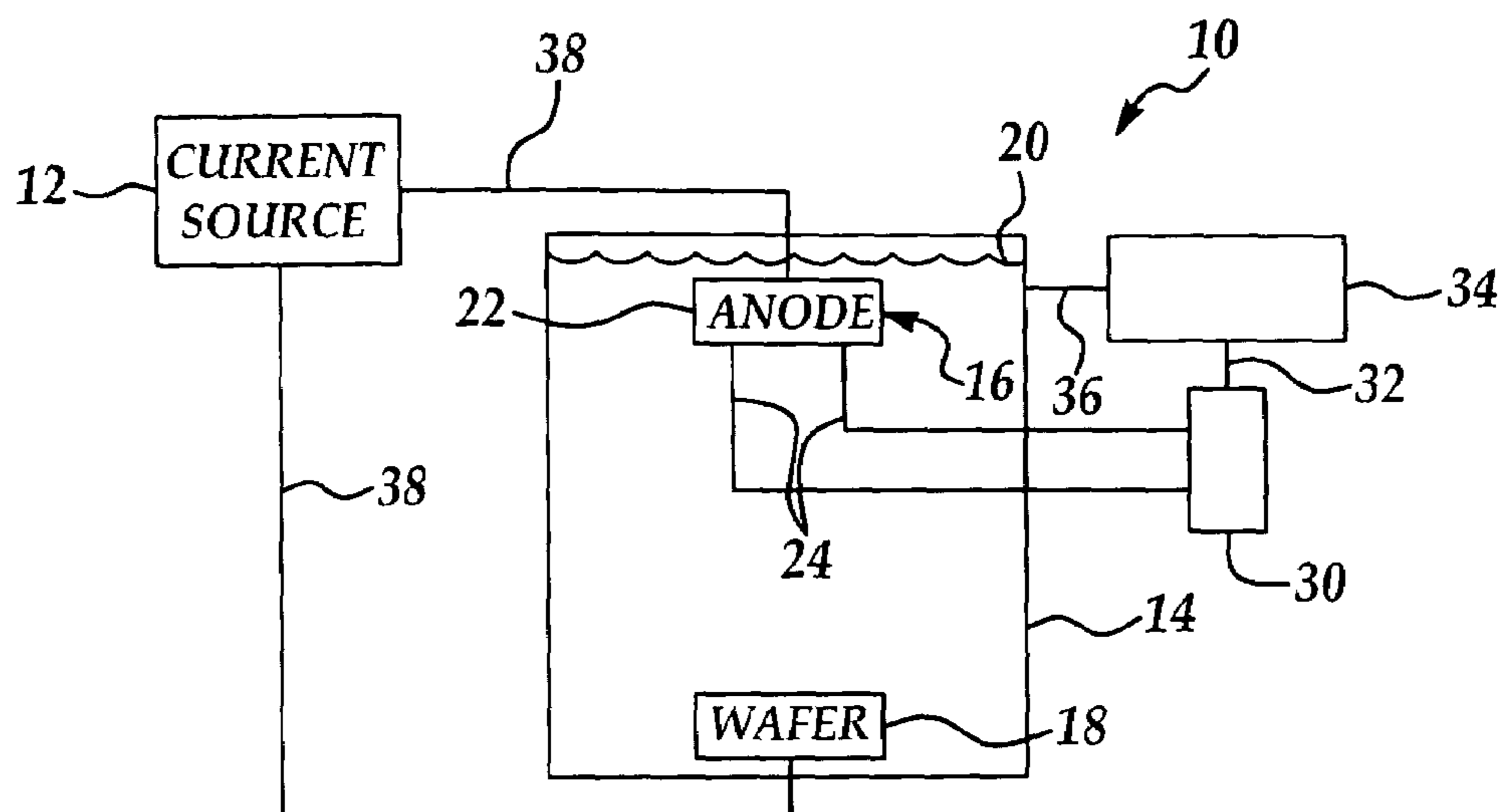
Figure 1 Prior Art
