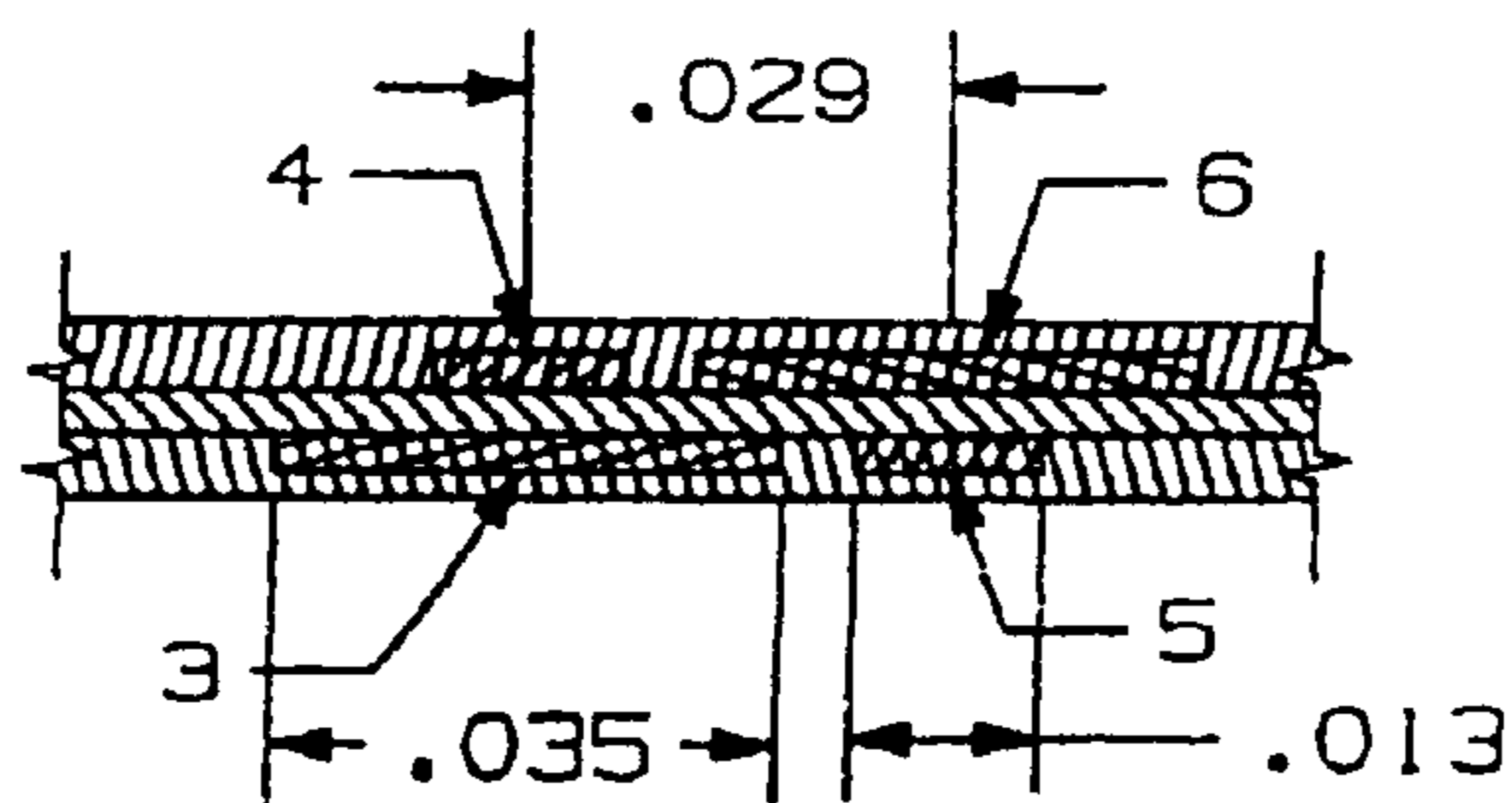
SECTION F-F
