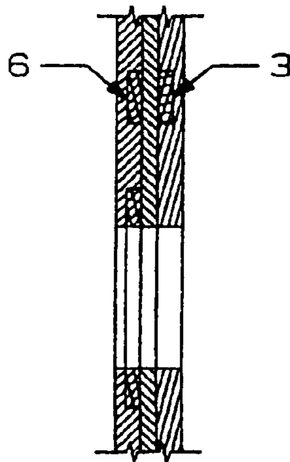
SECTION H-H
