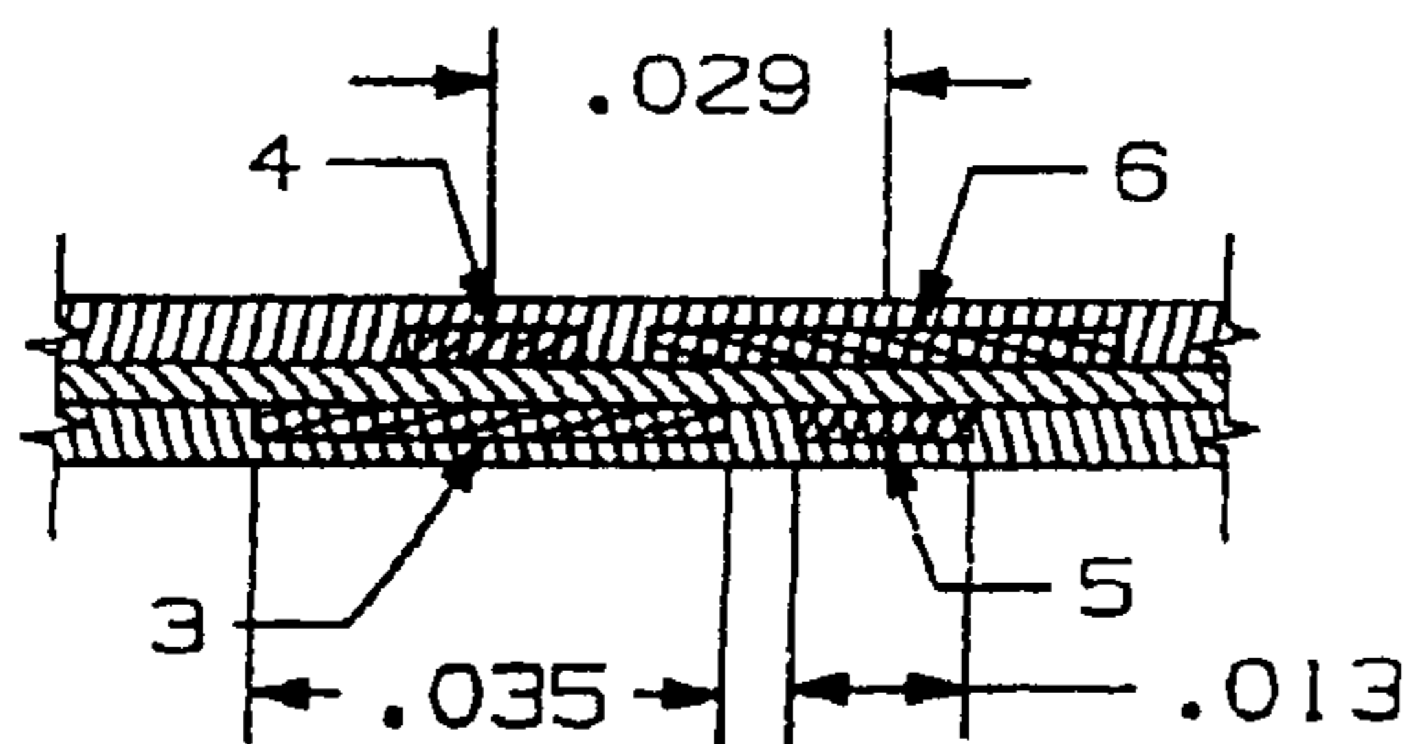
SECTION F-F
