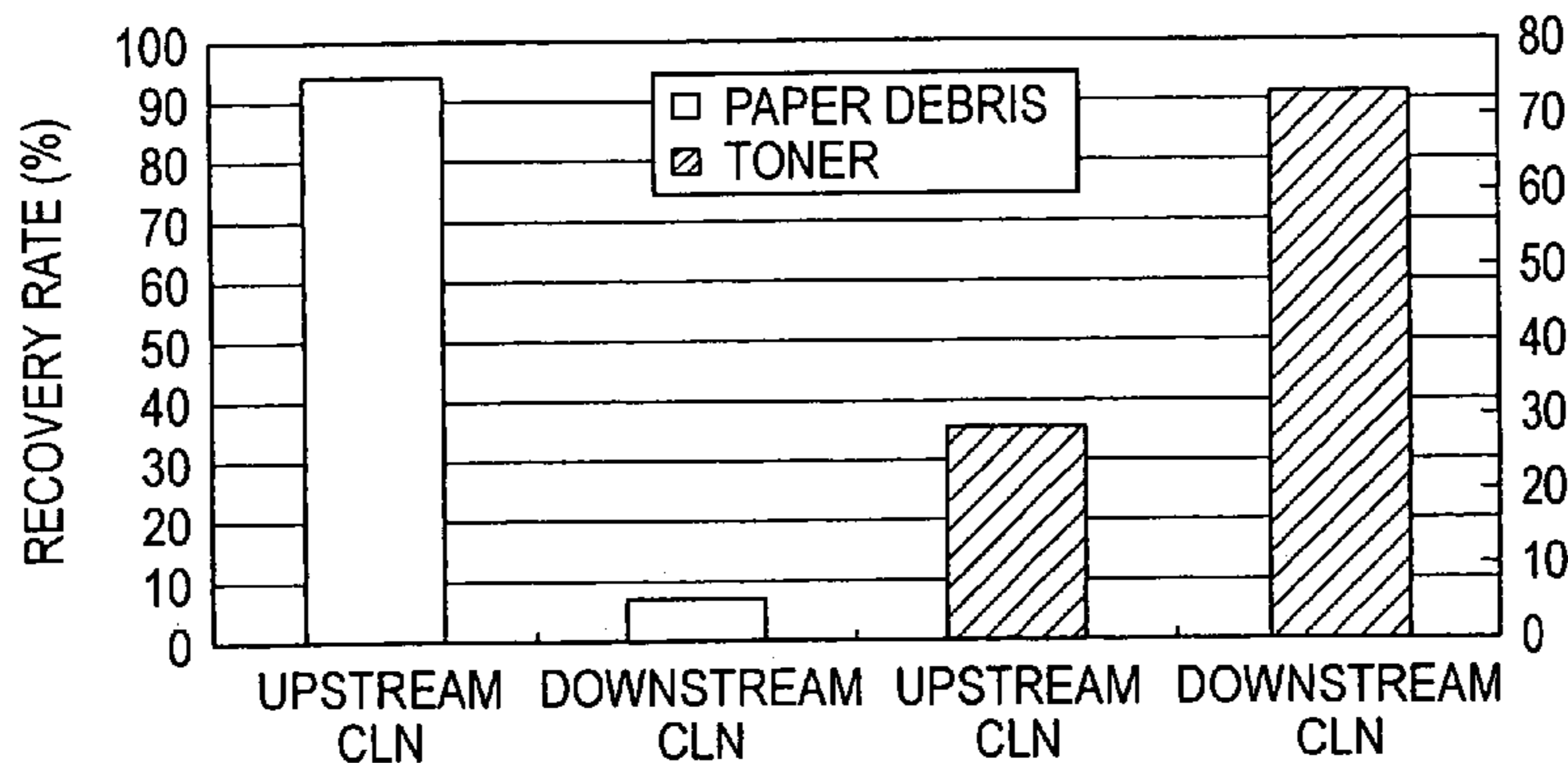
RECOVERY RATE OF PAPER DEBRIS AND TONER IN EACH CLEANING UNIT
