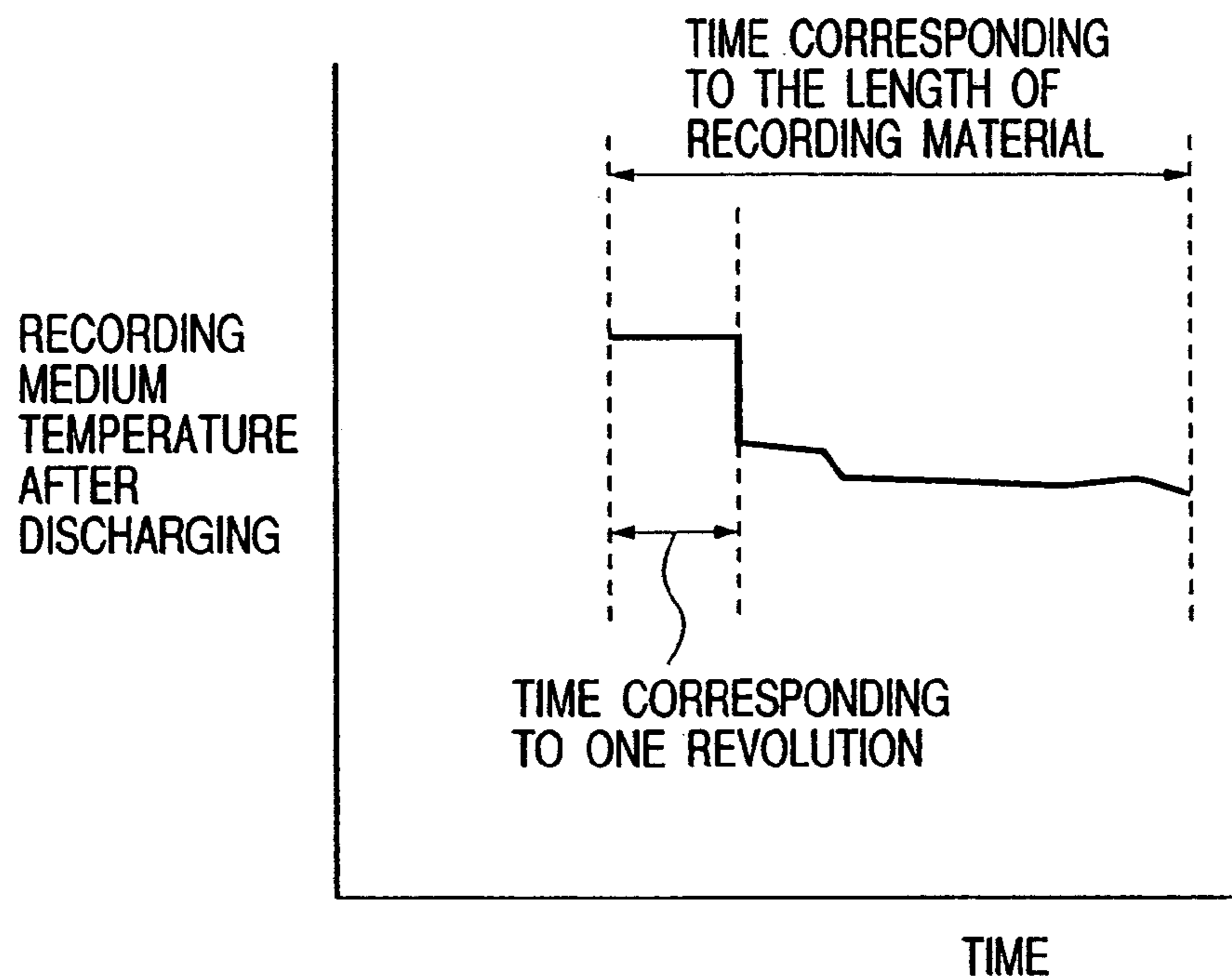
FIG. 5 PRIOR ART
