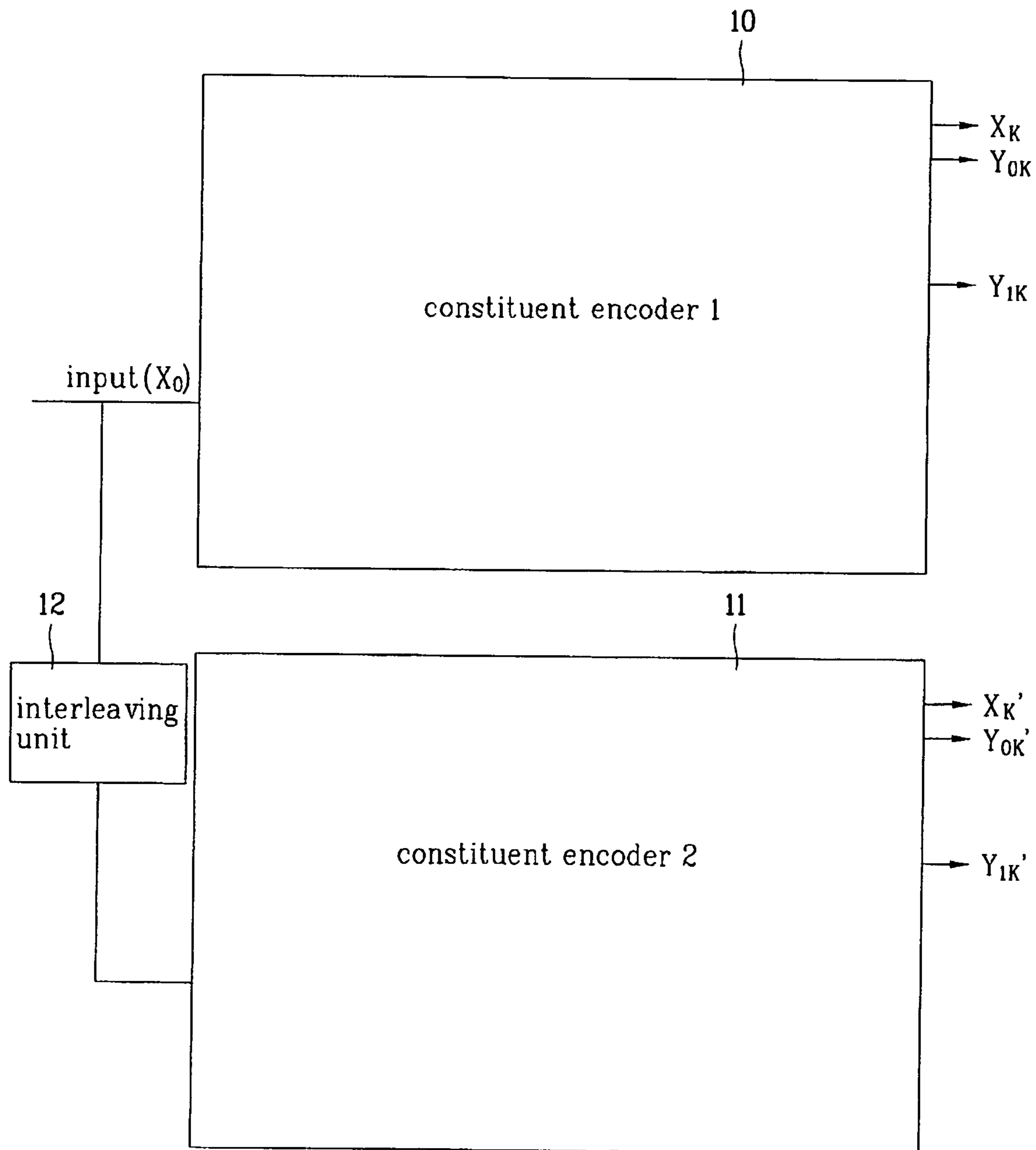
FIG. 1 Related Art
