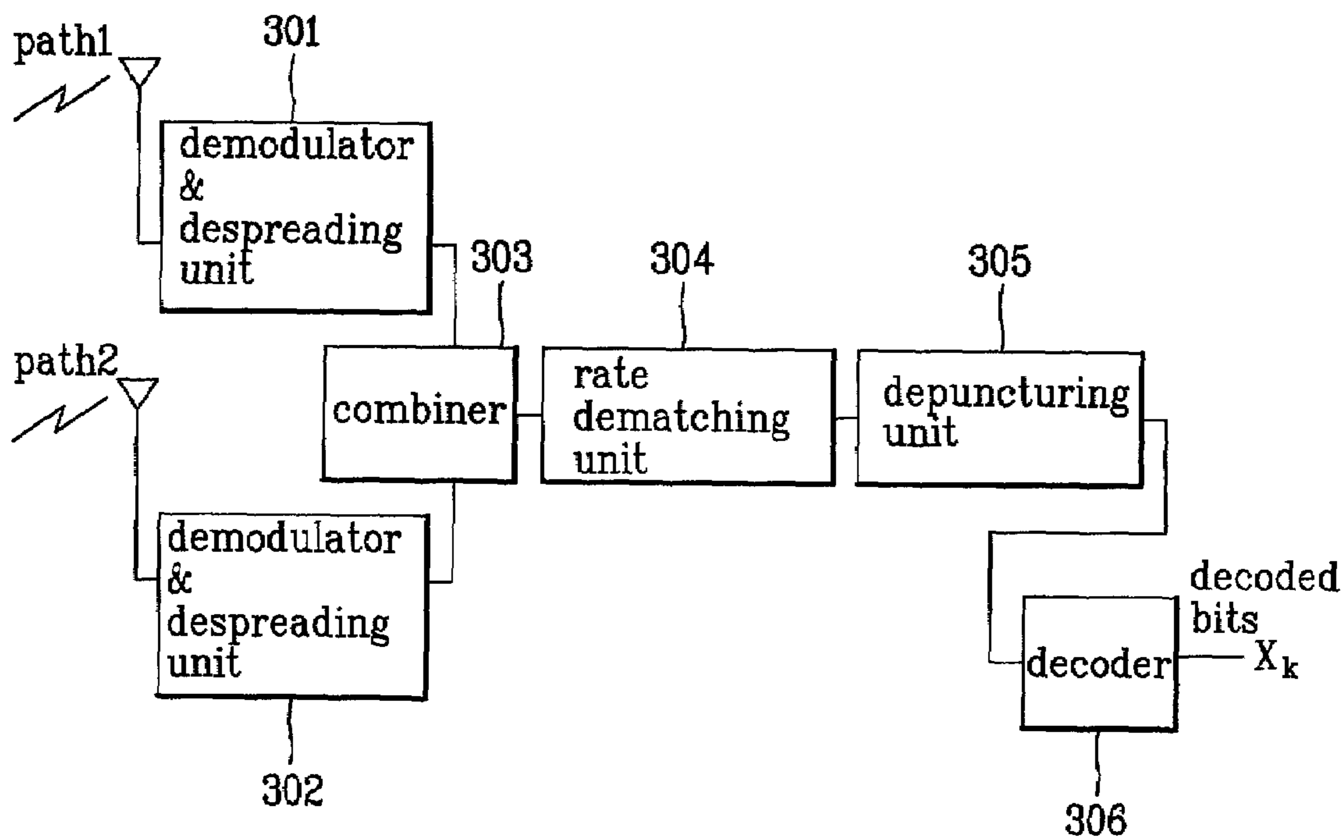
FIG. 3 Related Art
