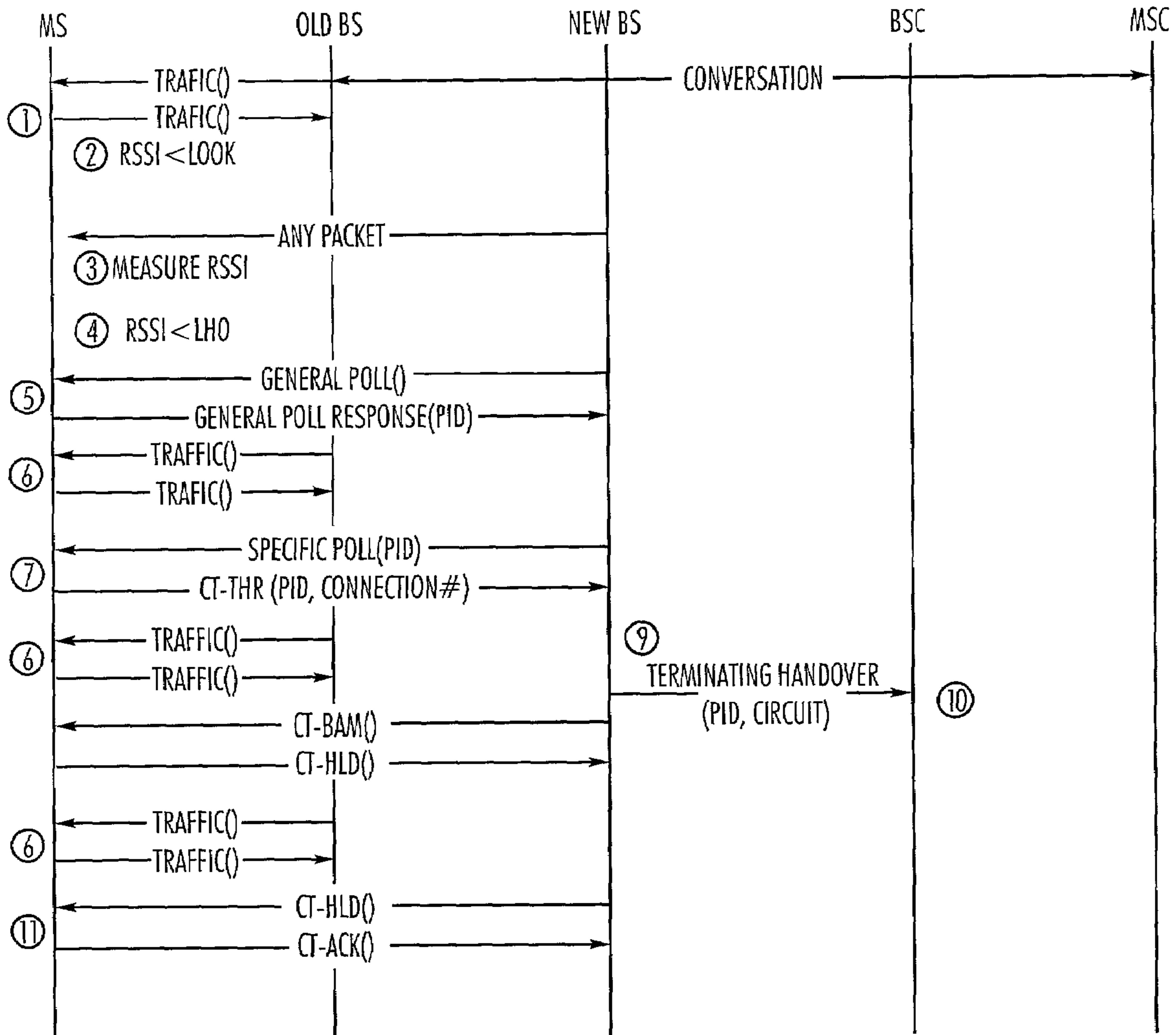
Fig. 11A INTRA BSC HANDOVER
